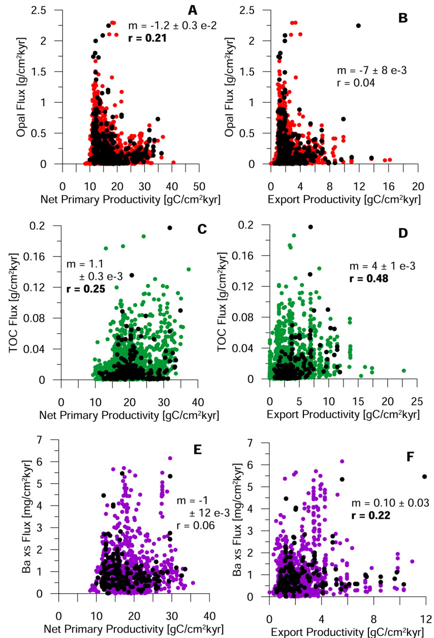
Figure 11. (a–f, respectively) Comparisons and linear correlation analyses between deep-sea opal flux, total organic carbon (TOC) flux, and Ba xs flux derived from the present study with net primary productivity (a, c, e) and export productivity estimates (b, d, f) (DeVries & Weber, 2017; Silsbe et al., 2016). Colored points are based on spatially-interpolated fluxes and black points are direct component and Th-normalized flux observations for the same core. The insets display the linear regression slope ( m , with e indicating power of 10 exponent) and Pearson correlation coefficient ( r , bold indicating statistical significance at 95% confidence).
