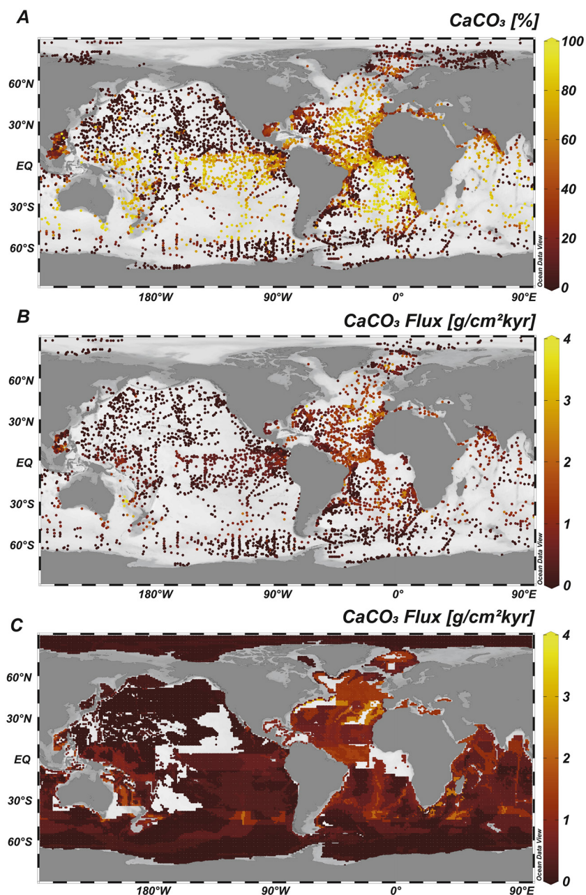
Figure 2. (a) Weight percentage of CaCO 3 , (b) flux of CaCO 3 in surface sediments using spatially-interpolated Th-normalized fluxes with discrete CaCO 3 % observations, and (c) flux of CaCO 3 using spatially-interpolated Th-normalized fluxes and spatially-interpolated CaCO 3 % values. Uncolored (white/gray) zones are shallower than 1 km or zones that do not contain any Th-normalized flux observations.
