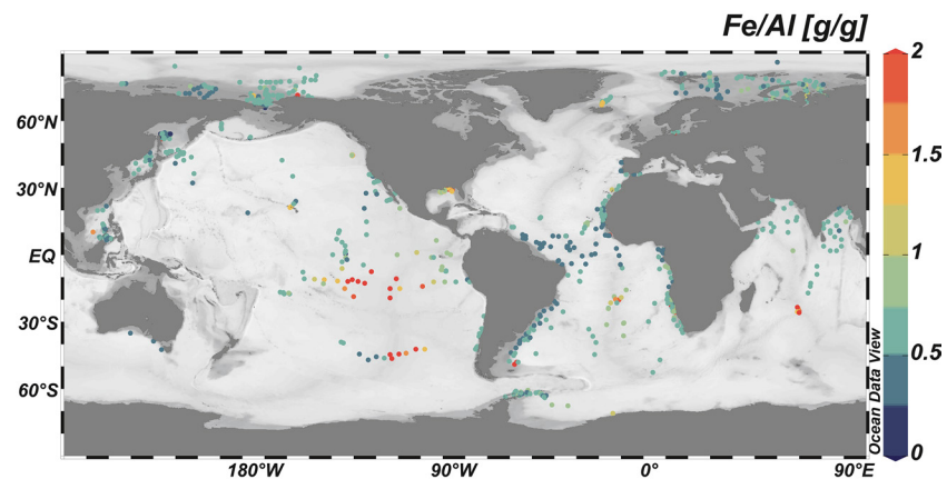
Figure 6. Fe/Al weight ratio in the global sediment composition database. The upper continental crust has an average ratio of 0.48 g/g and mid-ocean ridge basalts have a ratio of 1.01 g/g. Note in comparison to Figure 5, only a subset of Fe datapoints had available Al data.
