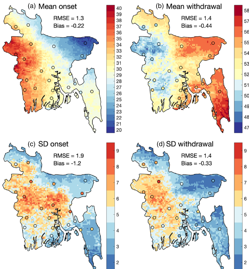
FIGURE 1 Climatology (1981–2017) of (a) monsoon onset and (b) withdrawal in Bangladesh, and (c),(d) their corresponding interannual local standard deviation (SD) for CHIRPS and station data (dots). All values are expressed in pentads. The corresponding RMSE and bias and between CHIRPS data and stations are displayed
