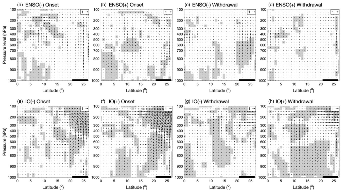
FIGURE 5 Composite anomalies of meridional circulation (vertical velocity is multiplied by 100) averaged between 85° and 95°E longitude during (a), (b) monsoon onset and (c), (d) withdrawal for the positive (+) and negative (−) phase of ENSO. Shaded areas represent the 95% confidence level of both vertical and meridional wind velocity. Black thick line at the bottom represents the location of Bangladesh
