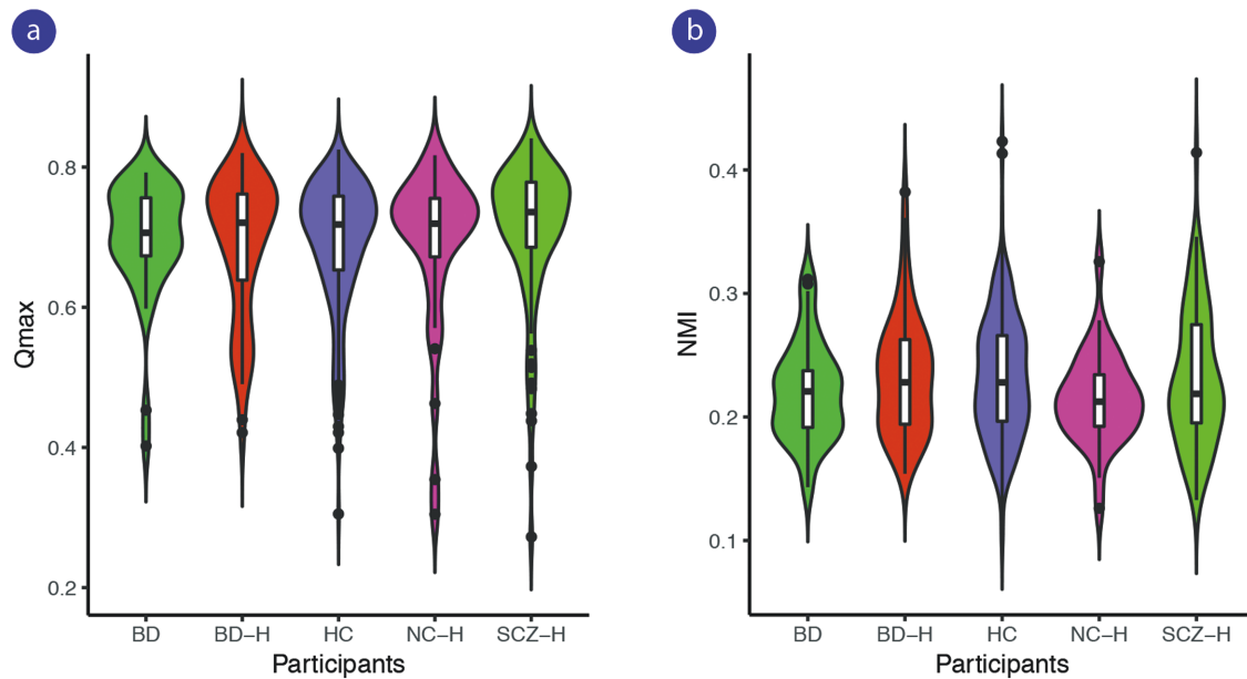
Fig. 2. Global modular organization scores per participant group. Violin plots depict the distribution of a) Q_{max} and b) NMI scores per participant group. De white boxes within the violin plots indicate the mean and standard deviations. All plots were generated before controlling for age and gender. None of the groups differed significantly at P < .05 (after regressing out age and sex, corrected for multiple comparison). These plots were generated using R package ggplot. Abbreviations: BD bipolar disorder without hallucinations; BD-H bipolar disorder with hallucinations; NC-H nonclinical individuals with hallucinations; NMI normalised mutual information; SCZ-H schizophrenia spectrum disorder with hallucinations.
