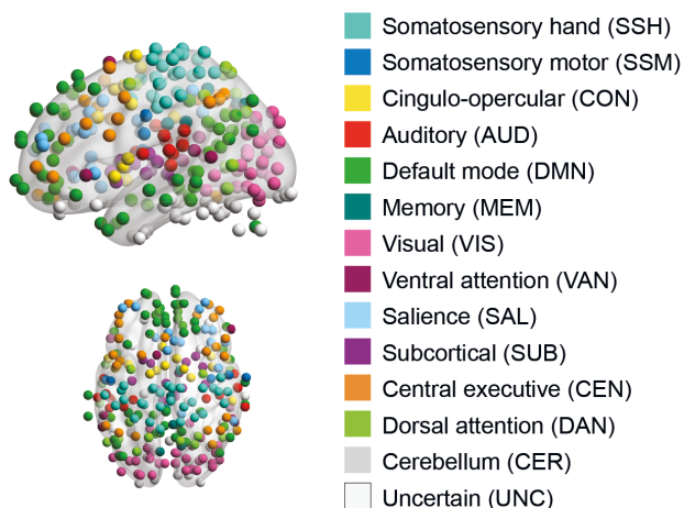
Fig. 1. A priori based modules of the Power atlas used for within- and between-module connectivity. Each node ( N = 264 ) is color-coded according to their a-prior defined module label as determined by Power et al. (2011). 15 This image was made in BrainNetViewer.
