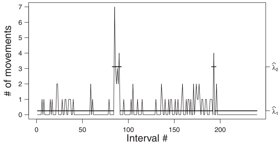
FIGURE 3 Plot of the lamb data.
