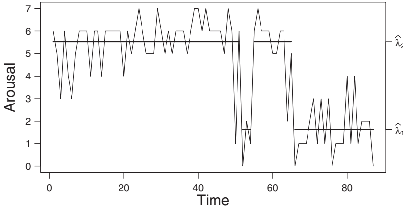
FIGURE 1 Plot of the TYT data Note: The solid horizontal lines correspond to the conditional mean of the inferred state at each time. See Table 5 for the values of \hat{\lambda}_i
