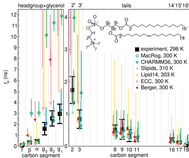
Figure 2: Evaluation of conformational dynamics of lipid from the preliminary NMRlipids Databank 103 against the effective correlation time of C–H bond rotation, \tau_e , determined using spin-relaxation data. 104 Figure adapted with permission from Ref. 103. Copyright 2021 American Chemical Society.
