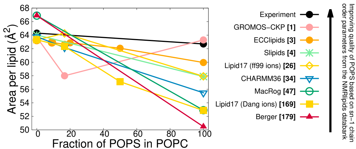
Figure 3: Area per lipid calculated from all simulations of POPC:POPS mixtures with sodium counterions at 298 K currently available in the NMRlipids Databank (left) ordered according to the quality of the POPS sn -1 acyl chain (right). The number in parenthesis describes the negative 10-base logarithm of the average probability of the acyl chain \text{CH}_2 -group order parameters to reside within experimental error in a simulation, thereby decreasing with increasing simulation quality. For reference, the values extracted from the experimental X-ray scattering data using the scattering density profile (SDP) model are shown in black. 105,106 The data used here have been originally reported in the NMRlipids publications. 33,38
