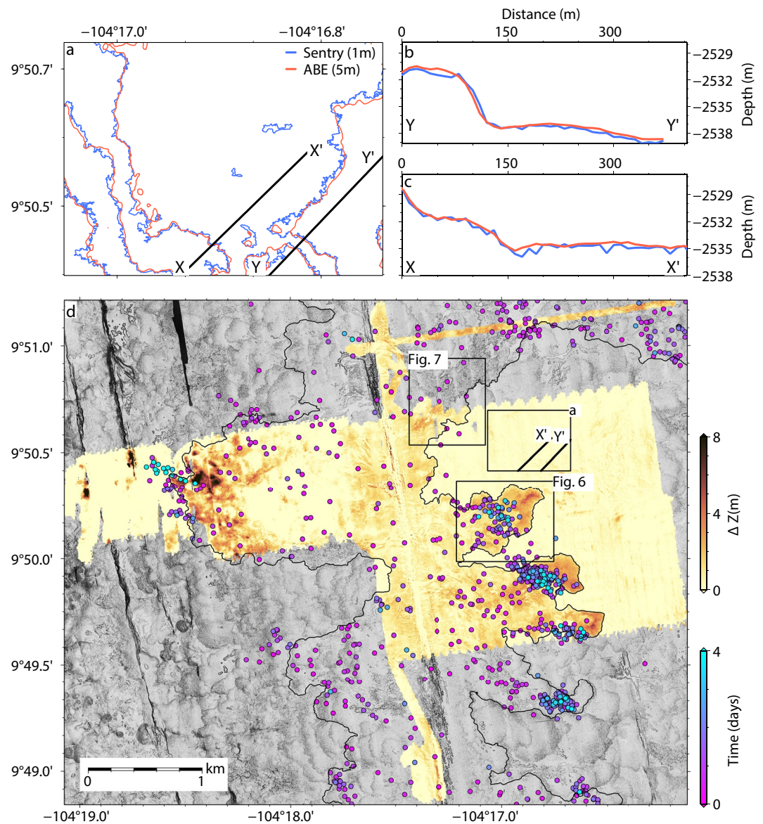
Figure 5. (a) Contours showing comparison of bathymetric data collected outside of 2005–2006 eruption extent. Red lines are pre-eruption data collected using ABE in 2001; blue lines are post-eruption data collected by Sentry in 2019. (b and c) Bathymetric profiles illustrating co-registration between shifted ABE and Sentry data. (d) Bathymetric difference map between pre- ( ABE ) and post- ( Sentry ) 2005–2006 eruptions surveys. Dots are impulsive events shaded by time after 2006-01-22 16:47 UTC (Tan et al., 2016), highlighting propagation toward the distal end of each flow away from the axial summit trough (AST). Mean flow thickness is 1.0 m, and up to ~9.0 m in the area ~2.0 km west of the AST near 9°50.4'N.
