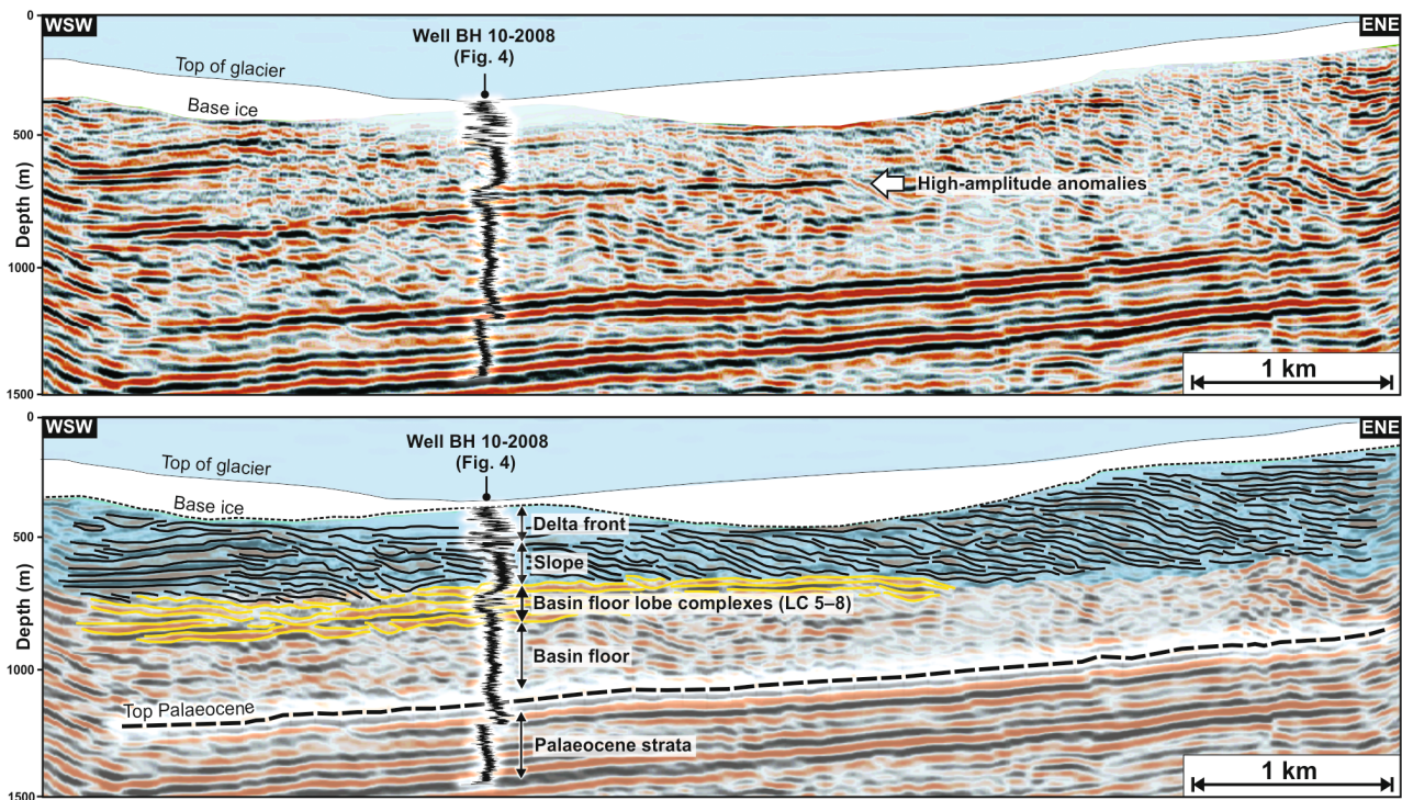
Fig. 5. Two-dimensional reflection seismic data from Sysselembreen. The line crosses Well BH 10-2008. See Fig. 1C for location. (A) Uninterpreted seismic line tied to the gamma-ray log of Well BH 10-2008. Note the presence of high-amplitude reflection anomalies exhibiting an offset stacking pattern towards the ENE (i.e. basinward), and how these anomalies correlate to an interval of serrated and blocky gamma ray signatures in the well (details shown in Fig. 4B). (B) Interpreted seismic line, showing a basinward-prograding slope succession, which partly connects with and overlies the progradationally-stacked series of lobe complexes. The interpretation is modified from Grundvåg et al. (2014a), based on Johannessen et al. (2011). The seismic data is from Johansen et al. (2011).
