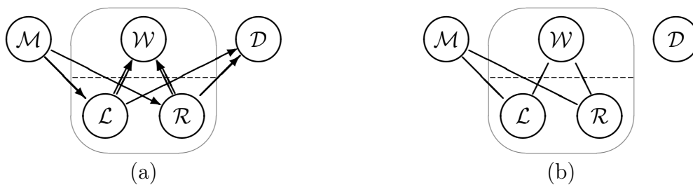
Figure 3: Voting with a non-reversible aggregation function. (a) is the true graph over \mathbf{O} = \{\mathcal{M}, \mathcal{L}, \mathcal{R}, \mathcal{W}, \mathcal{D}\} under epiphenomenalism* (where double arrows are constitutive). Graph (b) results from applying PC to the true conditional (in)dependencies over \mathbf{O} .
