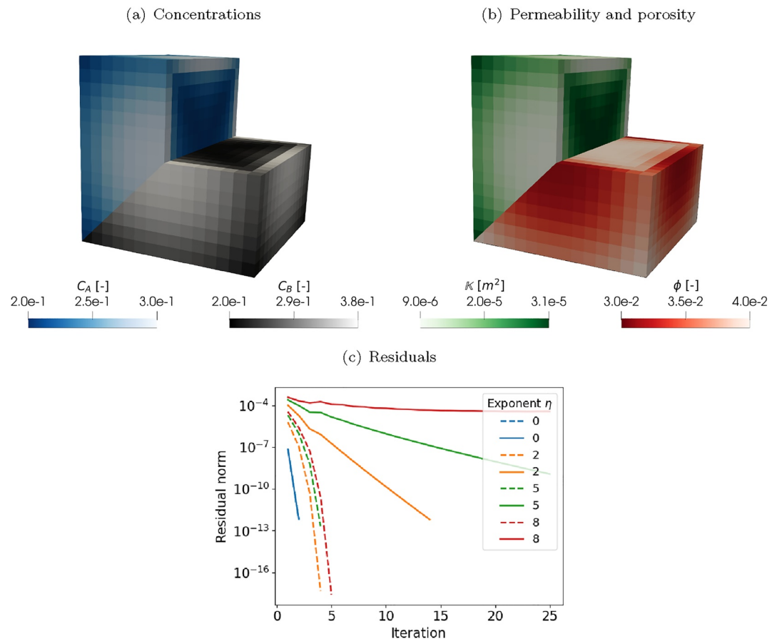
Figure 3. (top) Solution plots for \eta = 5 and (bottom) convergence rates for the reactive transport simulation. We show solute concentration ( C_A ) and precipitate volume fraction ( C_B ) to the left and permeability ( \kappa ) and porosity changes ( \phi ) to the right. The simulation domain has been sliced to expose the solution in the interior and different quantities are shown for each half of the slice using separate color maps.
