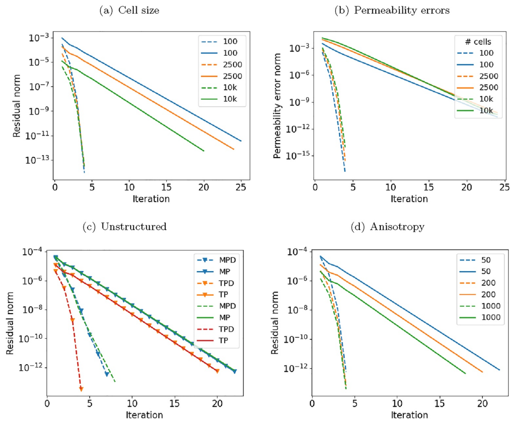
Figure 1. (top left) Convergence rates for different cell sizes, (bottom left) different mesh types, and (bottom right) discretization schemes and varying degree of mesh anisotropy. For the mesh refinement study, the permeability error is also shown (top right). We use solid lines for TP and MP and dashed lines for TPD and MPD. The bottom left plot contains results for tetrahedral and perturbed Cartesian meshes, the former of which are identified with triangular markers.
