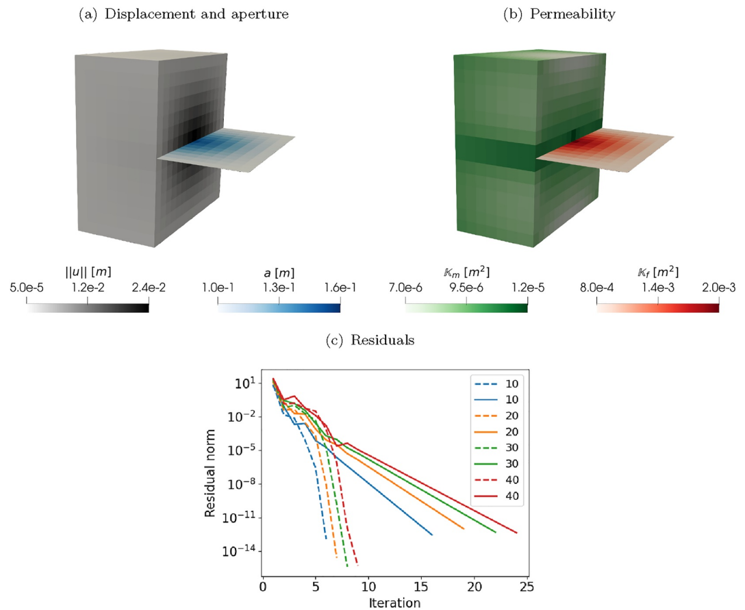
Figure 5. (top) Solution plots for the second highest source rate and (bottom) convergence rates for the deforming fracture simulation. We show matrix displacement magnitude ( \|u\| ) and fracture aperture ( a ) to the left and permeability in matrix ( K_m ) and fracture ( K_f ) to the right. Convergence plot labels correspond to the four source rates in \text{kg s}^{-1} .
