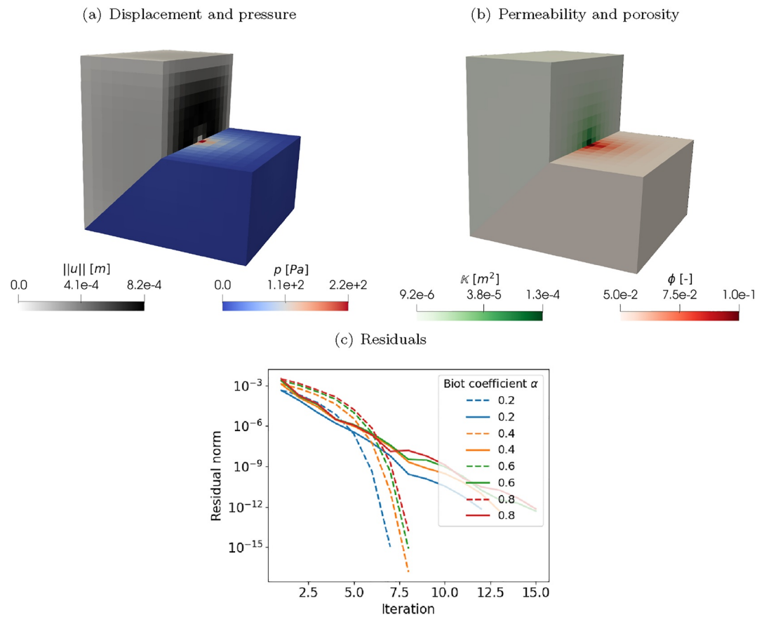
Figure 4. (top) Solution plots for \alpha = 0.6 and (bottom) convergence rates for the poroelasticity simulation. We show displacement magnitude ( \|u\| ) and pressure ( p ) to the left and permeability ( K ) on a logarithmic scale and porosity ( \phi ) to the right.
