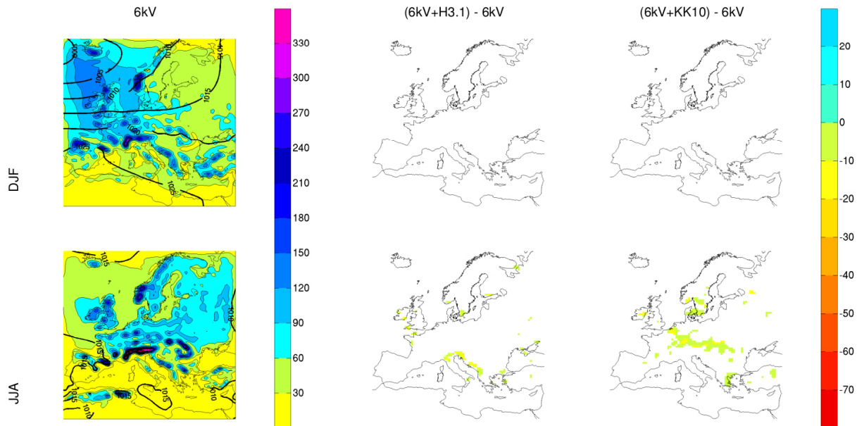
Fig. 7. Precipitation ( \text{mm month}^{-1} ) at 6 k BP for winter (top row) and summer (bottom row). Absolute precipitation and pressure from run 6 kV (left), difference 6kV + H3.1–6 kV (middle) and difference 6kV + KK10–6 kV (right). In the left panels isolines indicate pressure (hPa). In the middle and right panels grid boxes with a significant precipitation difference at the 95 % level are coloured. Isolines show differences in the remaining regions. The “zero isoline” is excluded.
