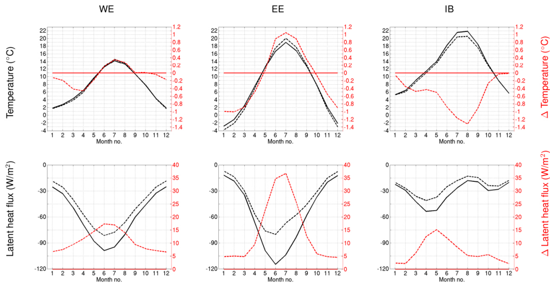
Fig. 11. Annual cycles of temperature ( ^{\circ}\text{C} , top row) and latent heat flux ( \text{W m}^{-2} , bottom row) for locations in western Europe (WE), eastern Europe (EE) and Iberian Peninsula (IB). Black lines show absolute values and red lines show anomalies relative to 0.2kV. Full black line: 0.2kV; dashed black line: 0.2kV + KK10; full red line: 0.2kV–0.2kV (i.e. zero difference); dashed red line: 0.2kV + KK10–0.2kV. Definitions of WE, EE and IB are found in Fig. 1.
