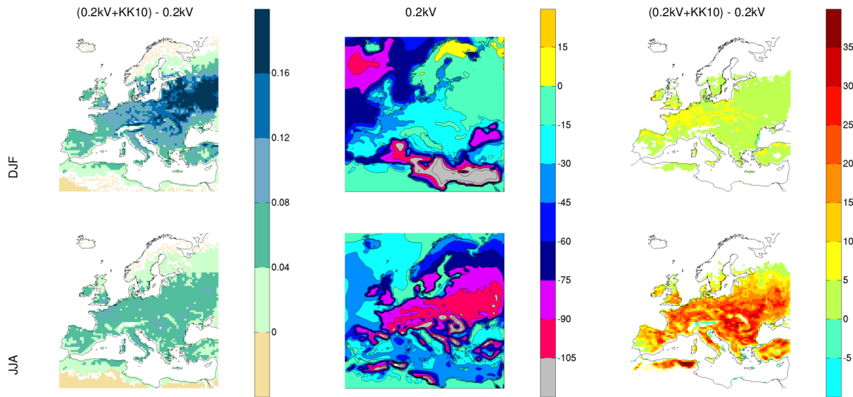
Fig. 10. Albedo difference, 0.2kV + KK10–0.2kV (left), absolute latent heat flux ( \text{W m}^{-2} ) from run 0.2kV (middle), and difference in latent heat flux 0.2kV + KK10–0.2kV (right) for winter (top) and summer (bottom). In the left and right panels, grid boxes with a significant difference at the 95 % level are coloured. Isolines show differences in the remaining regions. The “zero isoline” is excluded.
