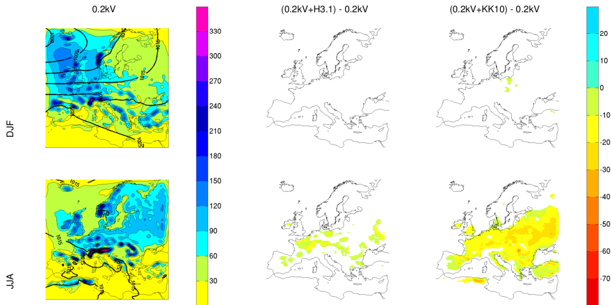
Fig. 8. Precipitation ( \text{mm month}^{-1} ) at 0.2 kBP for winter (top row) and summer (bottom row). Absolute precipitation and pressure from run 0.2 kV (left), difference 0.2kV + H3.1–0.2kV (middle) and difference 0.2kV + KK10–0.2kV (right). In the left panels isolines indicate pressure (hPa). In the middle and right panels grid boxes with a significant precipitation difference at the 95 % level are coloured. Isolines show differences in the remaining regions. The “zero isoline” is excluded.
