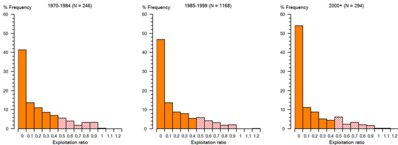
Figure 10. Frequency distribution of all fished functional groups ( F/Z > 0.001 ) by 15-year intervals since 1970 in relation to their fishing pressure (exploitation ratio). Relative proportion of overfished groups ( F/Z > 0.4 ) is indicated by hatched bars and has decreased slightly from 18 to 16% over the period. N is total number of exploited groups in each time period. This figure is available in black and white in print and in colour at ICES Journal of Marine Science online.
