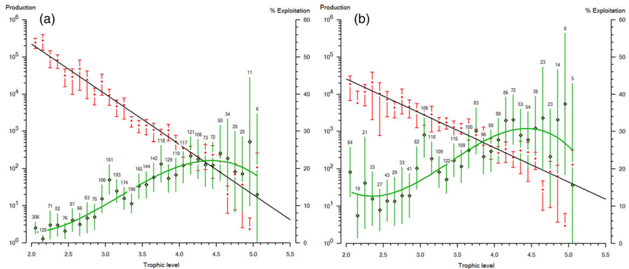
Figure 4. (a) Left axis: Total (average) production per unit area ( \text{kg km}^{-2} \text{yr}^{-1} ) against TL in 110 Ecopath models (Figure 2) across the world since 1970. All functional groups included. (b) Same as A but only with exploited functional groups ( E > 0.001 ) included. Right axes: The global fishing pattern and pressure expressed as average exploitation rate ( E = Y/P = F/Z ) against TL in 0.1 intervals. Error bars represent the 95% confidence limits and small numbers = sample size (number functional groups in each TL interval). This figure is available in black and white in print and in colour at ICES Journal of Marine Science online.
