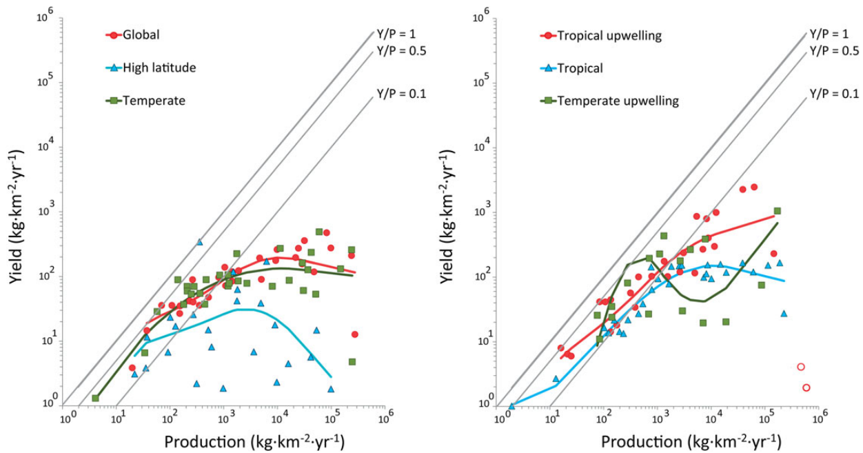
Figure 7. A summary of the fishing pattern and fishing pressure globally and across five different ecosystem types using a mixed effects model with a spline as random effect to show the general non-linear and non-balanced harvest patterns across TLs. High latitude and temperate fisheries, left panel, and temperate upwelling, right panel, are least balanced, and tropical and tropical upwelling fisheries, right panel, the most balanced. Each point is the mean of all functional groups in 0.1 TL intervals between TL 2 and TL 5. Open circles are groups of gastropods and benthic organisms and are not taken into account. All non-linear patterns are significantly different from the linear component. In the regression all data points (averages per trophic bin of 0.1) are weighted for the number observations over which the average is taken (see Supplementary material). This figure is available in black and white in print and in colour at ICES Journal of Marine Science online.
