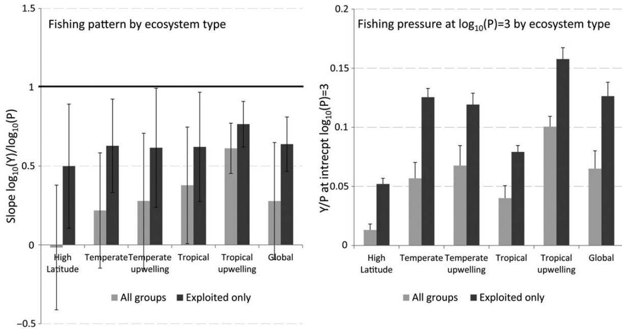
Figure 8. Left panel: Fishing pattern. Values of the slope of the regression of \log_{10}(Y) over \log_{10}(P) for the five ecosystem types. Error bars ( \pm 1.96SE ) indicate significance of the difference between the slope = 1 (balanced) and slope = 0. Black horizontal line represents slope = 1. Right panel: Fishing pressure. Exploitation rate ( Y/P ) per ecosystem type calculated from the intercept of the regression of \log_{10}(Y) over \log_{10}(P) centered on \log_{10}(P) = 3 ( =1 \text{ ton km}^{-2} \text{ yr}^{-1} ), for which groups exploitation is generally highest (Figure 4). Values are shown for models including all groups by TL bins of 0.1 and exploited groups only.
