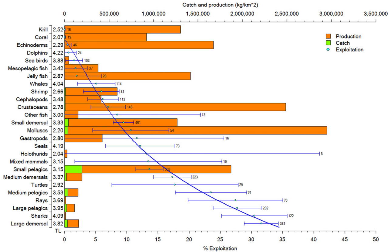
Figure 5. Total mean production (orange bars) and total mean yield (green bars) in \text{kg km}^{-2} of major functional species groups (top axis) and overall mean exploitation rates (line) with 95% confidence intervals and number of functional groups in each category (bottom axis). X-axis is ordered by exploitation rate. TL = mean trophic level. This figure is available in black and white in print and in colour at ICES Journal of Marine Science online.
