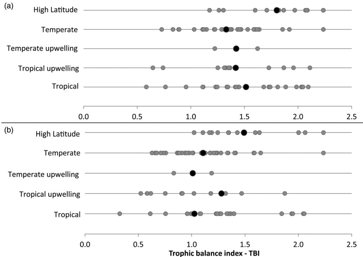
Figure 12. TBI plotted against ecosystem type for the subset of 103 models, where average values are indicated by the black filled circles. (a) All functional groups included. (b) Same as (a) but only including exploited functional groups ( E > 0.001 ).
