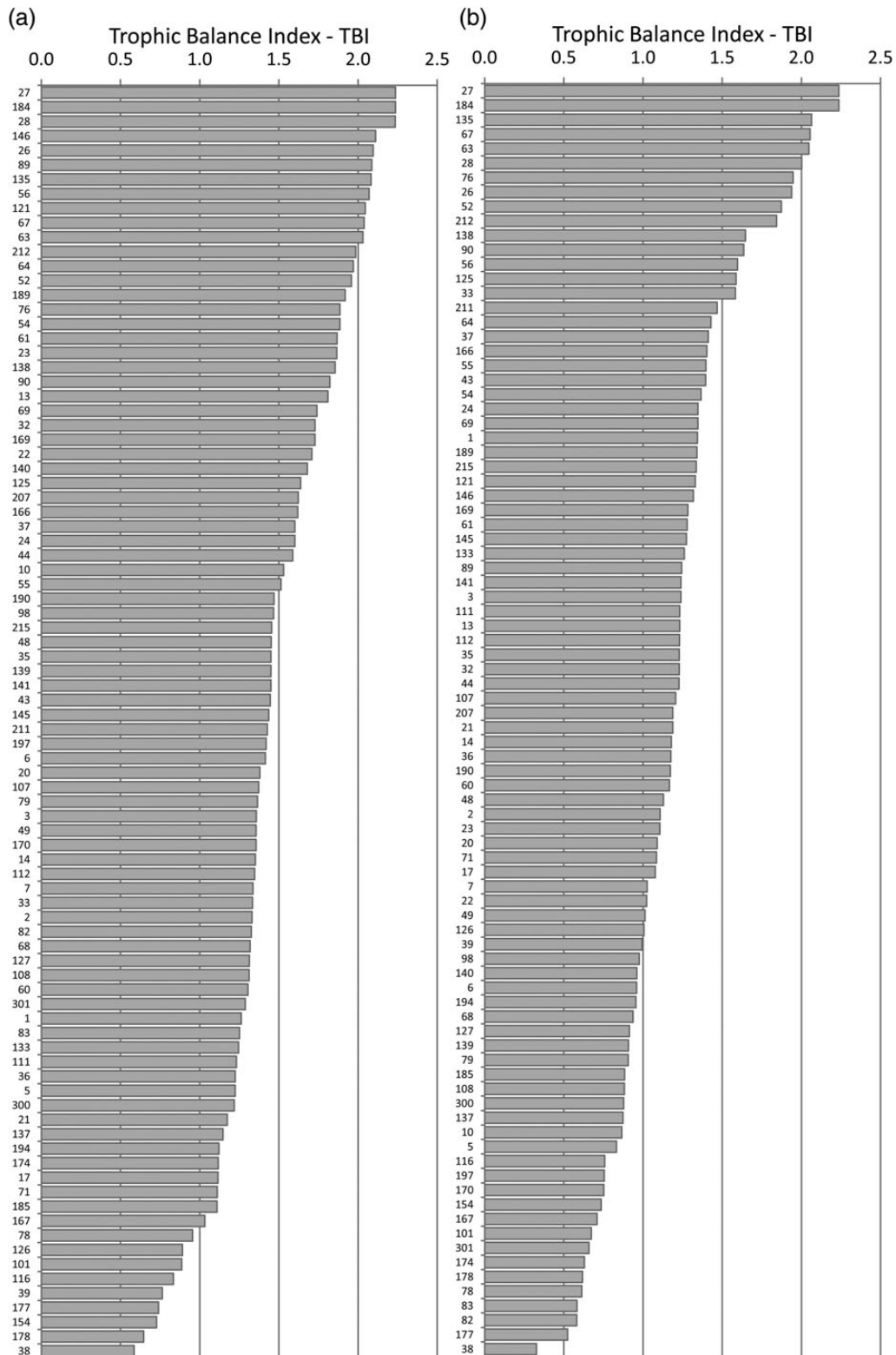
Figure 11. TBI for the subset of 103 modelled, exploited marine ecosystems when (a): all functional groups included. (b) Same as (a) but only including exploited functional groups ( E > 0.001 ). Numbers refer to Ecopath models and are provided in Supplementary material.
