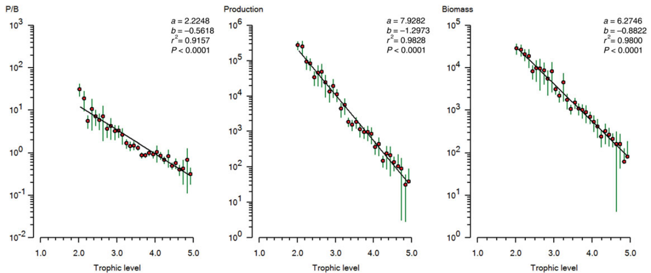
Figure 3. Overall relationships between production to biomass ratio ( P/B , \text{year}^{-1} ), production ( \text{kg km}^{-2} \text{yr}^{-1} ), and biomass ( \text{kg km}^{-2} ) with mean TL in 0.1 intervals of all functional species groups (except TL < 2 ) in 110 Ecopath models. Error bars are 95% confidence intervals. This figure is available in black and white in print and in colour at ICES Journal of Marine Science online.
