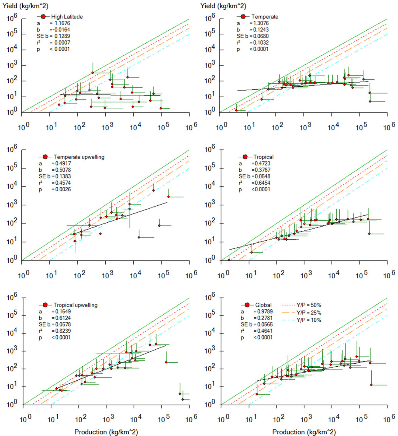
Figure 6. Average fishing pattern in five main ecosystem types across the world since 1970, and the total global average, expressed as log 10 yield (kg km -2 yr -1 ) vs. log 10 production (same units). Each point is the mean of functional groups in 0.1 TL intervals (Figure 3) between TL 2 and TL 5, green error bars are standard deviations. The more the slope deviates from the 1:1 line (green) between yield and production, the more “unbalanced” ( sensu Garcia et al., 2012 ) the fishery is. Fishing pressure or exploitation rate ( E ) is inversely correlated with orthogonal distance from the 1:1 line where yield = production. Exploitation rates equivalent to 10, 25, and 50% are given as parallel lines. p -values give the test of slopes ≠ 1. All slopes are significantly different from 1, but High latitude, Temperate, and Temperate upwelling are not significantly different from zero. Two outliers consisting of benthos and gastropods (blue circles) have been omitted from the trend in Tropical upwelling. This figure is available in black and white in print and in colour at ICES Journal of Marine Science online.
