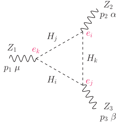
Figure 2: Feynman diagram related to \text{Im } J_2 .
