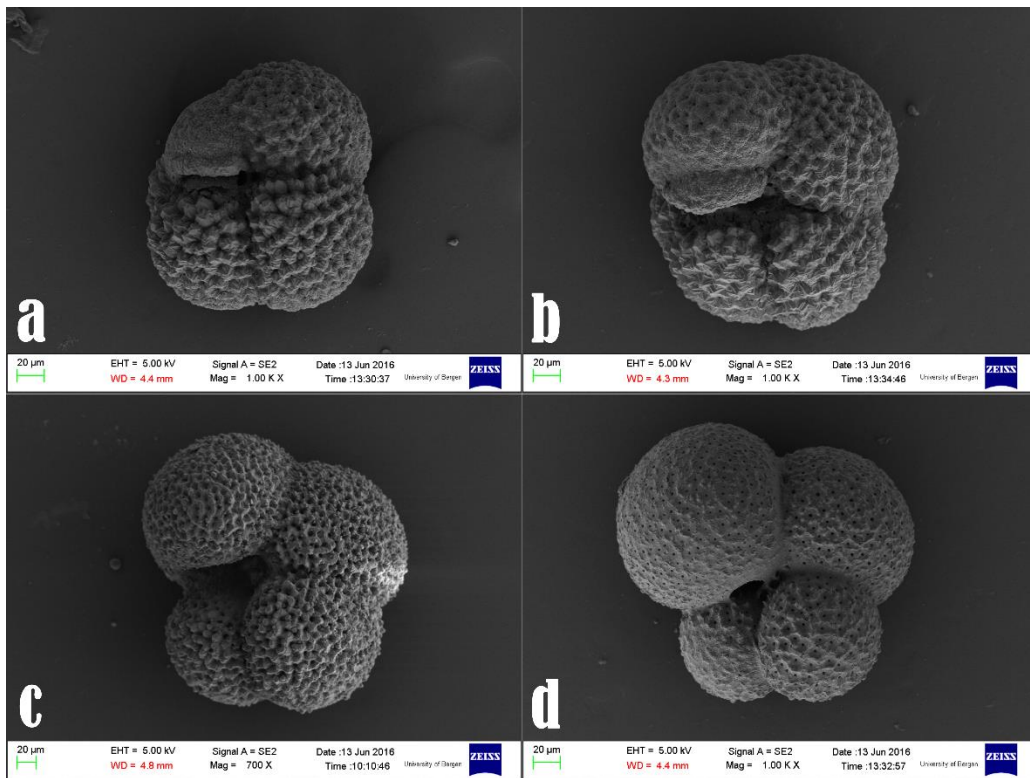
Figure 3.4 N. incompta showing different morphologies.
