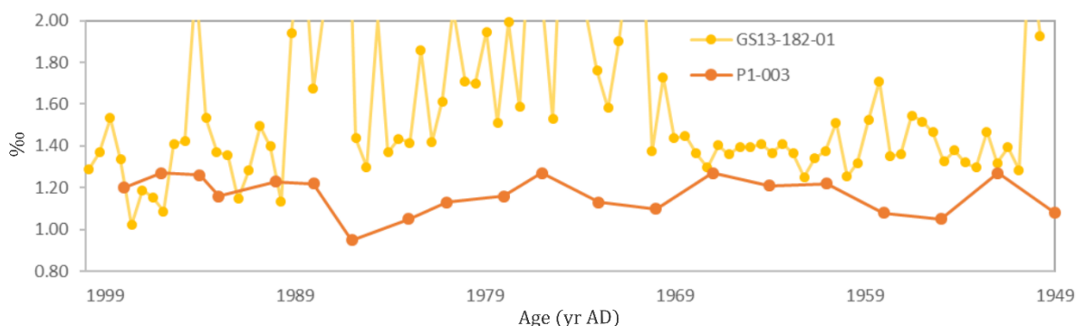
Figure 5.4 Stable oxygen isotope data from core GS13-182-01 and P1-003 (Sejrurp et al., 2010; 2011)
