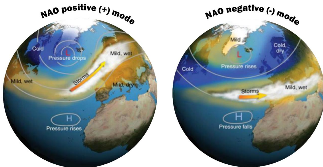
Figure 2.11 Different modes of the NAO. Positive NAO reflects a pressure drop of the Icelandic Low and storm patterns moving over Scandinavia, resulting in mild and wet conditions. Negative NAO reflects a pressure rise of the Icelandic Low and storm patterns moving over the southern part of Europe, resulting in cold and dry conditions in Scandinavia (modified from Climatesnack, 2013).
