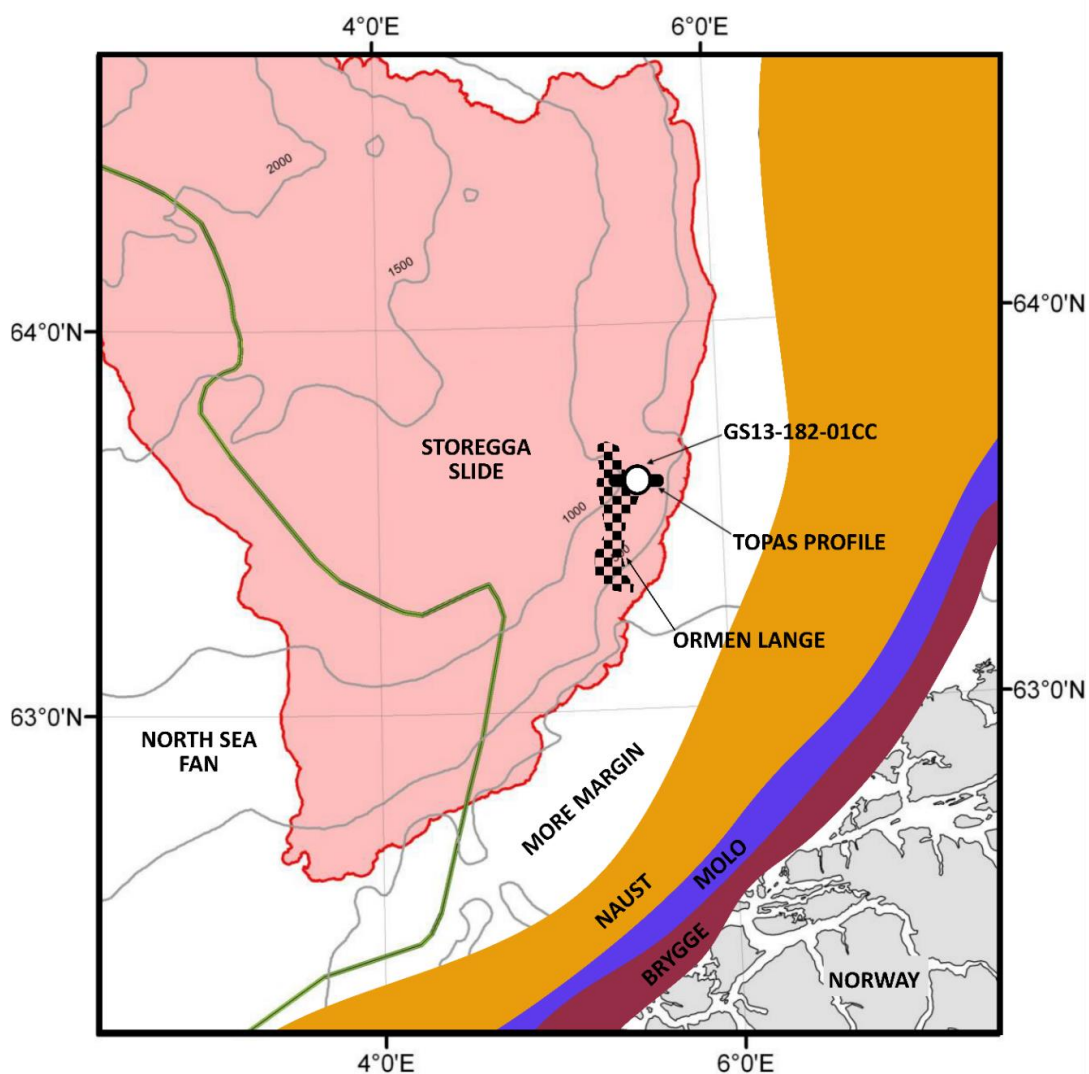
Figure 2.3 Bathymetry map of the head of the Storegga slide and adjacent formations, the North Sea fan, Naust, Molo and Brygge. Ormen lange, the GS13-182-01 coring site and TOPAS profile are also shown (modified from Hjelstuen et al., 2013 and Ottesen et al., 2009).
