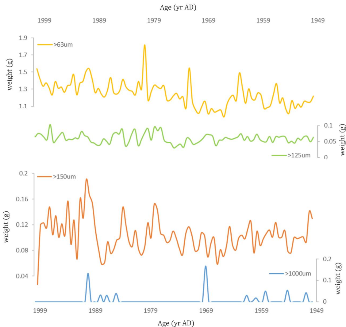
Figure 3.6 Grain size results from core GS13-182-01 (Becker et al., in prep).
