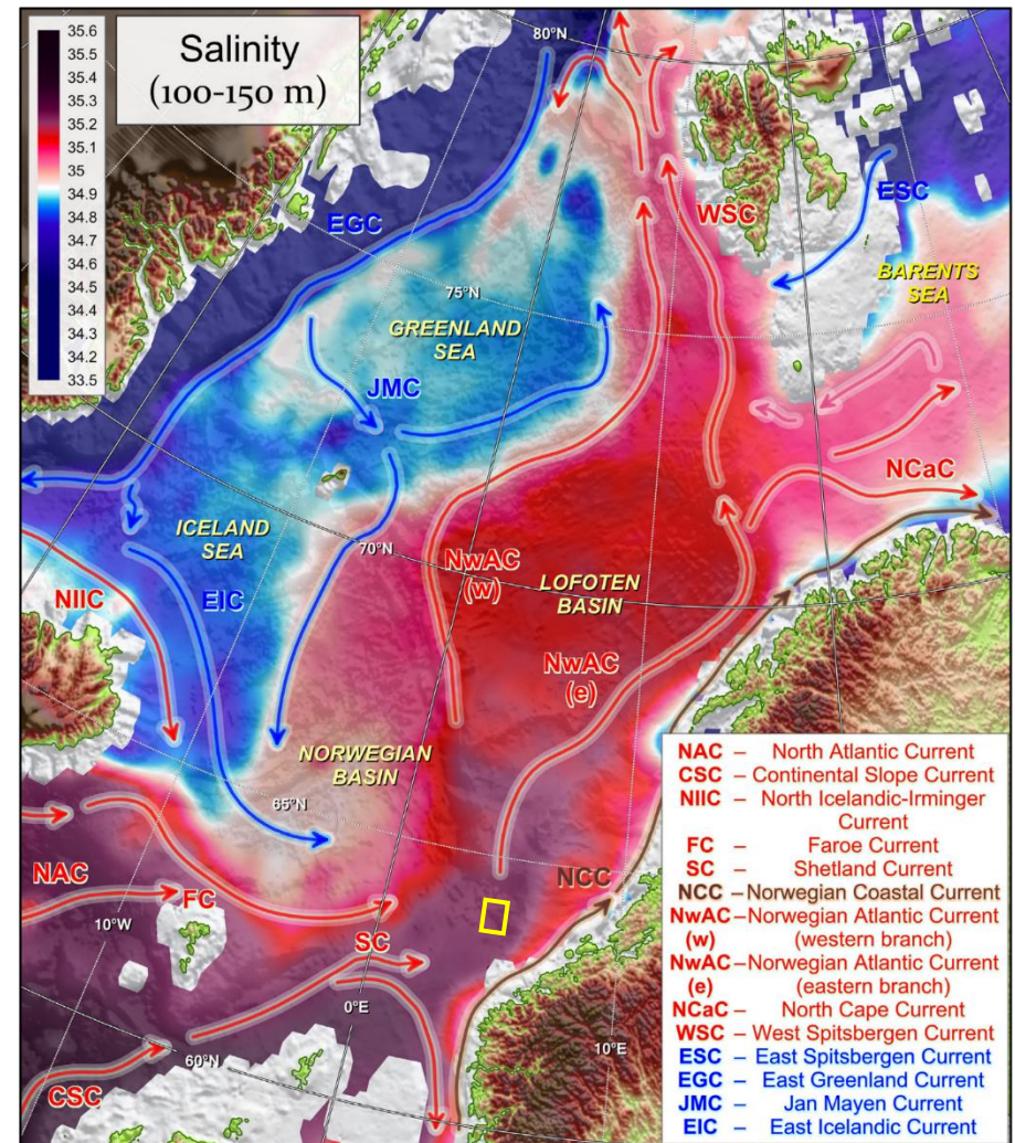
Figure 2.8 Near-surface salinity in the Nordic seas. Major currents and basins are displayed. The study area is marked with a square (Yashayaev et al., 2015).
