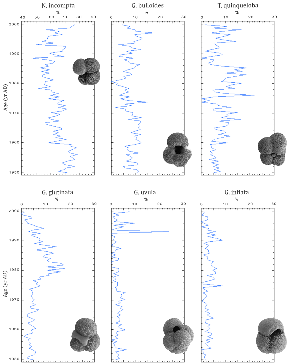
Figure 4.2 Results from the foraminifera analysis of 90 samples between 1949-200 AD from core GS13-182-01.
