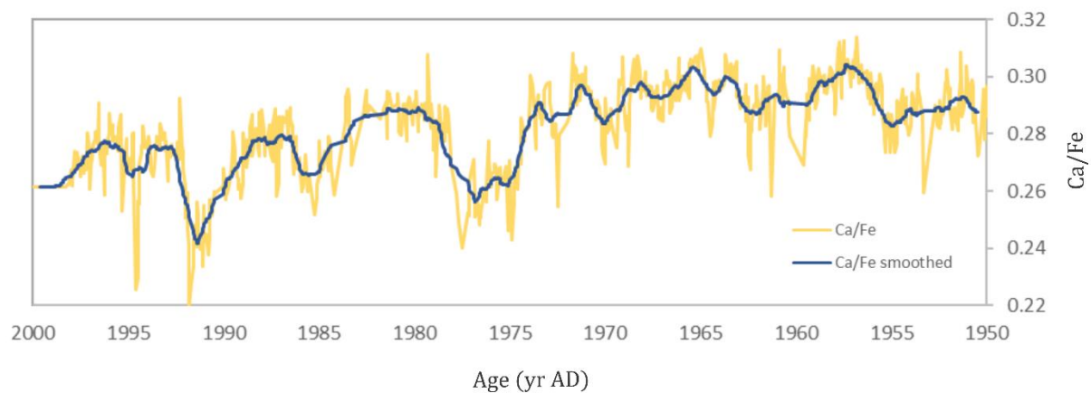
Figure 3.8 Ca/Fe results from core GS13-182-01 (Becker et al., in prep).
