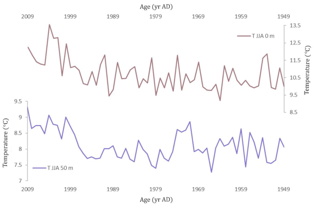
Figure 5.2 Temperature data from OWSM at 0 m and 50 m depth. Notice that the time scale is extending to 2009, capturing the current warming trend.
