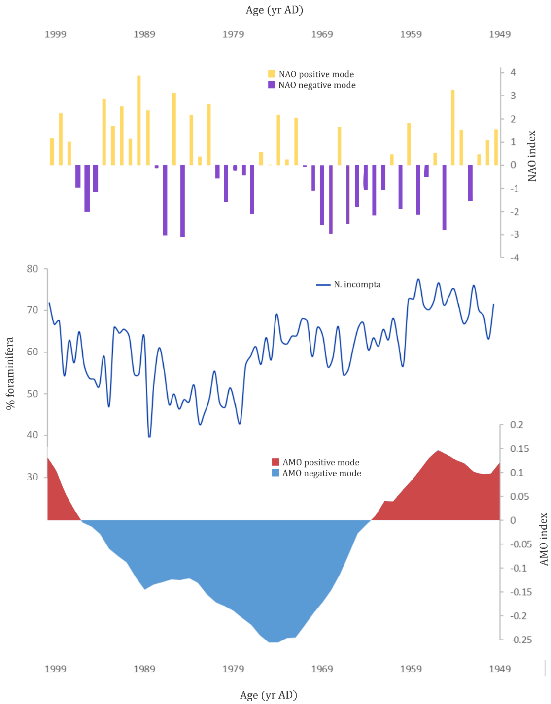
Figure 5.6 Comparison of the NAO index (Hurrell et al., 2016), AMO index (Enfield et al., 2001) and abundance of N. incompta .
