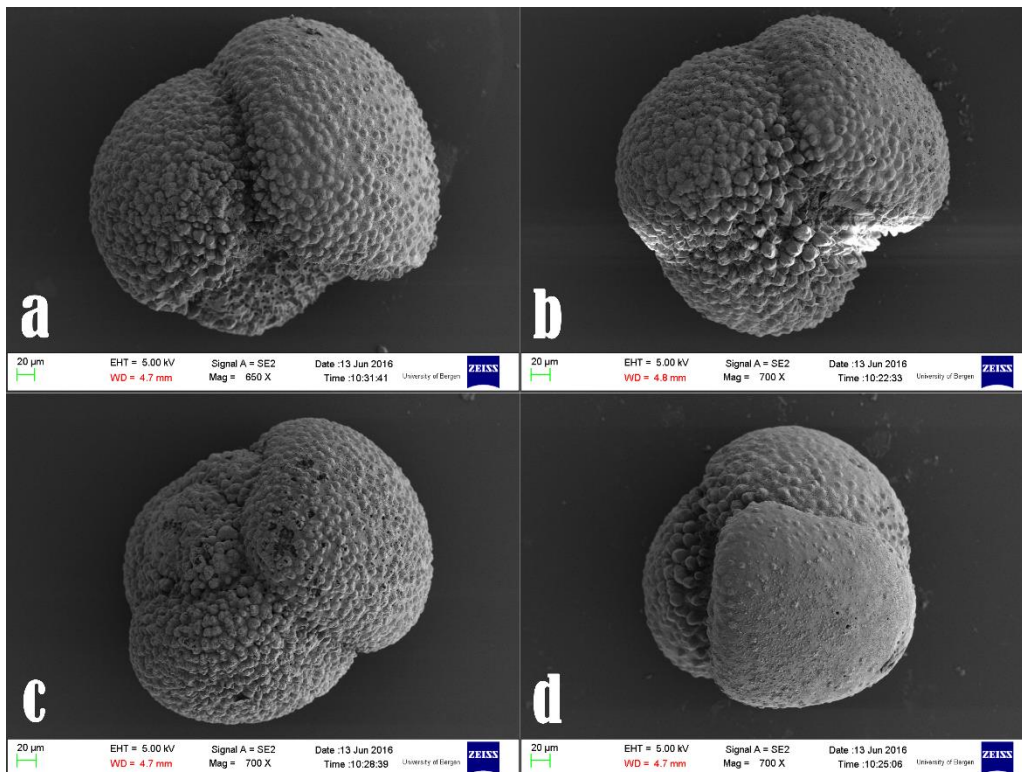
Figure 3.5 G. inflata . (a) and (b) different morphologies umbilical side (c) back view, (d) top view
