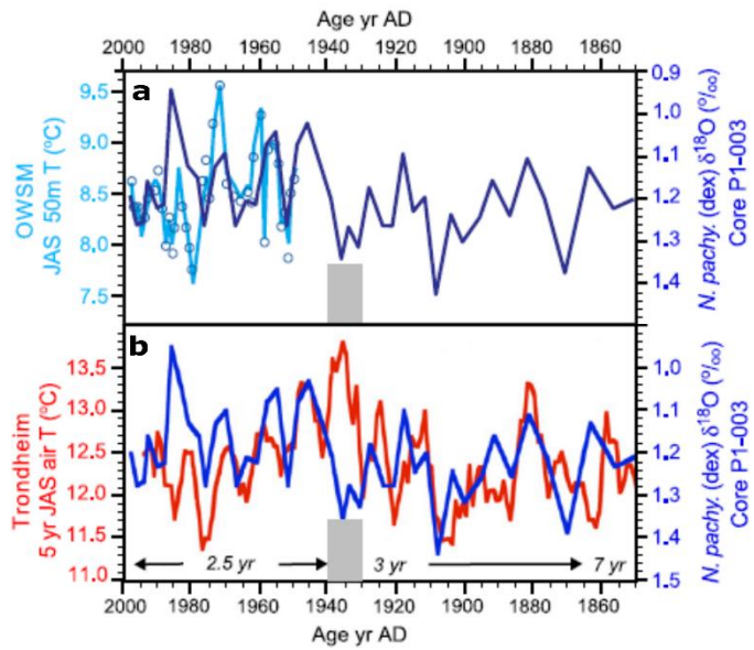
Figure 2.16 Results from Sejrup et al. (2011) where stable oxygen isotopes are compared to JAS temperature at OWSM and Trondheim (Sejrup et al., 2011).
