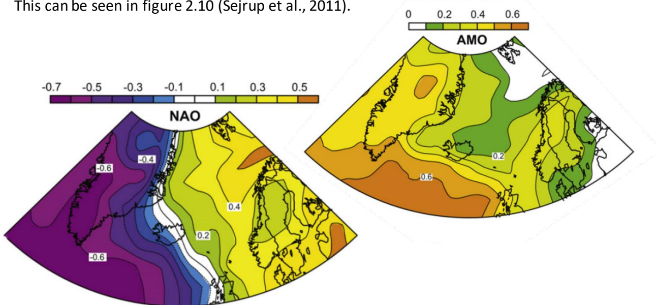
Figure 2.10 The spatial expression of the NAO (East-West gradient) and the AMO (North-South gradient) (Sejrup et al., 2011).
