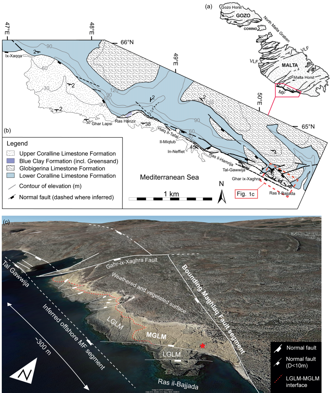
Fig. 1. (a) Map showing the location of major normal faults in Malta. MF, Maghlaq Fault; VLF, Victoria Lines Fault. Based on Dart et al. (1993) and Bonson et al. (2007) and modified from Rotevatn et al. (2016). (b) Geological map of the Maghlaq Fault, outcropping along 4 km of the southwestern coastline of Malta. Note that individual members of the stratigraphic formations are not distinguished on the map. The topographic contour intervals are in metres above sea level. Location is shown in (a). The study area is located in the WSW, marked by the red polygon and shown in (c). Based on Dart et al. (1993) and Bonson et al. (2007) and modified from Rotevatn et al. (2016). (c) Perspective view on to satellite imagery draped on digital elevation model showing the study area on the WSW coastline of Malta. The studied deformation bands are located within the MGLM interval within the fault block bounded by the Gahr ix-Xaghra Fault and the Maghlaq Fault. The location is shown in (b). The red star shows the location of the area shown in Figure 6 which is used in the reservoir models in the present study. No vertical exaggeration. MF, Maghlaq Fault; LGLM, Lower Globigerina Limestone Member; MGLM, Middle Globigerina Limestone Member. Modified from Rotevatn et al. (in review); imagery courtesy of Google Earth.
