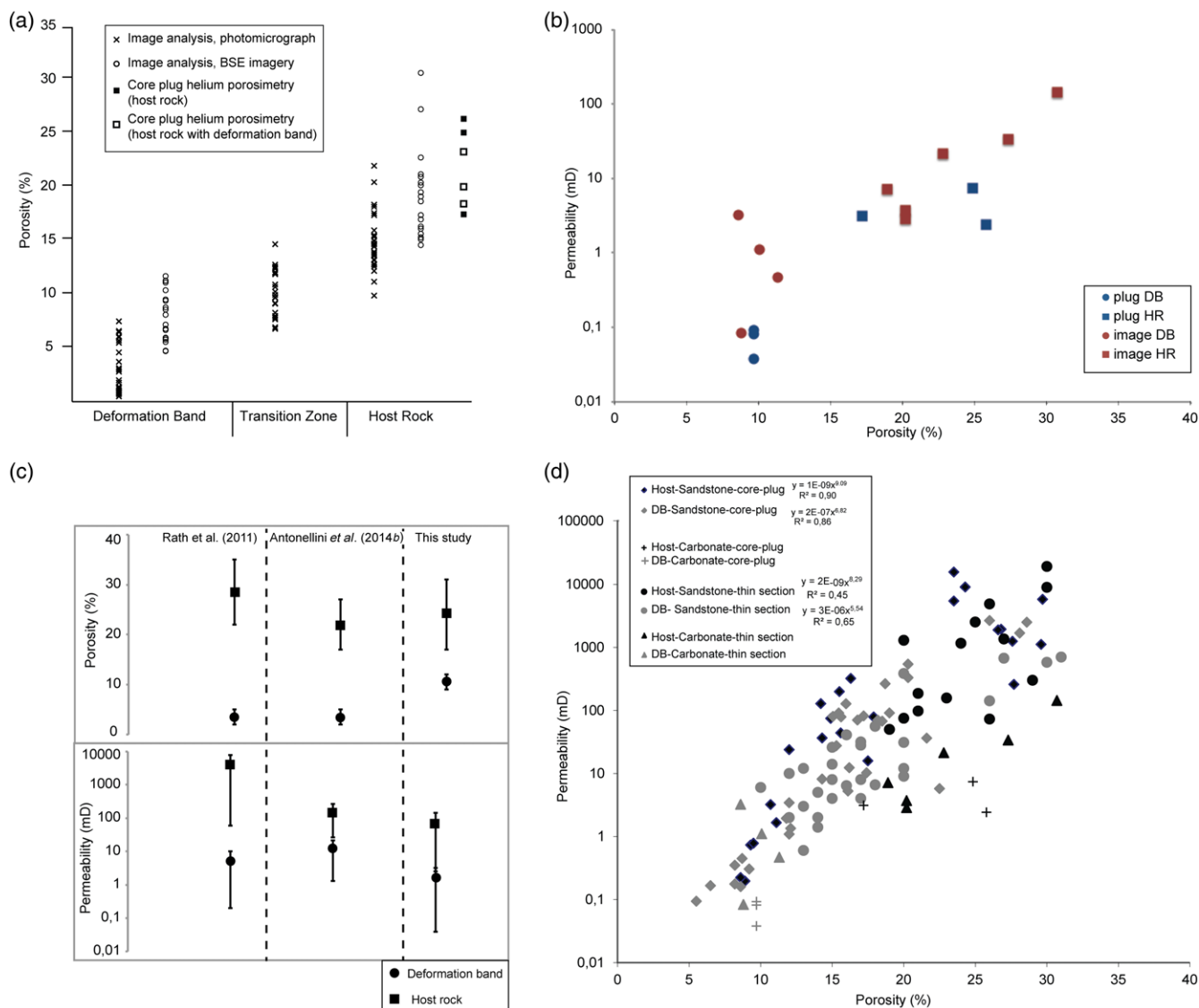
Fig. 4. Porosity and permeability data. (a) Porosity data from host rock, deformation bands and transition zones. From Rotevatn et al. (2016).
