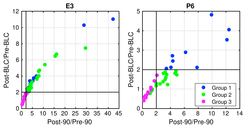
Figure 12. The ratios of postfluxes to prefluxes in BLC and 90^{\circ} fluxes are scattered for all 41 storms ((left) E3, > 292 keV; (right) P6, > 756 keV). The color indicates which group the event belongs to, as defined based on the increase seen in BLC flux (see text for full description). Some of the blue dots are overplotted by green dots in Figure 12 (left) (E3).
