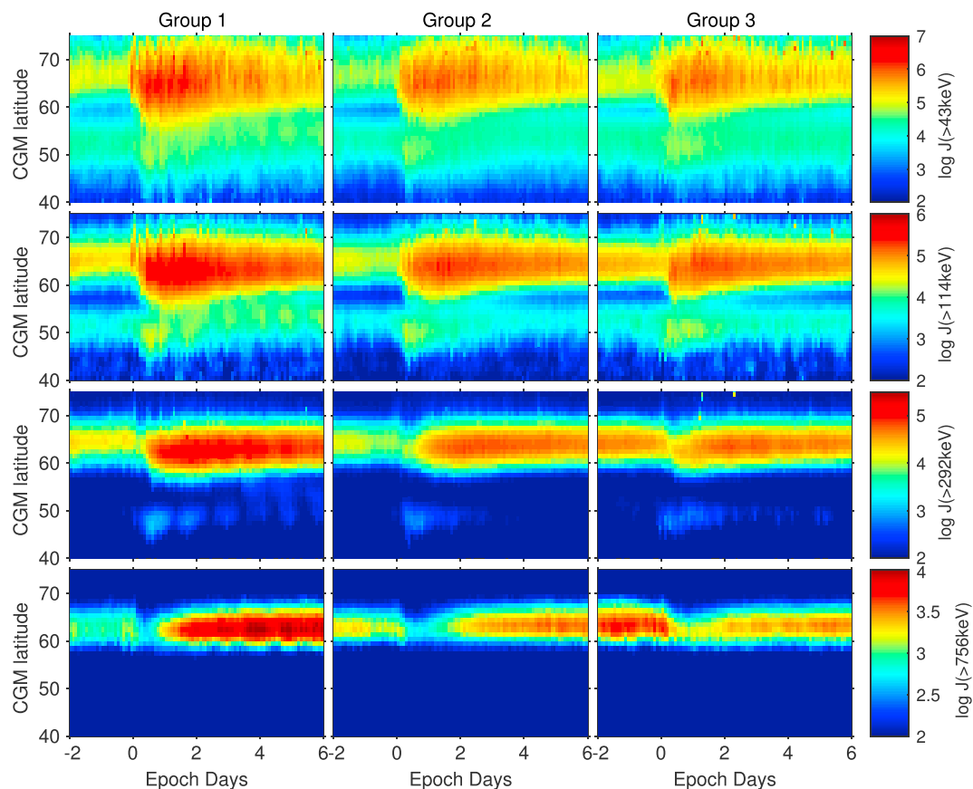
Figure 10. The same as in Figure 9 but here we plot 90° fluxes for the same groups. The range of the colorbar is identical to the BLC fluxes within each channel (and in units of integral flux [cm -2 s -1 sr -1 ]). Groups are defined based on the BLC fluxes, see the text for a detailed description.
