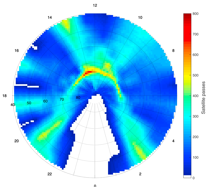
Figure 1. The total number of times a satellite entered a box of size 1 h MLT and 1^\circ corrected geomagnetic latitude during 41 storms.
