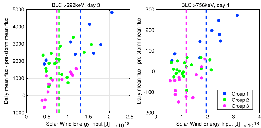
Figure 11. Prestorm flux calculated as mean over epoch hours -48 to 0 , CGM latitude 55^{\circ} – 70^{\circ} , and all MLT. Daily mean BLC flux (starting with day 1 from zero epoch) is calculated over the same geomagnetic coordinates. We subtract prestorm flux from daily mean flux and plot versus the integrated \epsilon parameter. The best correlation for E3 (P6) daily mean BLC flux is found on day 3 (4) versus energy input in Joules (integrated \epsilon from zero epoch up to, and including, day 3 (4)). Correlation coefficient irrespective of group: E3, r = 0.70 and P6, r = 0.68 . The mean energy input for each group is plotted as dashed vertical lines in the same color as the dots ((right) the green vertical dashed line is overlotted by the magenta line).
