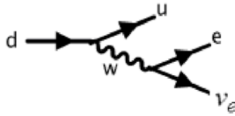
Figur 1 Feynmandiagram for beta–stråling
