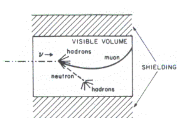
Figur 16 "Associated Event".
