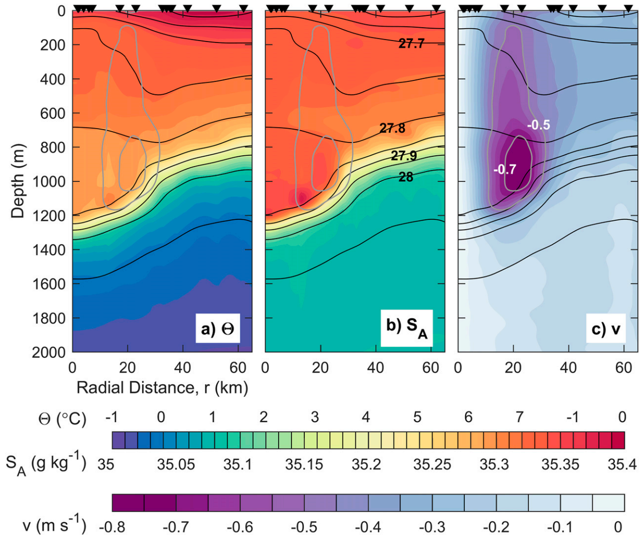
FIG. 3. Radial sections of (a) Conservative Temperature \Theta , (b) Absolute Salinity S_A , and (c) azimuthal velocity, v , obtained from the CTD/LADCP profiles collected at positions indicated at the top. In each panel, v contours for -0.5 and -0.7 \text{ m s}^{-1} are marked for reference. Black contours are for the potential density anomaly \sigma_\theta at 0.05 \text{ kg m}^{-3} intervals. Sections are obtained by referencing each station to a time-variable core position (at r = 0 ) and using optimal interpolation with correlation length scales of 20 km (horizontal) and 100 m (vertical).
