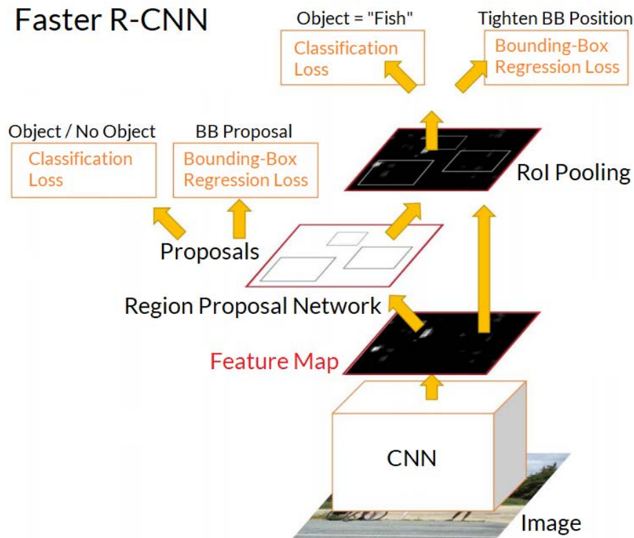
Figure 34: Overview of Faster R-CNN architecture – Adapted from [70]
