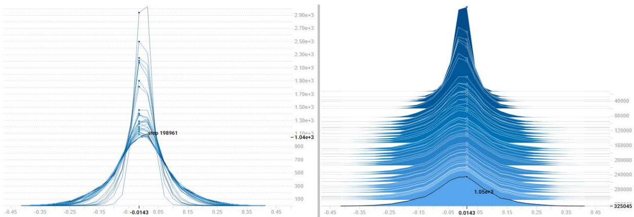
Figure 51: Change in weights over time for FRCNN ResNet 152 @2
