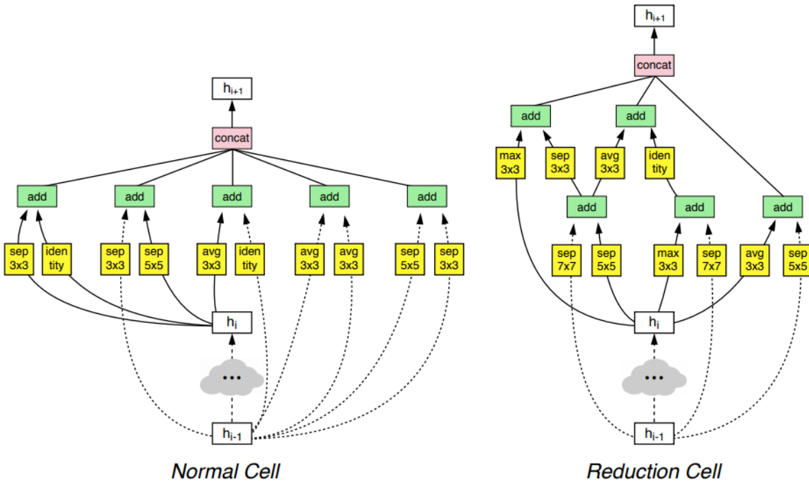
Figure 45: NASNet-A architecture with B = 5 blocks – Source [61]
