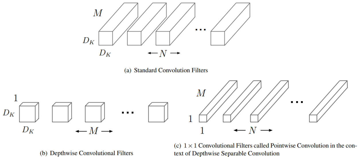
Figure 43: Standard convolution vs depthwise separable convolution – Adapted from [78]
