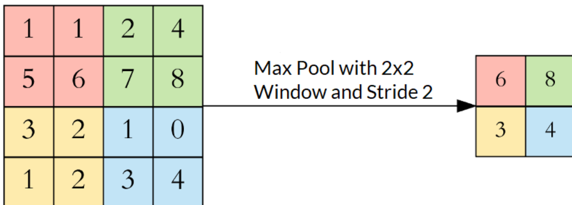
Figure 28: Applying pooling to reduce dimensionality – Adapted from [63]
