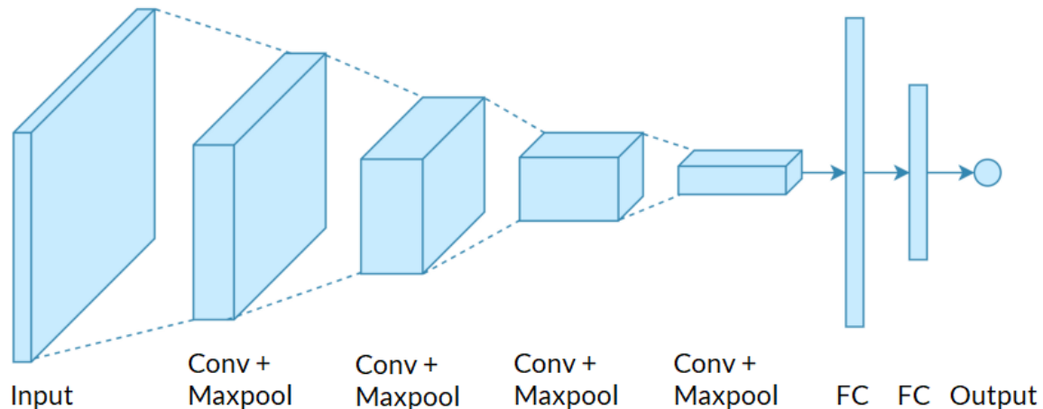
Figure 21: Convolutional neural network (CNN) architecture – Adapted from [63]
