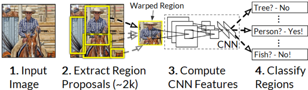
Figure 31: R-CNN step-by-step process – Adapted from [68]
