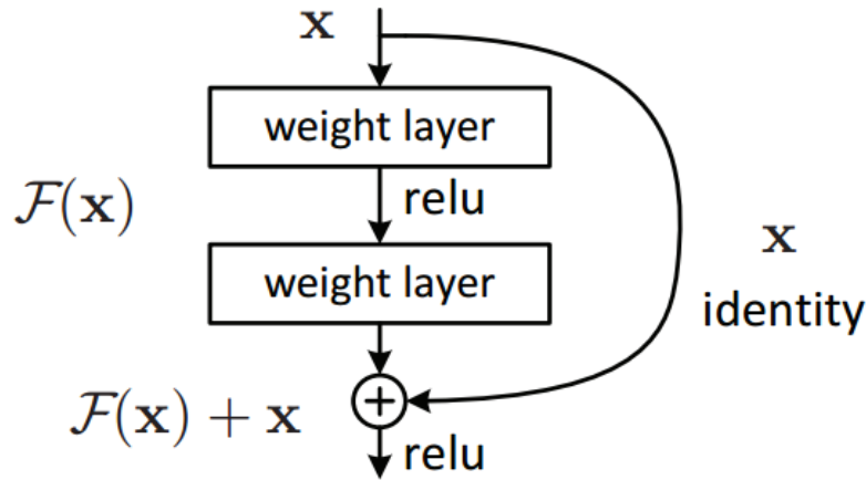
Figure 37: ResNet building block – Source [75]
