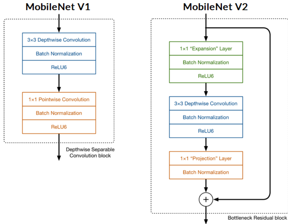
Figure 44: Comparison of the blocks in MobileNet V1 and MobileNet V2 – Adapted from [79]
