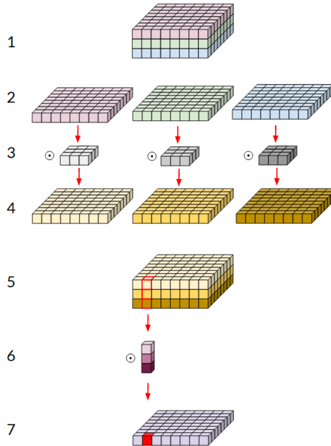
Figure 27: Depthwise (step 2 - 5) and separable (step 5 - 7) convolution – Adapted from [66]
