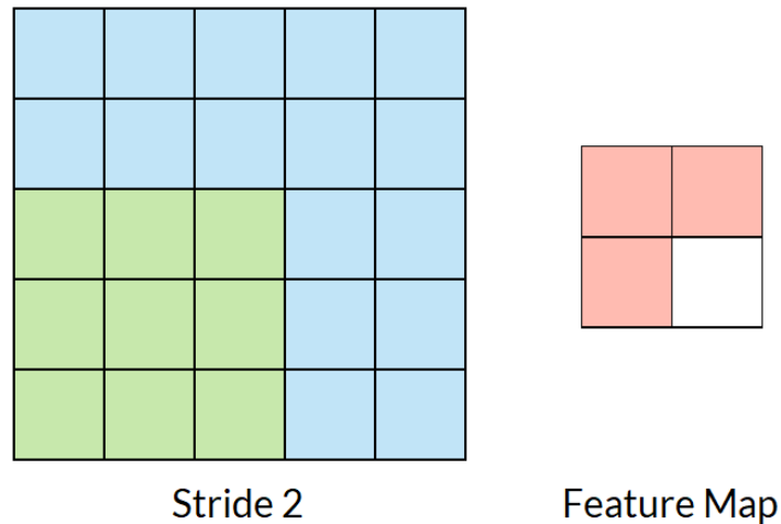
Figure 24: Filter with a stride of 2 – Adapted from [63]
