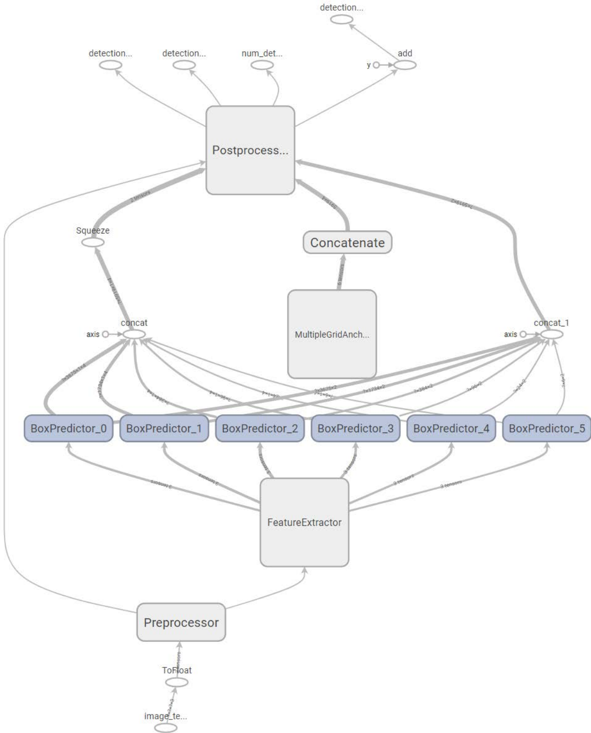
Figure 60: SSD model
