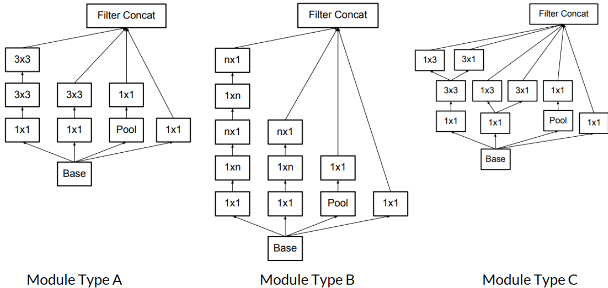
Figure 39: The three types of modules used in Inception V2 – Adapted from [77]
