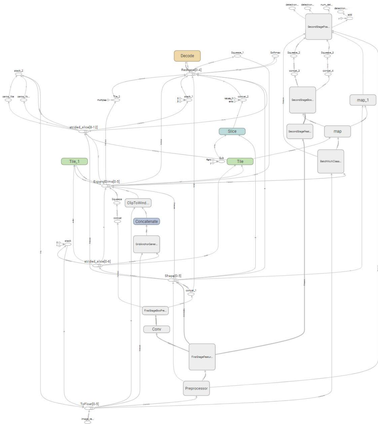
Figure 62: R-FCN model
