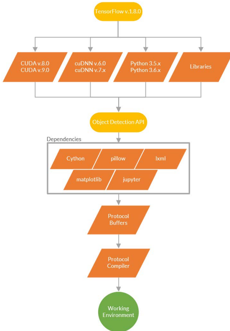
Figure 18: TensorFlow dependencies
