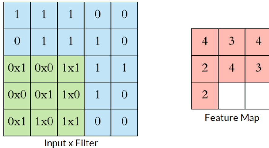
Figure 22: 2D convolution with input, filter, and feature map – Adapted from [63]
