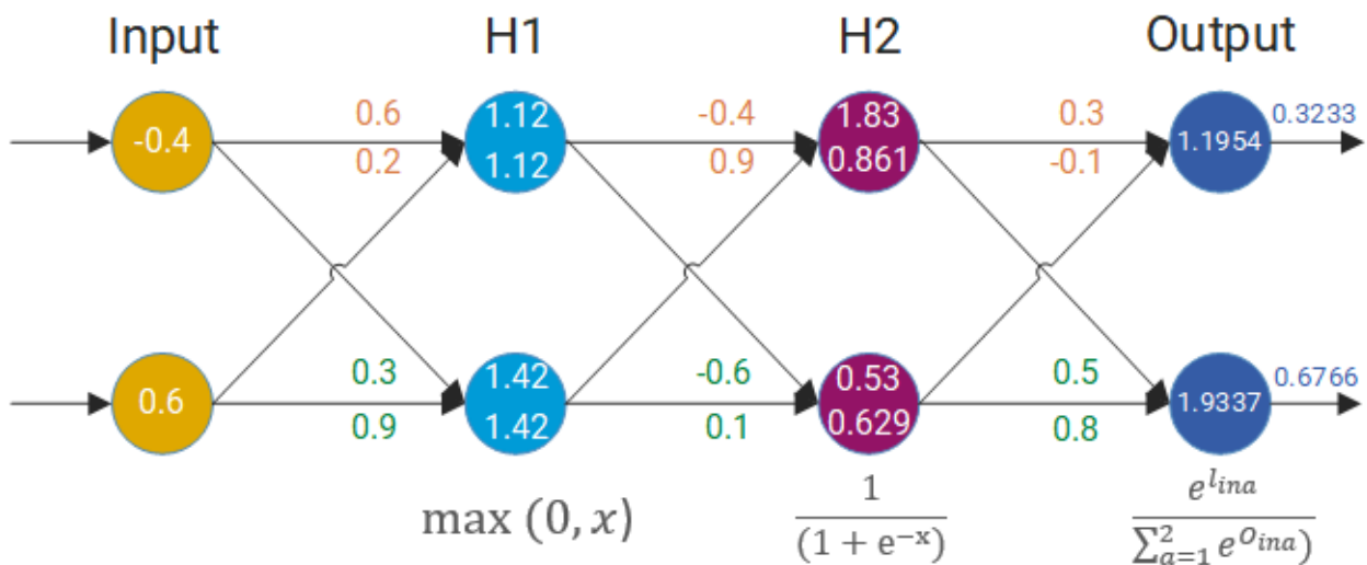
Figure 59: Results from a single forward pass in a neural network
