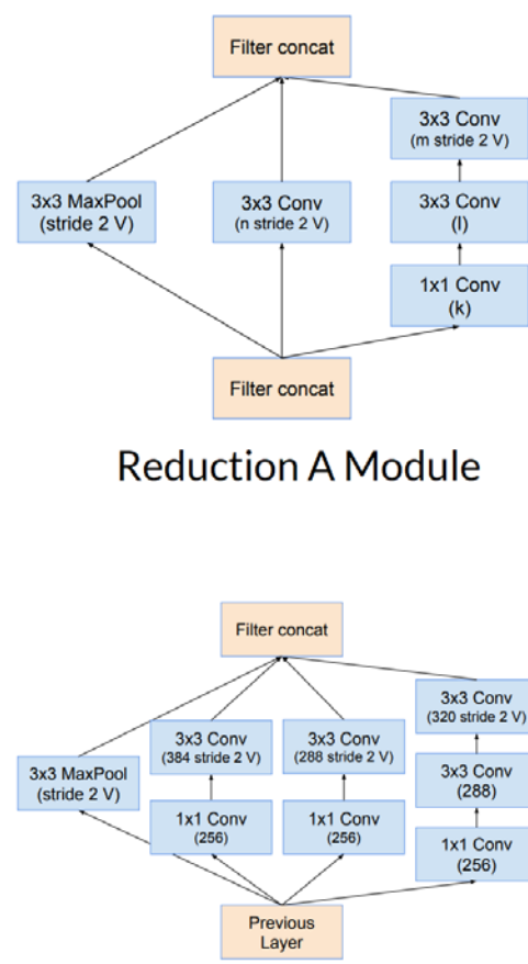
Reduction B Module
