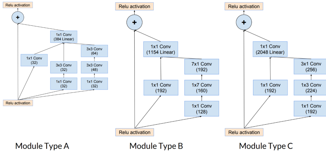
Figure 42: Inception ResNet V2 modules A, B, and C – Adapted from [59]
