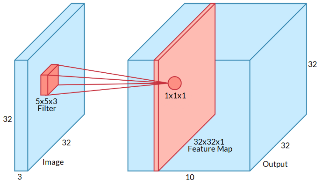
Figure 23: 3D convolution with image, filter, feature map, and output – Adapted from [63]
