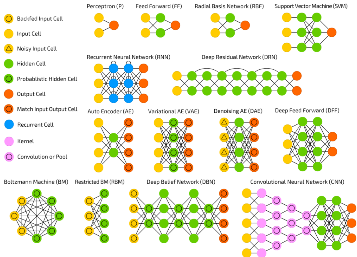
Figure 20: Chart of multiple types of neural networks – Adapted from [56]
