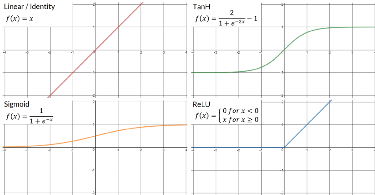
Figure 5: Common activation functions, each remapping the input values to a certain range
