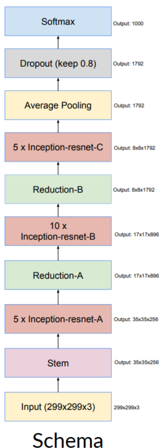
Figure 40: Inception ResNet V2 schema - Adapted from [59]
