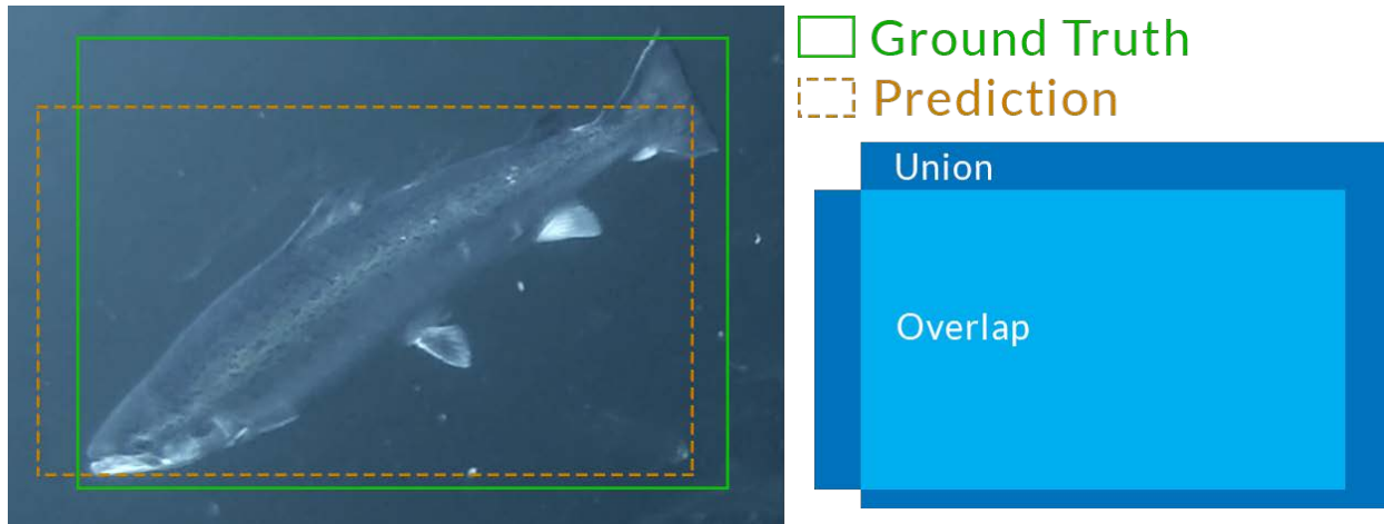
Figure 47: Intersection over Union (IoU)
