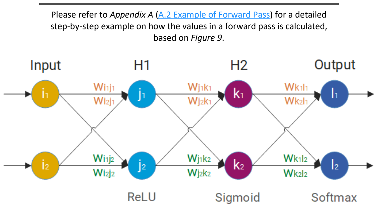
Figure 9: Notation in a neural network with two hidden layers
