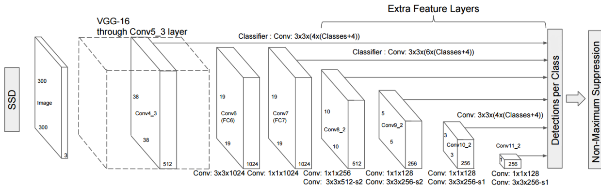
Figure 36: SSD architecture – Adapted from [74]
