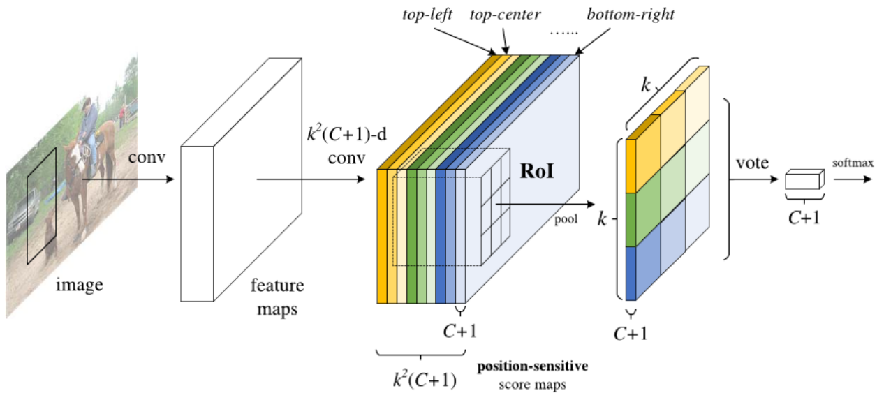
Figure 35: R-FCN architecture – Source [70, 73]
