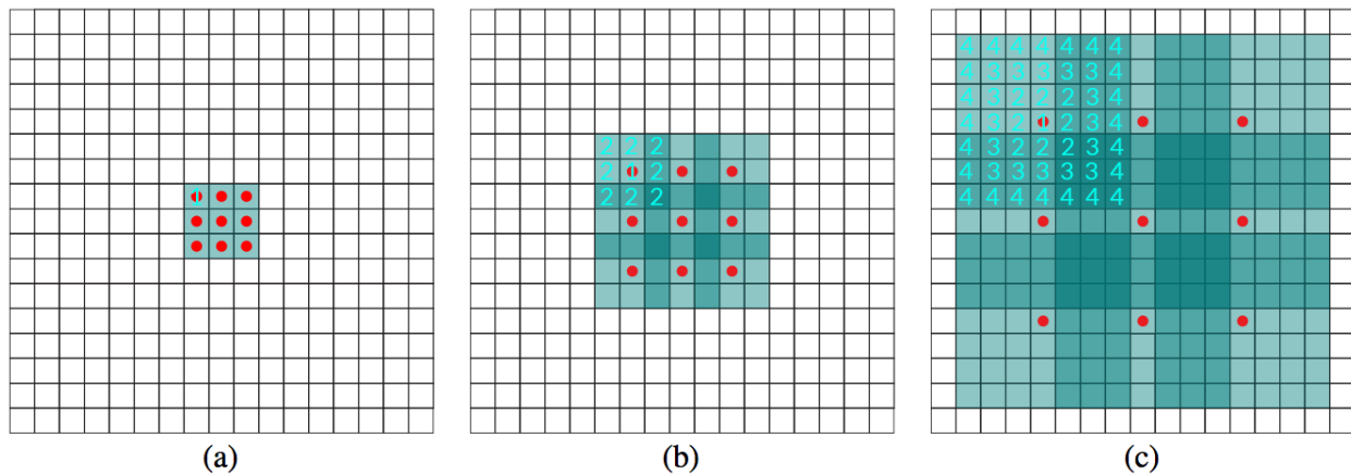
Figure 26: Increased dilation rates causes increased receptive fields – Adapted from [65]
