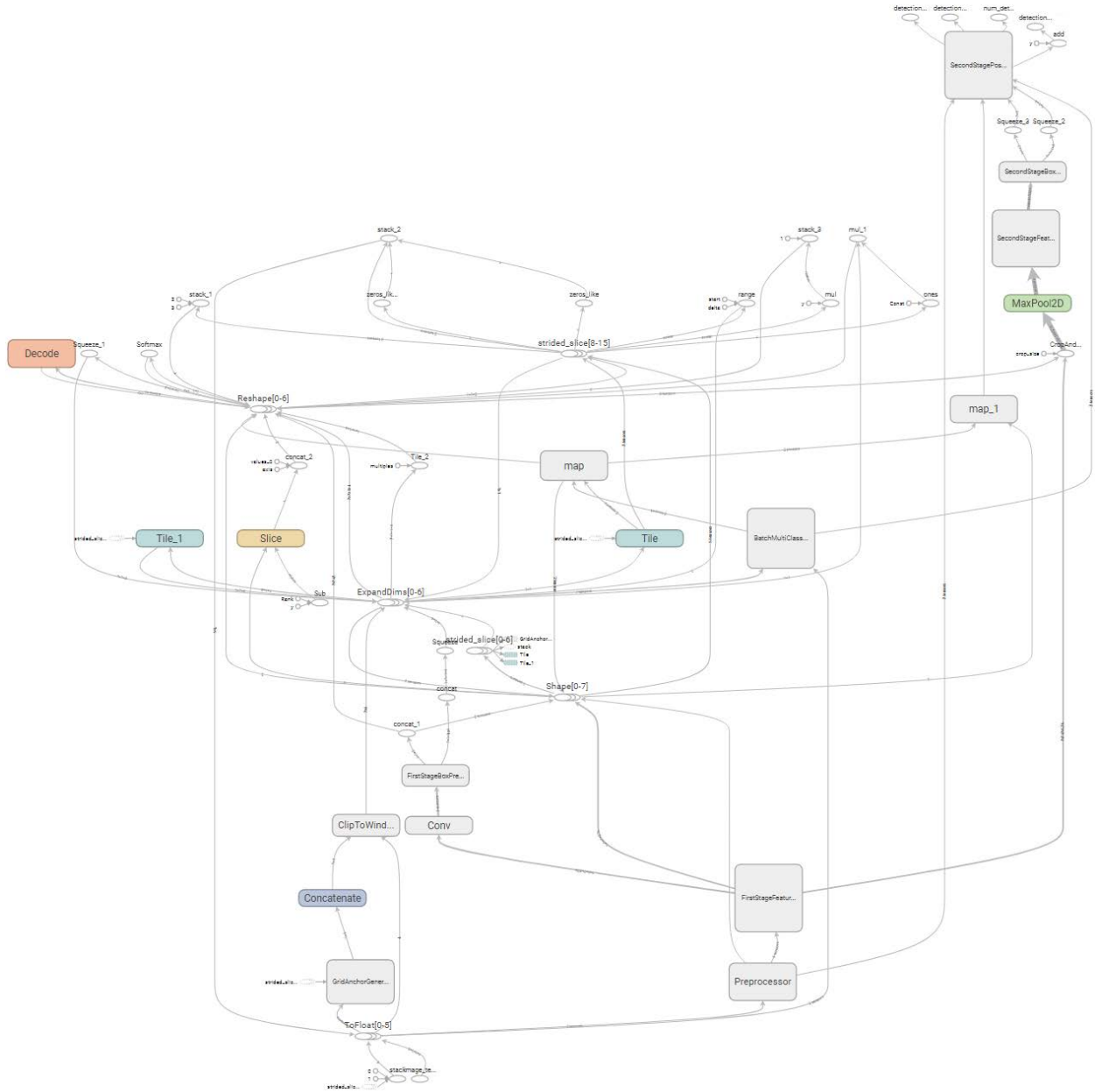
Figure 61: Faster R-CNN model
