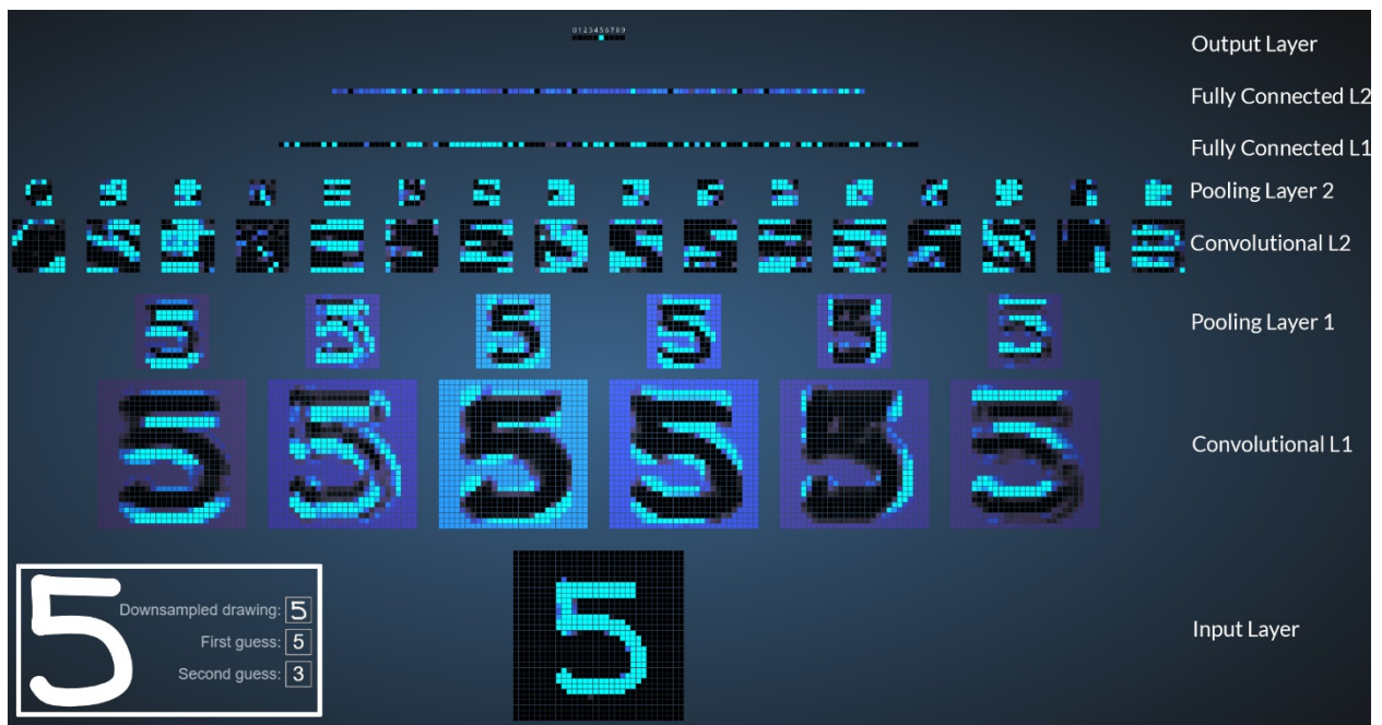
Figure 29: Visualization of a convolutional neural network (CNN) – Adapted from [67]
