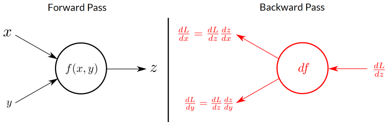
Figure 8: Forward pass and backward pass on a neuron – Adapted from [36]
