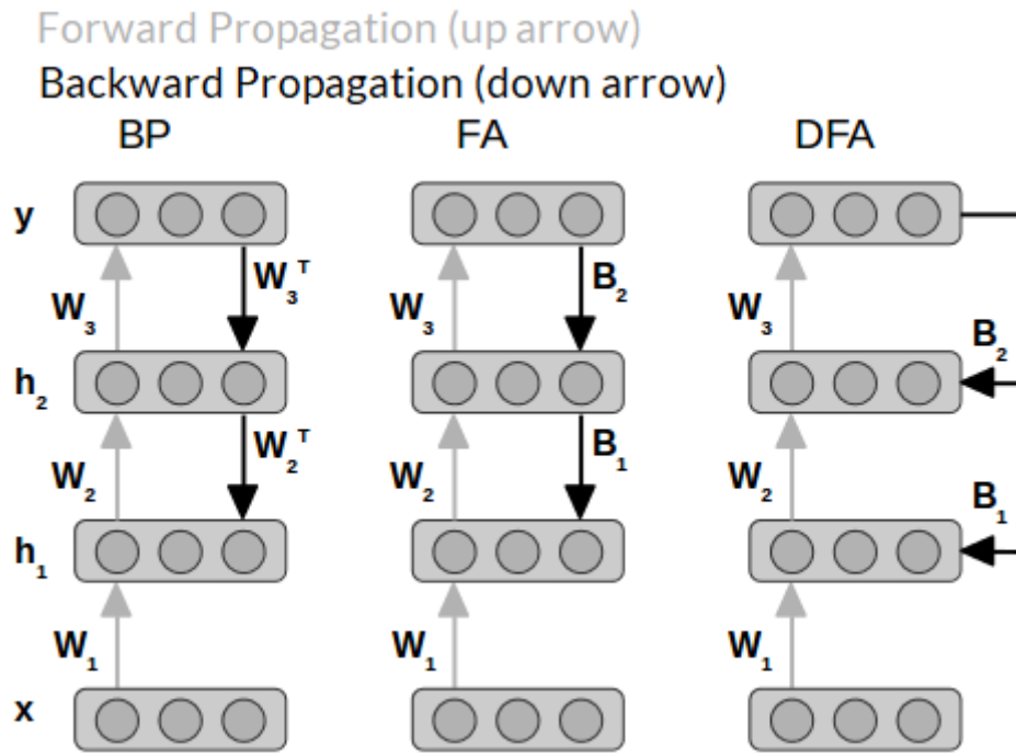
Figure 11: Backpropagation, and (Direct) Feedback Alignment – Adapted from [40]
