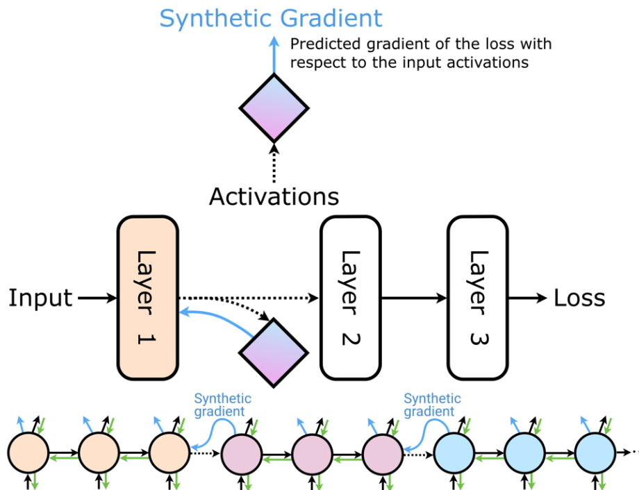
Figure 10: Illustration of Deep Neural Interfaces using Synthetic Gradient – Adapted from [39]
