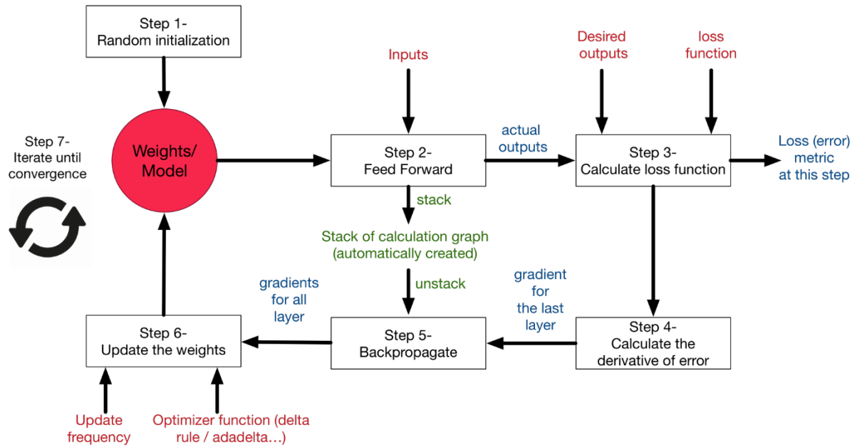
Figure 6: The learning process for neural networks – Source [33]
