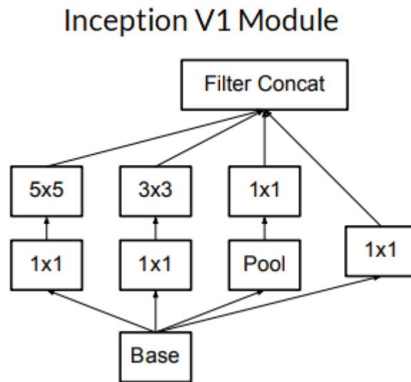
Figure 38: Inception V1 module – Source
