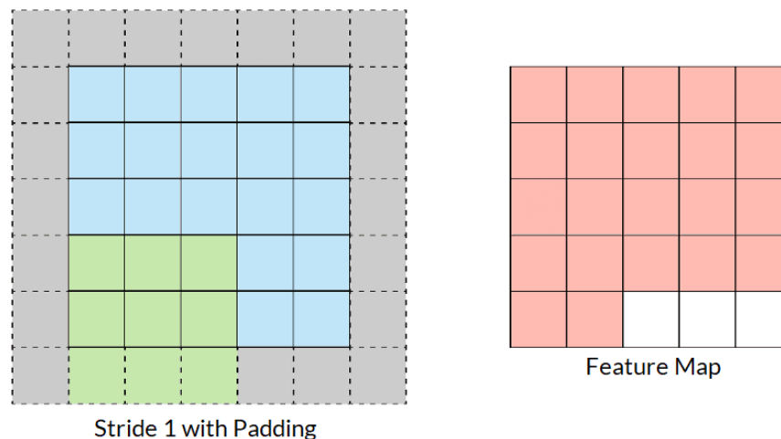
Figure 25: Padding the input to preserve the size of the feature map – Adapted from [63]
