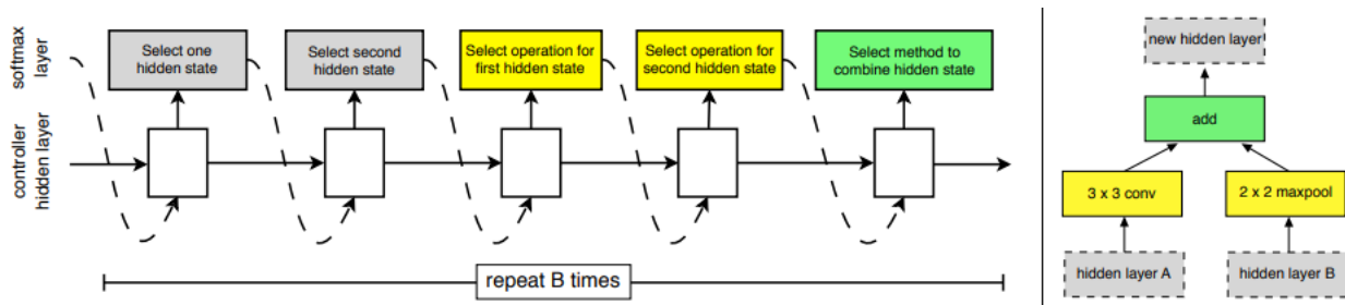
Figure 46: Controller model architecture (left) constructing one block (right) – Adapted from [61]
