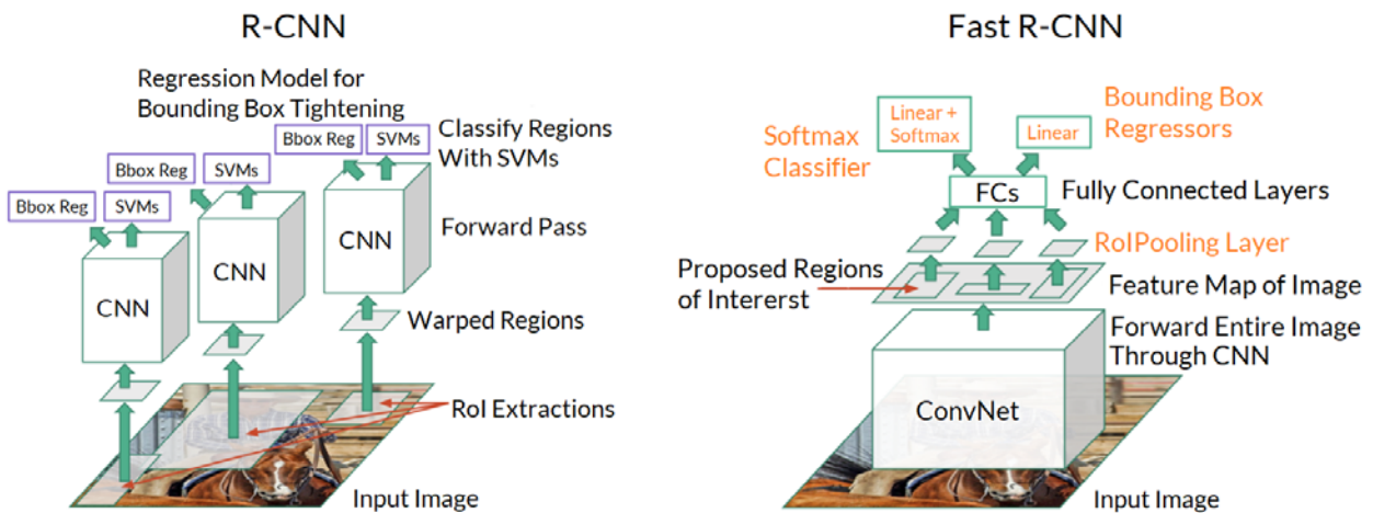
Figure 33: R-CNN compared to Fast R-CNN – Adapted from [70]
