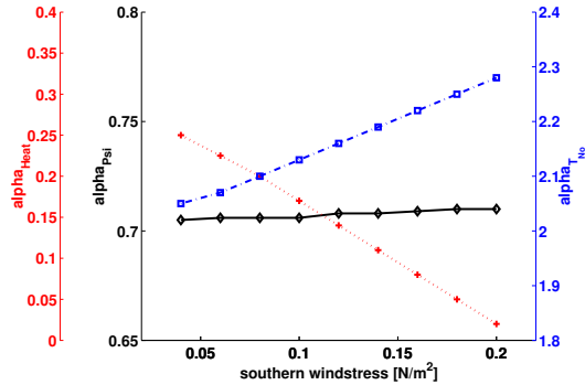
Figure 2.9: Dependency of the critical values of \alpha on the strength of southern ocean wind forcing. Lines as in fig. 2.7
