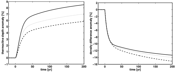
Figure 2.2: Left: anomaly of the thermocline depth after the freshwater flux is increased by 50% at t = 0 . Dashed line \alpha = 0 , dotted line \alpha = 0.5 , solid line \alpha = 1 . Right: anomaly of the density difference between the thermocline and northern boxes.
