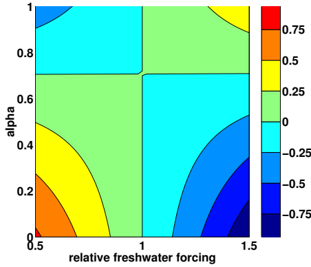
Figure 2.3: Anomaly of the northward volume transport \Psi_{\text{No}} [Sv] as a function of the relative freshwater forcing F_n , and \alpha . F_n = 1 corresponds to the default value of 0.24 Sv, the zero anomaly contour corresponds to 18 Sv of overturning.
