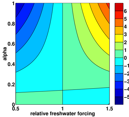
Figure 2.4: As fig. 2.3, but for the anomaly of the northward effective heat transport [%]. The zero anomaly contour corresponds to \sim 1.2 PW heat transport in the model.
