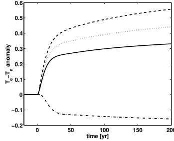
Figure 2.6: Anomaly of the temperature difference between low latitudes and northern box. Dashed, dotted, solid as in figures 2.2 and 2.5, dash-dotted for \alpha = 3
