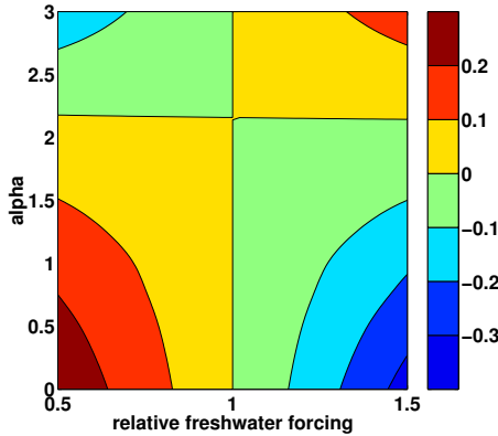
Figure 2.8: Anomaly of temperature of the northern and deep box T_n [K] as a function of F_n and \alpha (note that the scale for \alpha is different from the previous plots)
