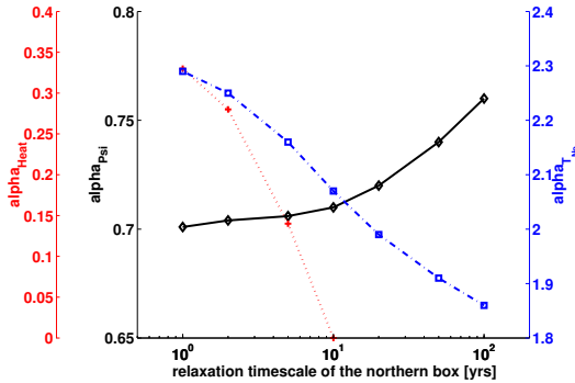
Figure 2.7: Dependency of the critical values of \alpha on the timescale of temperature relaxation in the northern box. Dotted line: \alpha_{Heat} , dash-dotted line: \alpha_{T_{No}} , solid line: \alpha_{Psi}
