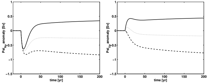
Figure 2.5: As figure 2.2, but left: anomalous northward volume transport. Right: upwelling into the thermocline box.
