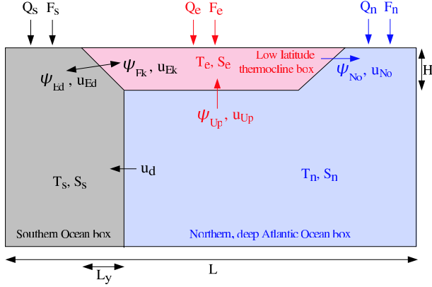
Figure 2.1: Schematic representation of the model
