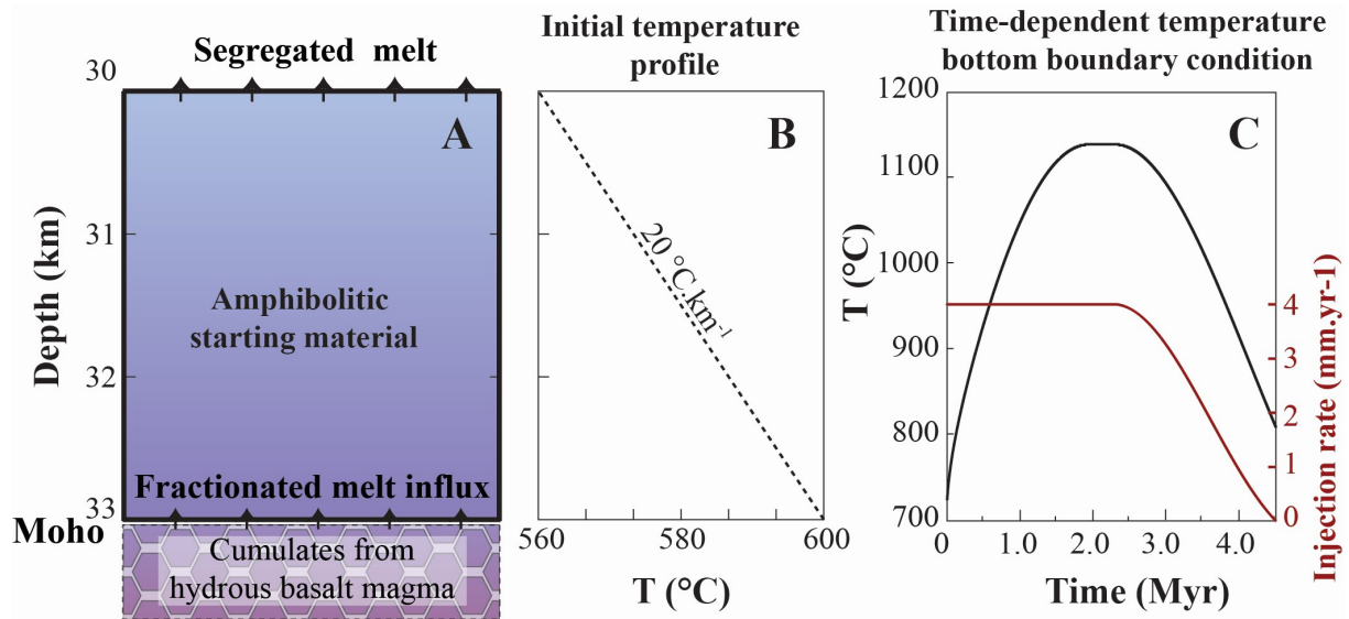
Figure 6. Model setup. A, Schematic representation of the modeled region. Fractionated melt from crystallizing mantle melts are injected at the bottom boundary, while extracted melts segregated from the crust are captured at the top boundary. B, Initial temperature profile. C, Time-dependent temperature bottom boundary condition. Note that temperature is maintained constant between \sim 2 and 2.5 Myr in order to reach a steady state. Then the temperature slowly decreases down to 4.5 Myr. During the cooling phase, the rate of mantle-derived magma emplacement is progressively decreased to 0.
