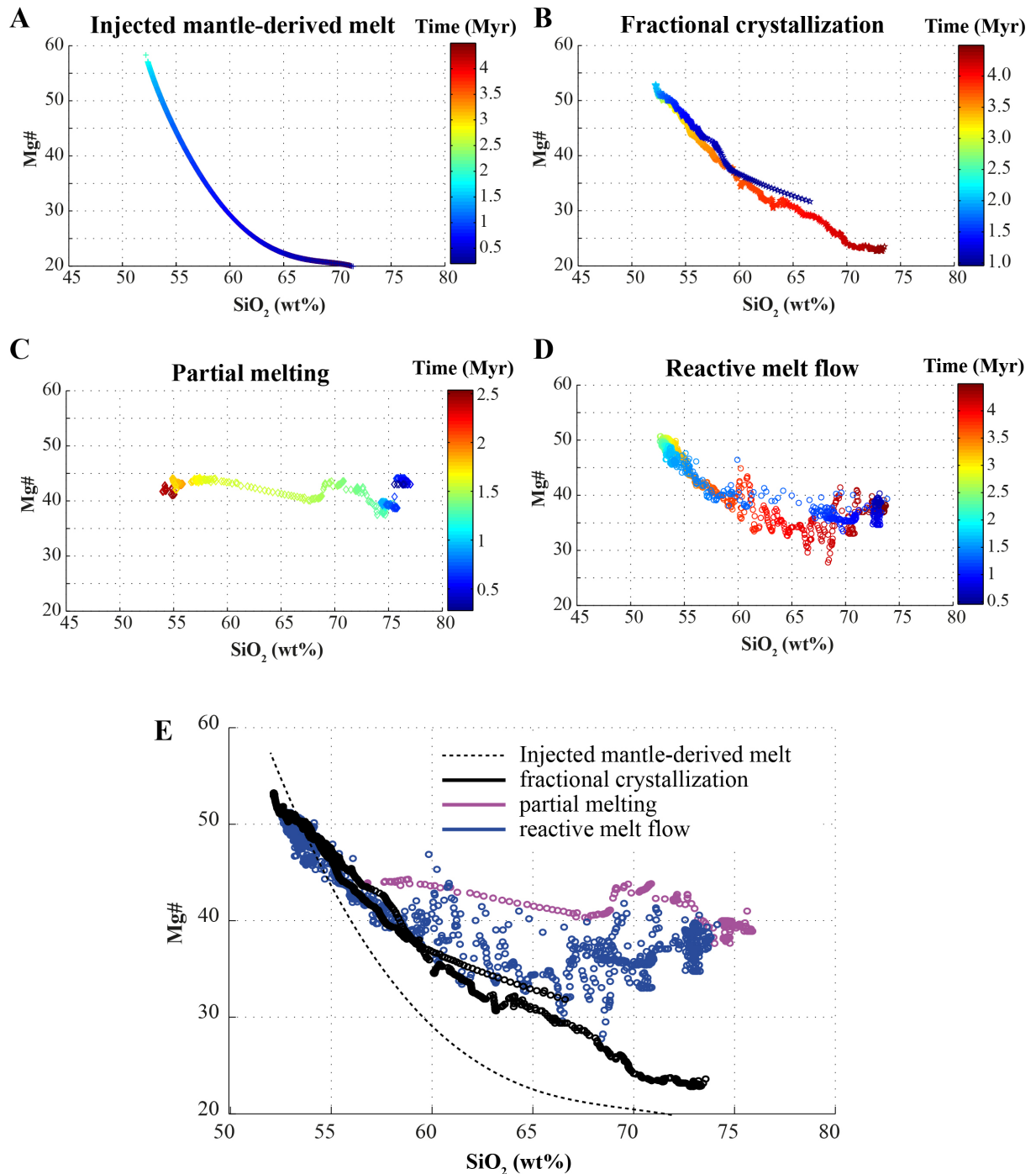
Figure 10. Mg# versus SiO 2 diagram of incoming mantle melts compared to melt output for the PM, FC and RMF models. A, Injected mantle-derived melt trend colored as function of time. B, Fractional crystallization model trend colored as function of time. C, Partial melting model trend colored as function of time. D, Reactive melt flow model trend colored as function of time. E, Comparison between incoming mantle melts (parameterized dash line) compared to melt output for the PM model (purple dots), FC model (black dots) and a fully reactive RMF model (blue dots).
