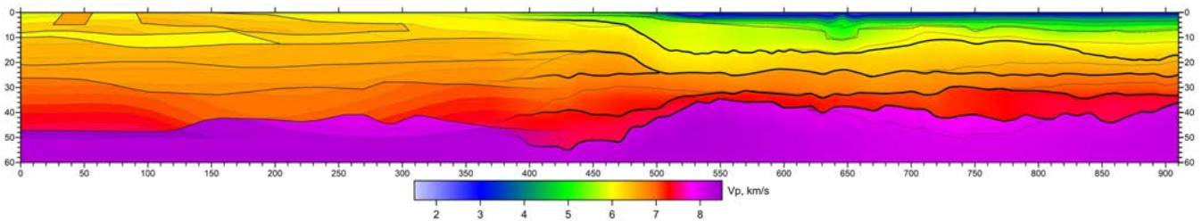
Figure 9. A combined plot, showing results from two different seismic profiles merged together (see Fig. 1 for locations). The colour-coding is identical for both profiles and represents Vp velocities. Left—results of the EGT Polar profile (Luosto et al. 1989); right—results from the present study. The overlap zone of two profiles is located between offsets 380–470 km.
