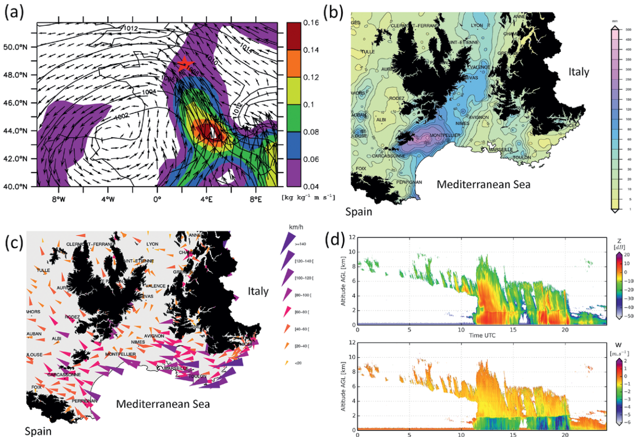
FIG. 10. (a) ERA-Interim moisture fluxes at 850 hPa (arrows; shading shows magnitude) and surface pressure (black contours; hPa) at 1200 UTC 13 Oct 2016. The red star indicates the location of the SIRTA surface observation site. (b) Daily accumulated precipitation (mm) and (c) daily maximum of instantaneous surface wind in southern France on 13 Oct 2016 from the high-resolution climatological network of Météo-France surface weather stations. The black areas in (b) and (c) mark the topography of the French Pyrenees, the Massif Central, and the French Alps. (d) Reflectivity and Doppler velocity (approximately equal to terminal fall speed) at the 25-m resolution of the BASTA radar at SIRTA on 13 Oct 2016.
