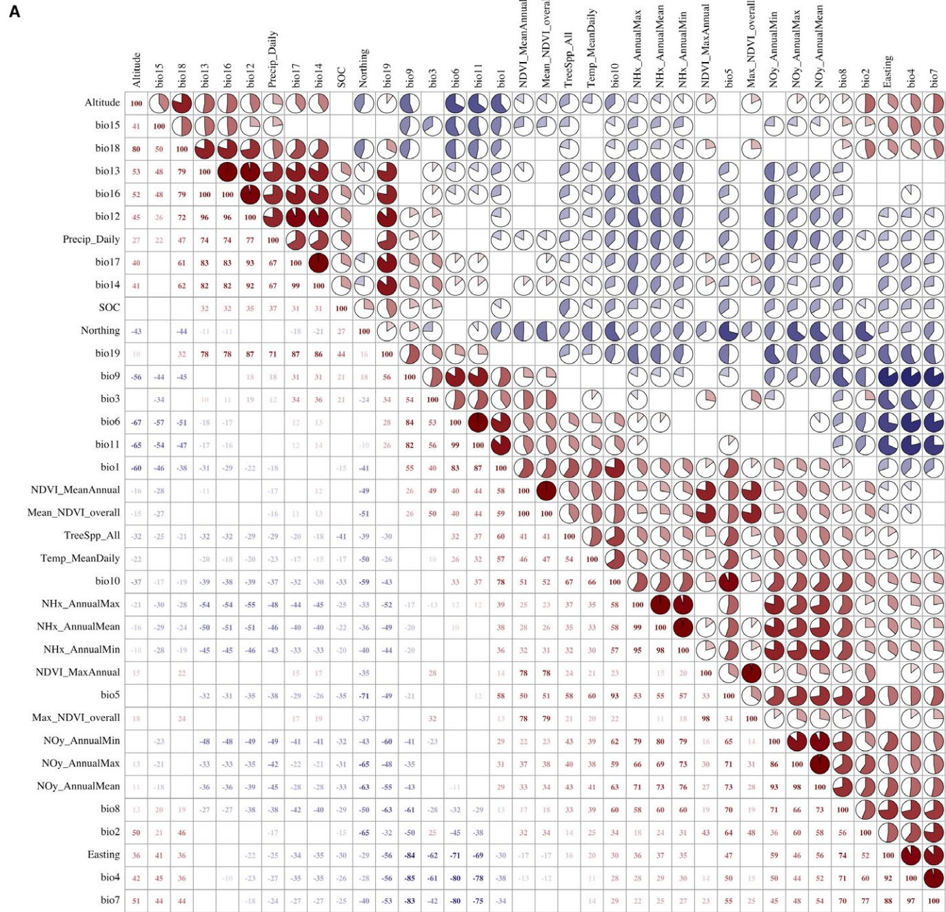
APPENDIX 5. Collinearities between all of the original potential explanatory variables for 50 × 50-km grids of saprotrophic fungi. The variables are averages, based on fruit body presences, from the most specific temporal resolutions and spatial scales, across the 40-year time period. Variables are ordered along the axes by general type (A) and similarity (B) based on hierarchical clustering.
