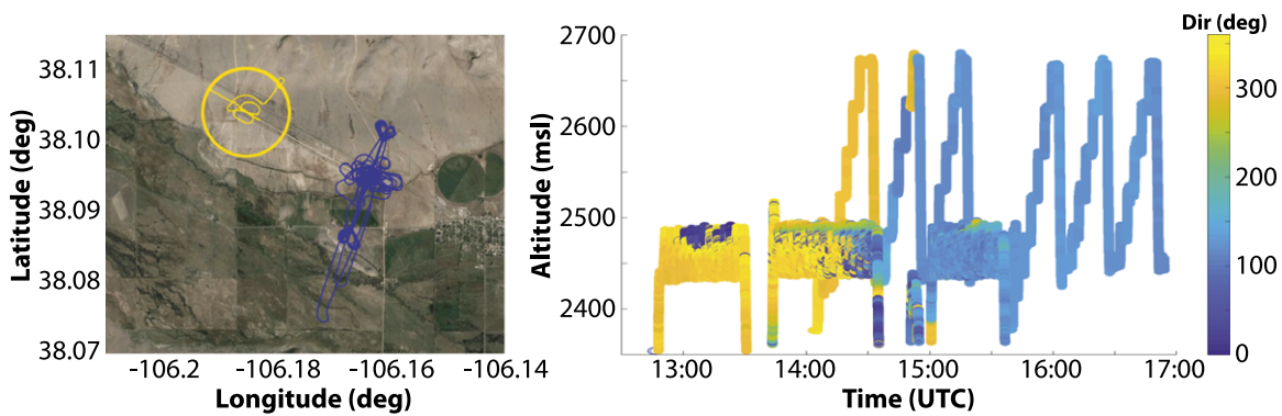
Fig. 7. Measurements from flights conducted by the University of Colorado TTWistor and University of Kentucky BLUECAT5 aircraft on 19 July to evaluate cold-air drainage from the San Luis Valley. (left) Locations of the flights (yellow points are the University of Colorado aircraft; blue points are the University of Kentucky aircraft). (right) Time–height cross section of the measured wind directions from both aircraft (the stair-step patterns are the CU TTWistor).
