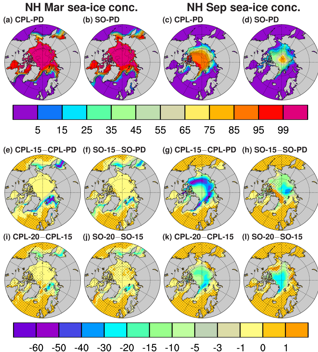
Figure 19. NH monthly-mean sea-ice concentrations for PD (a–d), the 1.5 °C warming relative to PD (e–h), and the 0.5 °C warming (i–l) from NorESM1-Happi (a, c, e, g, i, k) and NorESM1-HappiSO (b, d, f, h, j, l). Fields are shown for March (a, b, e, f, i, j) and September (c, d, g, h, k, l). The modelled concentrations are from the default 90-year periods (Sect. 3.2). The PD results (colours; top colour bar) are shown together with observational estimates (OSI-SAF, 2017; solid black contours) from 2006 to 2015. Differences that are not statistically significant at the 5% level according to the Mann–Whitney U test are marked with black dots. Units are percentages of ocean surface area (a–l).
