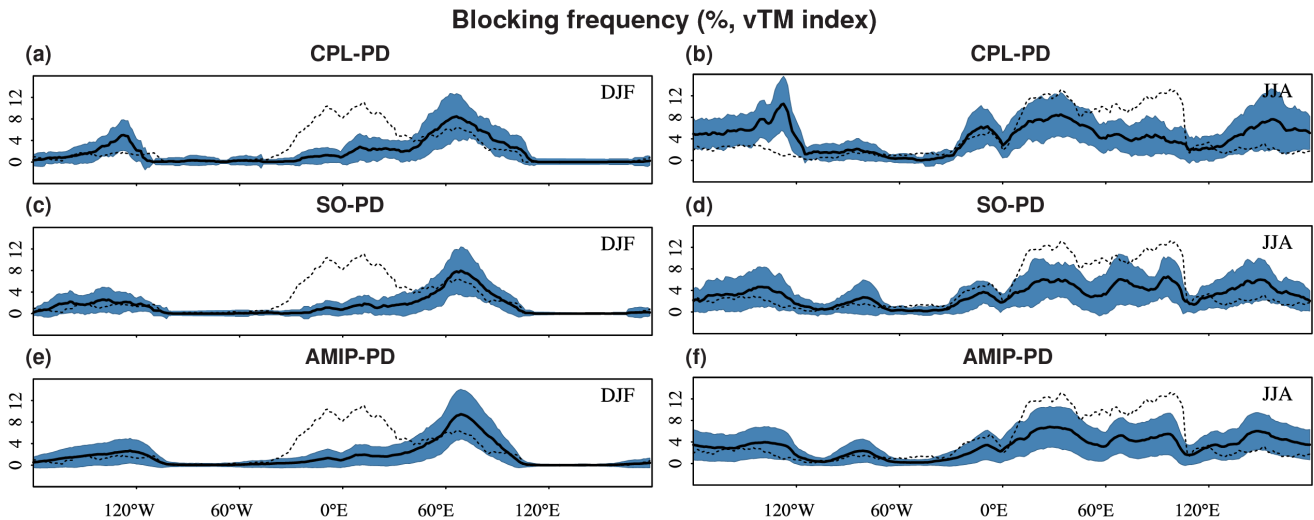
Figure 17. PD climatology of blocking frequency from NorESM1-Happi (a, b), NorESM1-HappiSO (c, d), and NorESM1-HappiAMIP (e, f) for DJF (a, c, e) and JJA (b, d, f). Shown are the mean (solid black line) and the spread (blue shading; \pm 1 SD) computed over the number of available decades (nine for NorESM1-Happi and NorESM1-HappiSO, and 125 for NorESM1-HappiAMIP) for the default time periods given in Sect. 3. Blocking frequency from ERA-Interim is shown for the period 1986–2015 (dotted black line). The blocking events are identified using the Tibaldi and Molteni (1990) blocking index with variable central latitude (vTM) (Tibaldi and Molteni, 1990; Pelly and Hoskins, 2003), as in Iversen et al. (2013). It is based on the TM index (Tibaldi and Molteni, 1990), which uses a persistent reversal of the meridional gradient of the 500 hPa geopotential height around the predefined central blocking latitude at 50° N as an indicator for blocking. The reversal must be present at 7.5° consecutive longitudes and persist for at least 5 d. In the vTM index, the requirement of a predefined central blocking latitude is relaxed in order to reduce spurious detection (Pelly and Hoskins, 2003). The central latitude is allowed to vary with longitude following the latitude of the maximum in the climatological storm track (using bandpass-filtered geopotential height at 500 hPa). To account for the seasonal cycle of the cyclone activity, the central latitude for a given month is calculated as the climatological 3-month moving average centred on that month. Units are percentages (a–f).
