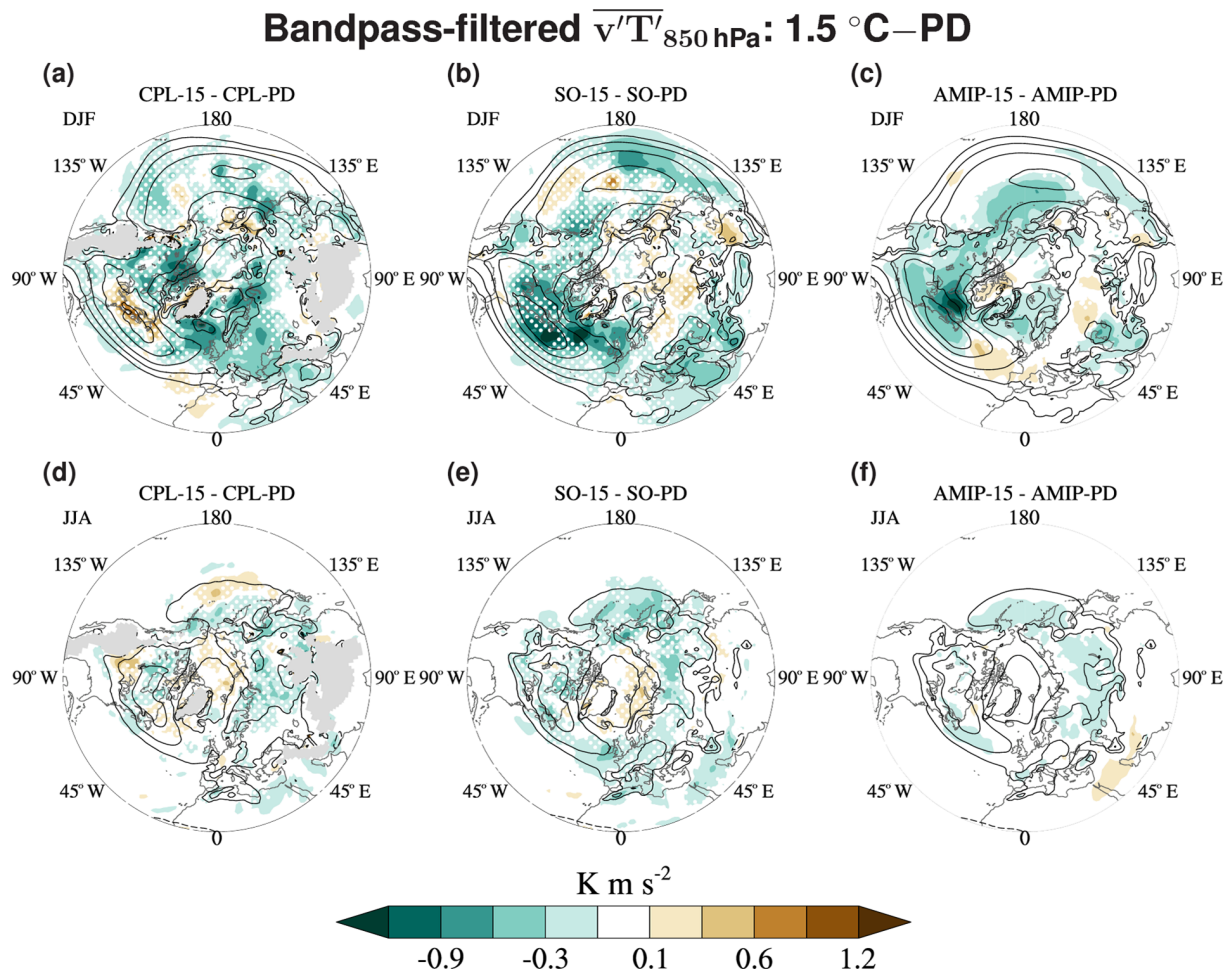
Figure 15. Changes in the low-level storm-track activity relative to PD (colours) and PD climatology (black contours; -12 to 12 \text{ K m s}^{-2} in increments of 4 \text{ K m s}^{-2} ) for the 1.5^\circ\text{C} experiment from NorESM1-Happi (a, d), NorESM1-HappiSO (b, e), and NorESM1-HappiAMIP (c, f) for DJF (a–c) and JJA (d–f). The storm tracks are represented in terms of the bandpass-filtered eddy heat flux v'T' at 850 hPa. The white dots indicate that the differences are not significant at the 5% level according to the Welch t test. The fields are shown for the default periods given in Sect. 3. Units are in \text{K m s}^{-2} (a–f).
