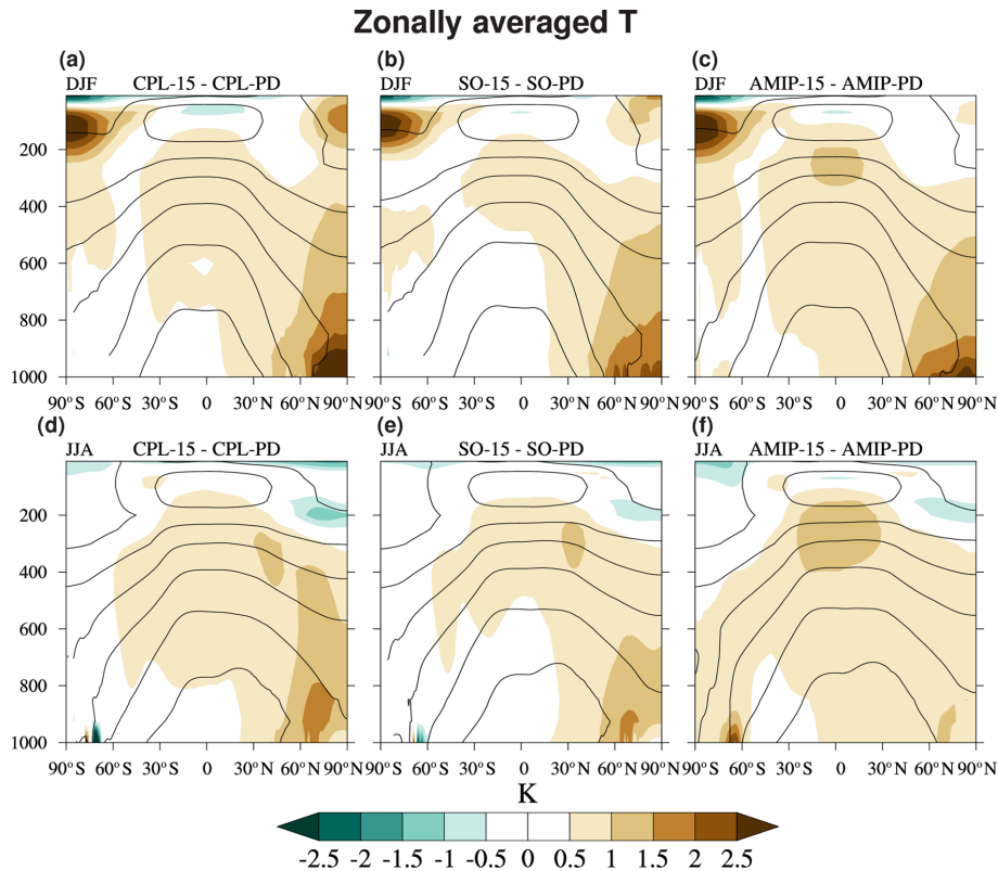
Figure 9. Zonal-mean temperature response relative to PD (colours) and climatology (solid black contours; 210 to 285 K in increments of 15 K) for the 1.5 °C experiment from NorESM1-Happi (a, d), NorESM1-HappiSO (b, e), and NorESM1-HappiAMIP (c, f). Fields are shown for DJF (a–c) and JJA (d–f) for the default periods given in Sect. 3. Units are in Kelvin (a–f).
