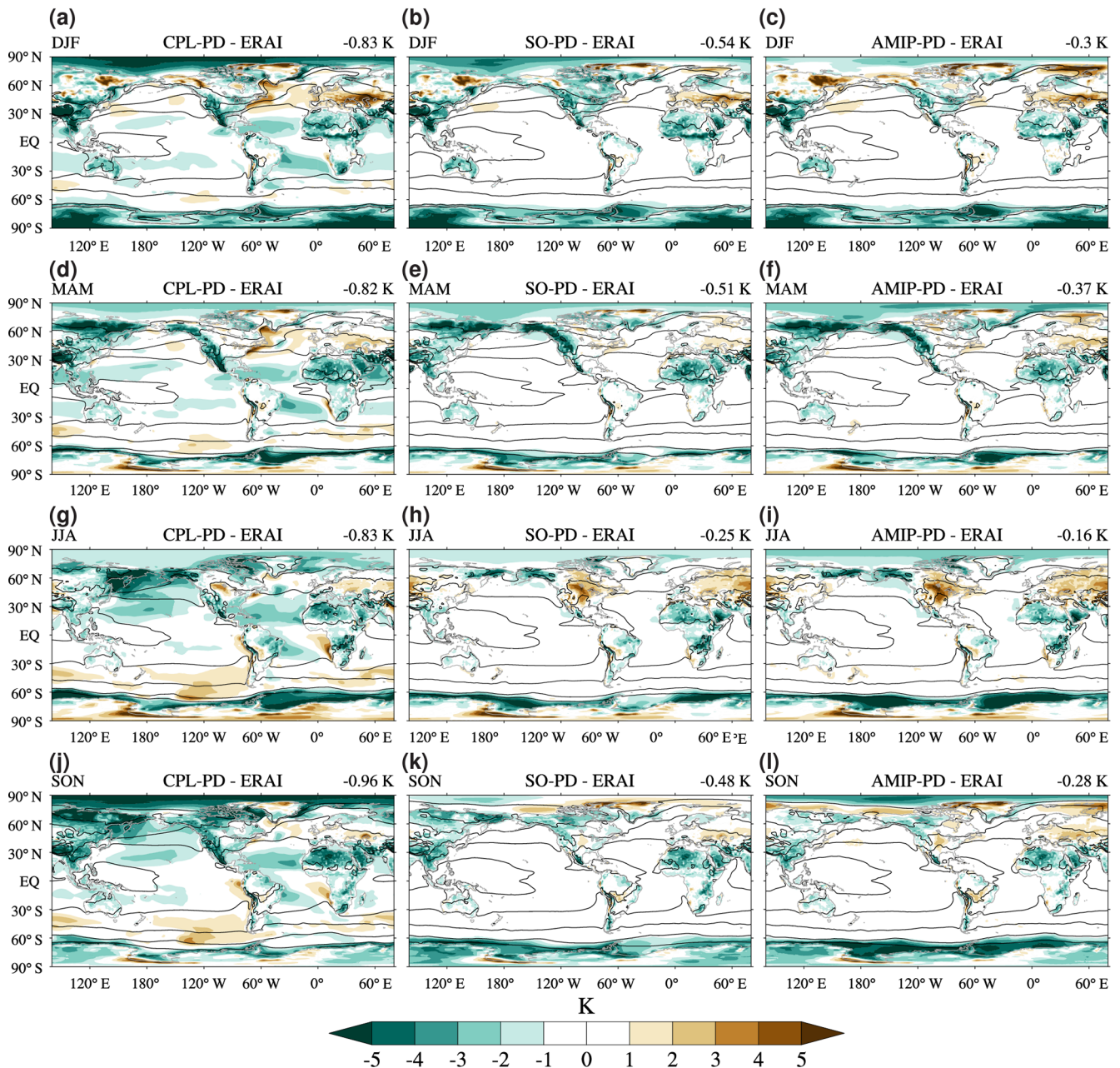
Figure 5. Near-surface temperature bias relative to ERA-Interim (colours) and near-surface temperature climatology (black contours; 260 to 350 K in increments of 10 K) for PD experiments from NorESM1-Happi (a, d, g, j), NorESM1-HappiSO (b, e, h, k), and NorESM1-HappiAMIP (c, f, i, l). We use the years 1986–2015 from ERA-Interim. The time periods for the NorESM experiments are the default periods given in Sect. 3. The global-mean ensemble-mean bias is given in the upper-right corner of each panel. Units are in Kelvin (a–l).
