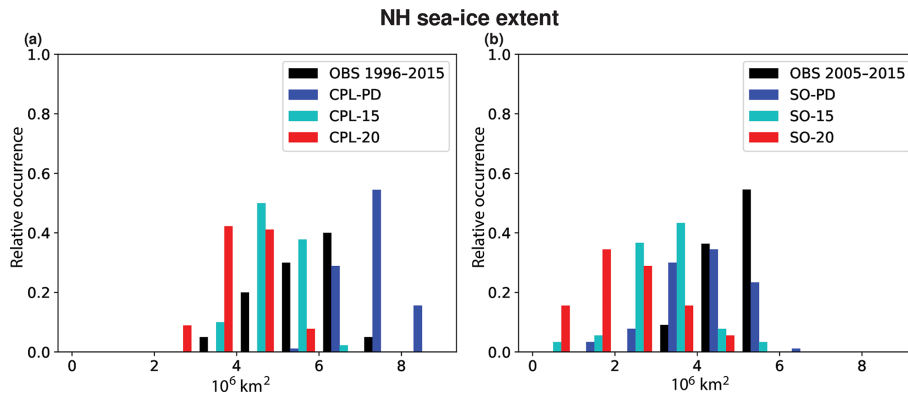
Figure 20. The relative occurrence of NH monthly-mean sea-ice extent in September for observations (black bars; OSI-SAF, 2017), the PD experiments (blue bars), and the 1.5 °C (green bars) and 2.0 °C warming experiments (red bars) from NorESM1-Happi (a) and NorESM1-HappiSO. The sea-ice extent is binned in 1.0 \times 10^6 \text{ km}^2 increments. The observations are from 1996 to 2015 (20 values) in panel (a) and from 2005 to 2015 (11 values) in panel (b). The values from NorESM1-Happi and NorESM1-HappiSO are from the default 90-year periods (Sect. 3.2). Units are in 10^6 \text{ km}^2 (a, b).
