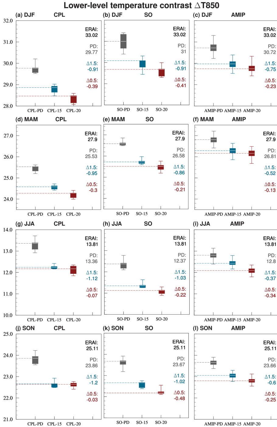
Figure 11. As in Fig. 10 but for the lower tropospheric temperature contrast at 850 hPa ( \Delta T_{850} ).
