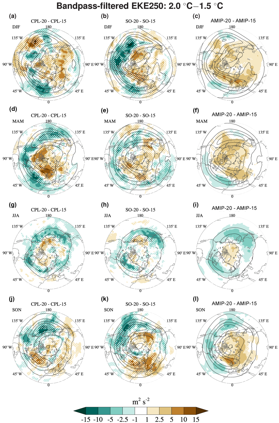
Figure 14. As in Fig. 13 but for the upper-level storm-track response to the additional 0.5 °C warming (i.e. the difference between the respective 2.0 and 1.5 °C experiments).
