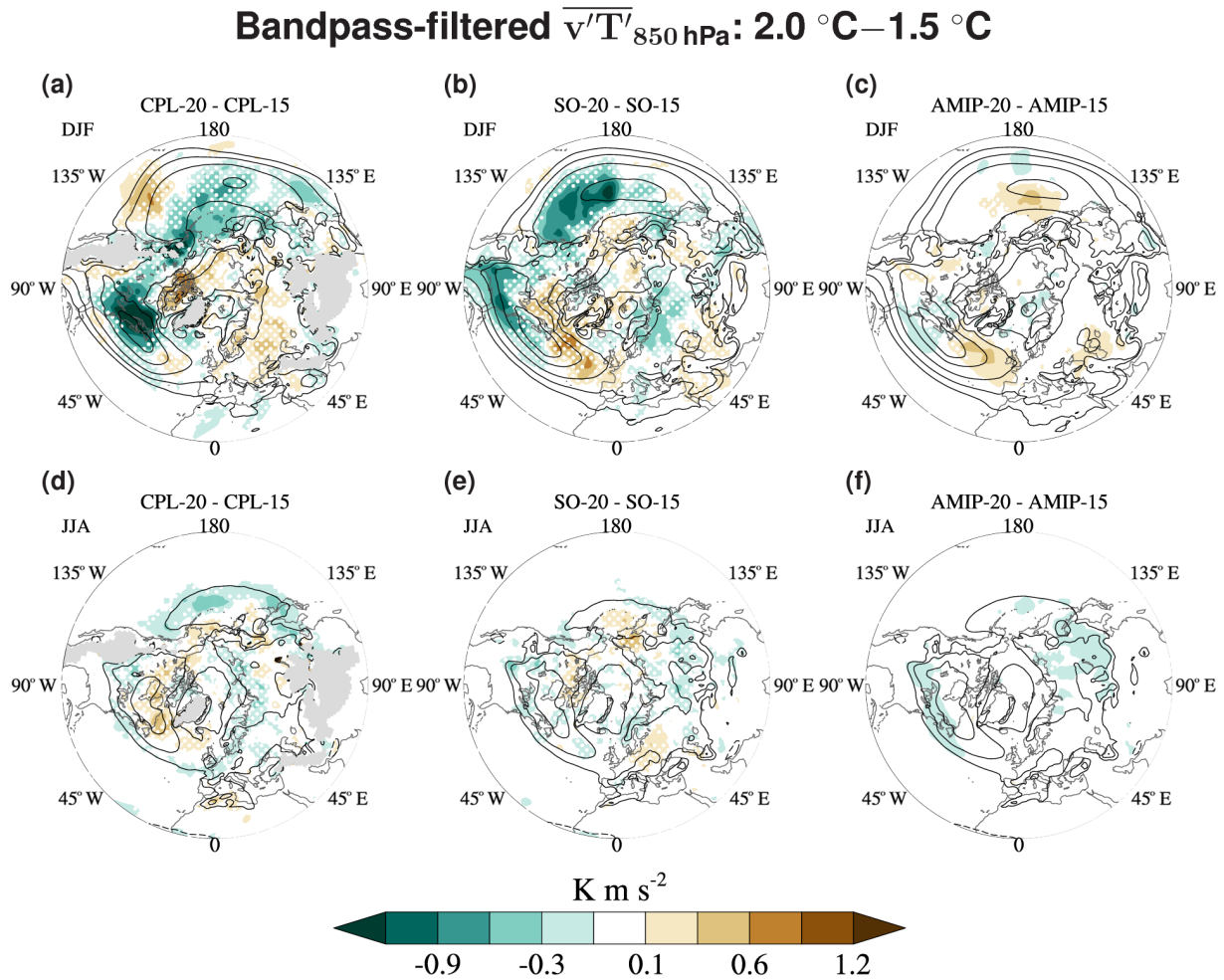
Figure 16. As in Fig. 15 but for the low-level storm-track response to the additional 0.5 °C warming (i.e. the difference between the 2.0 and 1.5 °C experiments).
