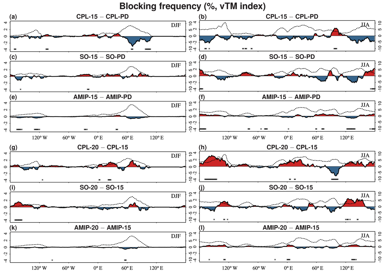
Figure 18. Change in blocking frequency (solid black line with red and blue shading) in the 1.5 °C experiment relative to PD (a–f) and for the additional 0.5 °C of warming (2.0–1.5 °C; g–l), shown along with the blocking climatology for the PD experiment (dotted black line). The fields are shown for NorESM1-Happi (a, b, g, h), NorESM1-HappiSO (c, d, i, j), and NorESM1-HappiAMIP (e, f, k, l) during DJF (a, c, e, g, i, k) and JJA (b, d, f, h, j, l) for the default periods given in Sect. 3. The asterisks along the x axis indicate where the changes at that longitude are statistically significant at the 5 % level according to the Welch t test. Note that the left y axis is for the difference field and the right y axis is for the climatology. Units are percentages (a–l).
