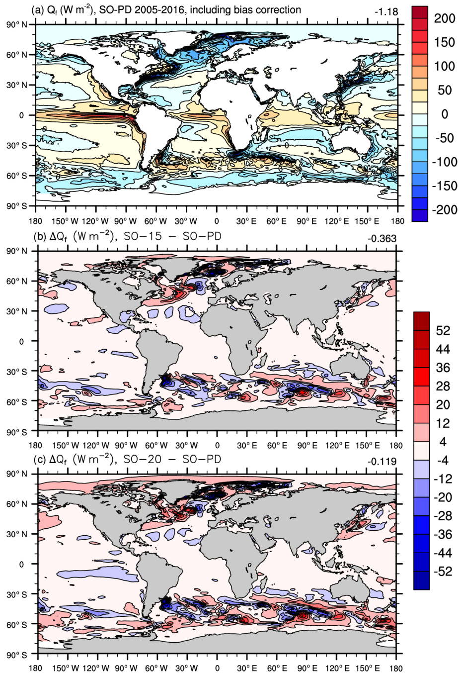
Figure 6. The annual-mean ocean heat flux ( Q_f ) needed in NorESM1-HappiSO to maintain a stable PD climate that is close to the observed SST used during calibration (a), and the change in Q_f for SO-15 (b) and SO-20 (c) compared to SO-PD. Negative values contribute to increasing SST (Eq. 1). Units are in \text{W m}^{-2} (a–c).
