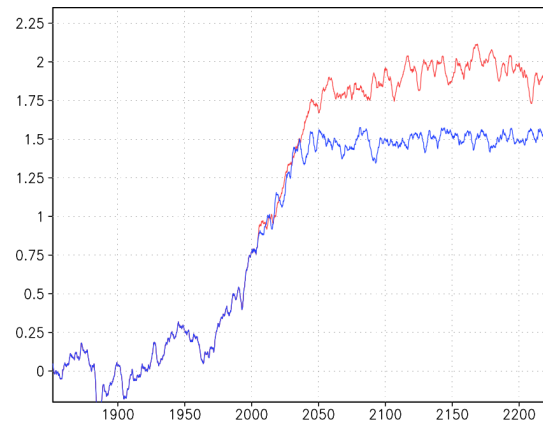
Figure 2. Time evolution of the global-mean near-surface temperature response in the Hist1 experiment (1850–2005; blue) and the CPL-15 (2006–2230; blue) and the CPL-20 experiments (2006–2230; red) relative to pre-industrial conditions (years 1850–1852). A 3-year running average is used for both curves. Units are in degrees Celsius.
