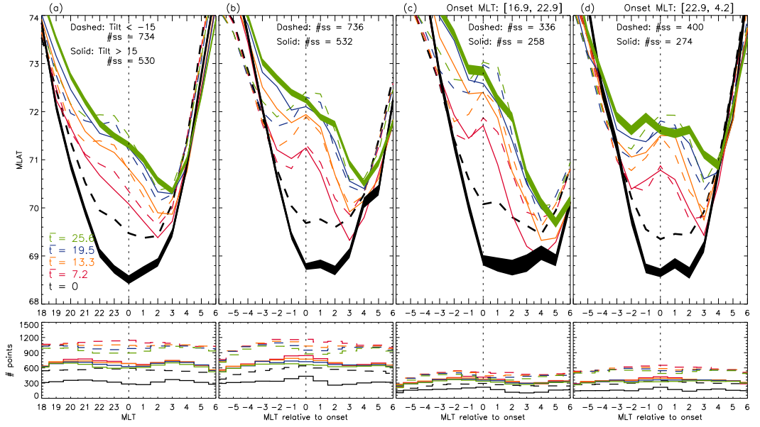
Figure 2. The figure shows average OCBs for substorms with onsets during periods when the dipole tilt angle was greater than 15^\circ (solid) and less than -15^\circ (dashed). The format is the same as in Figure 1. The format is also explained in Section 3.1. #ss denotes number of substorms in each bin.
