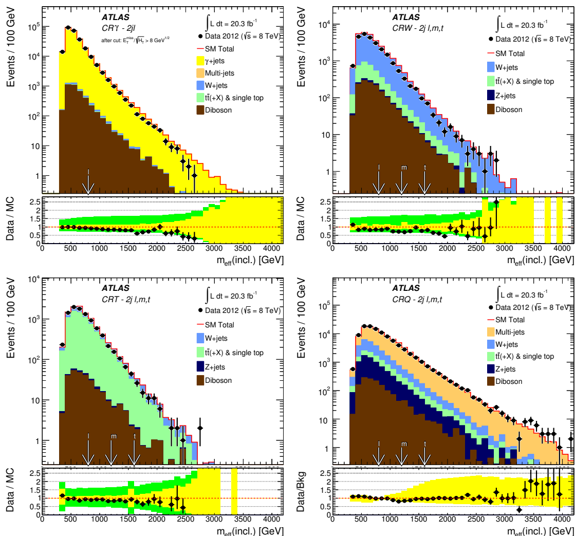
Figure 1. Observed m_{\text{eff}}(\text{incl.}) distributions in control regions \text{CR}\gamma (top left, for SR 2j selection criteria only), \text{CRW} (top right), \text{CRT} (bottom left) and \text{CRQ} (bottom right, excluding requirements on E_T^{\text{miss}}/\sqrt{H_T} ) corresponding to SRs 2jl, 2jm and 2jt. With the exception of the multi-jet background (which is estimated using the data-driven technique described in the text), the histograms denote the MC background expectations, normalised to cross-section times integrated luminosity. In the lower panels the light (yellow) error bands denote the experimental systematic and MC statistical uncertainties, while the medium dark (green) bands include also the theoretical modelling uncertainty. The arrows indicate the values at which the requirements on m_{\text{eff}}(\text{incl.}) are applied.
