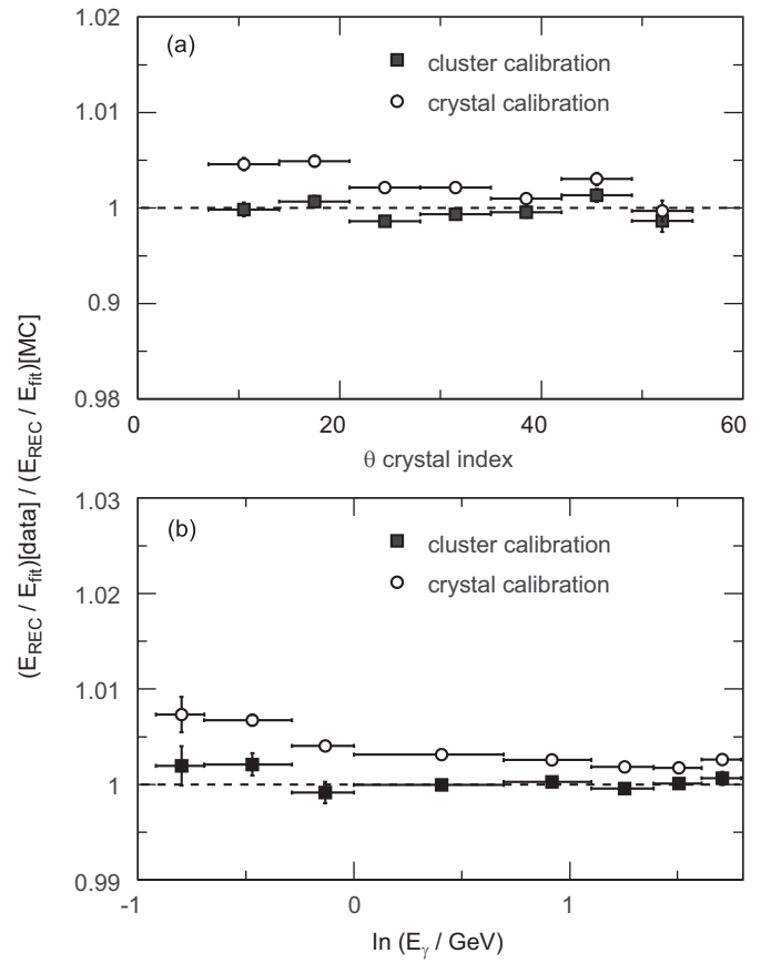
Fig. 66. EMC: Comparison of two photon calibration procedures based on selected \mu^+\mu^-\gamma events. Data/MC ratio E_{\text{REC}}^{\text{data}}/E_{\text{FIT}}^{\text{MC}} as a function of (a) the polar angle (crystal index) and (b) the photon energy (2006 data).
