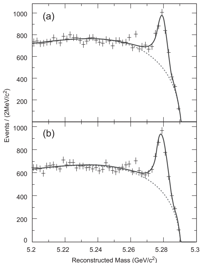
Fig. 81. Reconstructed mass of hadronic B meson candidates, for (a) tracks from the first pass reconstruction, and (b) after the implementation of track refinement and selection. The solid line represents the fit to the total distribution, the dashed lines describe the background.
