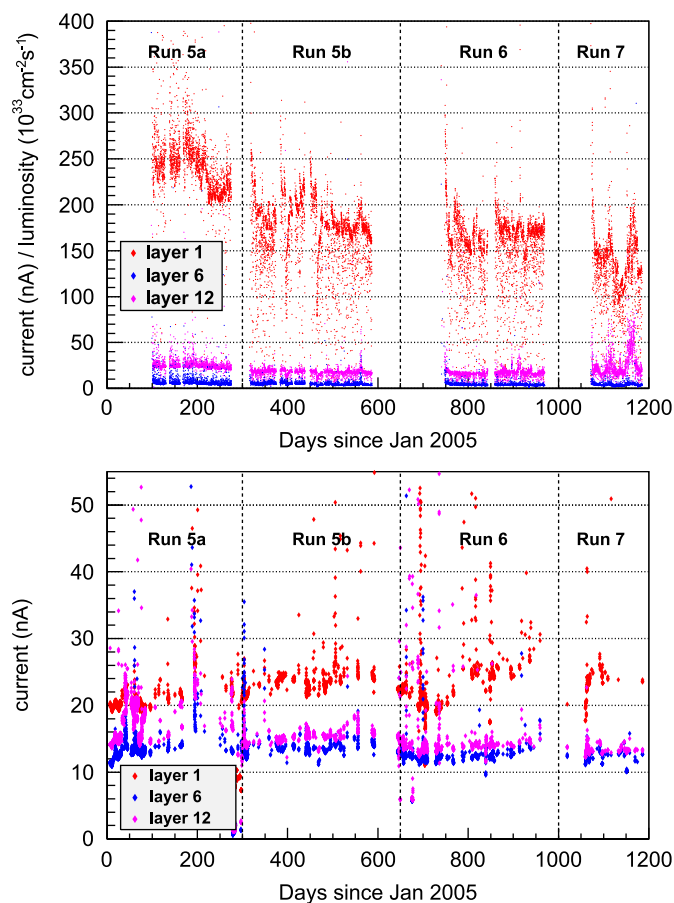
Fig. 73. Average LST currents as a function of calendar time: (top) Ratio of the average currents to the PEP-II luminosity recorded during colliding beams and (bottom) currents drawn for cosmic ray data recorded without beams.
