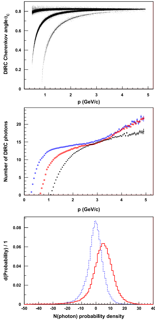
Fig. 88. (top) DIRC ring fit \theta_c vs p_{\text{lab}} for \pi (upper band), K (middle band), protons (lower band); (middle) mean number of DIRC signal photons vs p_{\text{lab}} for K (red), \pi (blue) and protons (black); (bottom) probability density function of the difference between the measured and expected numbers of DIRC signal photons. The plot is drawn for true K (solid red) and \pi (dashed blue) particles, with 0.9 < p < 1.0 GeV/c and assuming the K hypothesis.
