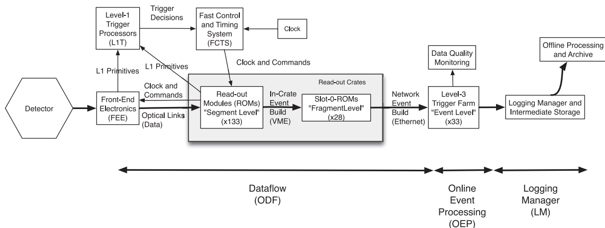
Fig. 24. Schematic diagram of the dataflow in the data acquisition chain.
