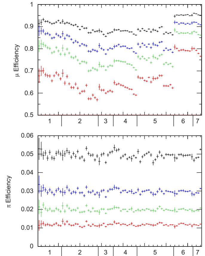
Fig. 76. Performance of muon identification based on BDT algorithms: muon identification efficiency (top) and pion misidentification (bottom) for selected charged tracks in the momentum range of 1.5–2.0 GeV/c as a function of calendar time, expressed in terms of Runs 1–7. The four data series marked in different colors correspond to four constant levels (1.2%, 2%, 3%, and 5%) of the average pion misidentification rates and indicate their correlation with the muon efficiencies. The data are integrated over the full fiducial volume.
