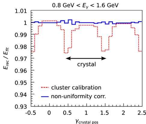
Fig. 84. Normalized response E_{rec}/E_{fit} across three CsI(Tl) crystals before (dashed, red) and after (solid, blue) the lateral non-uniformity correction.
