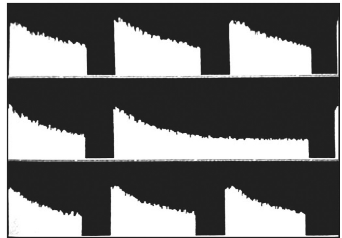
Fig. 5. PEP-II: oscilloscope record of bunch trains. The online luminosity per bunch (vertical axis) for 830 stored bunches (horizontal axis) on three consecutive traces from top left to bottom right. There are eight bunch trains, separated by gaps that are much larger than the 8.4 ns separation between consecutive bunches.
