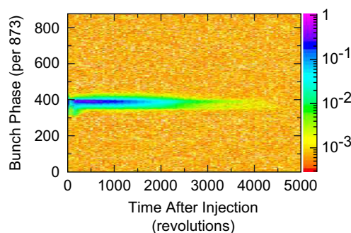
Fig. 6. PEP-II trickle injection background: EMC single cluster trigger rate per 420 ns (color coded as shown on the right) as a function of the bunch phase (873 clock ticks per revolution) for the first 5000 revolutions (36.7 ms) after the injection into the LER. Note that 420 ns correspond to 50 clock ticks.
