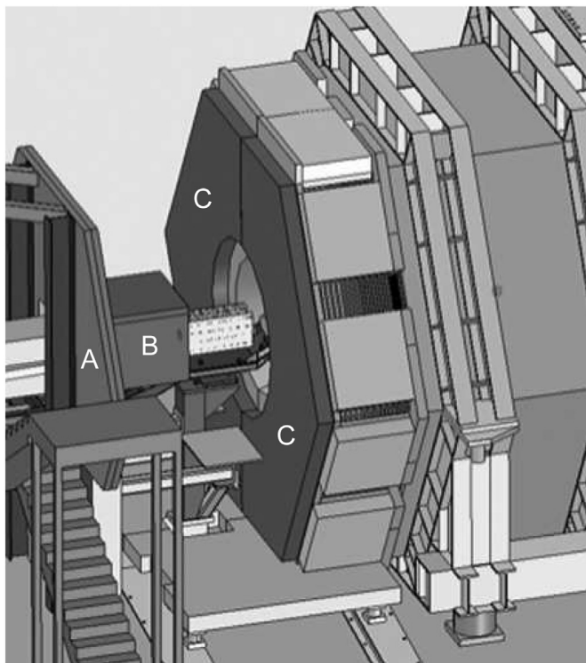
Fig. 16. IFR forward endcap shielding: (A) wall covering the tunnel exit and (B) extension around the beam line components built to protect the outer RPC layers of the upgraded endcap (C) from beam-generated background.
