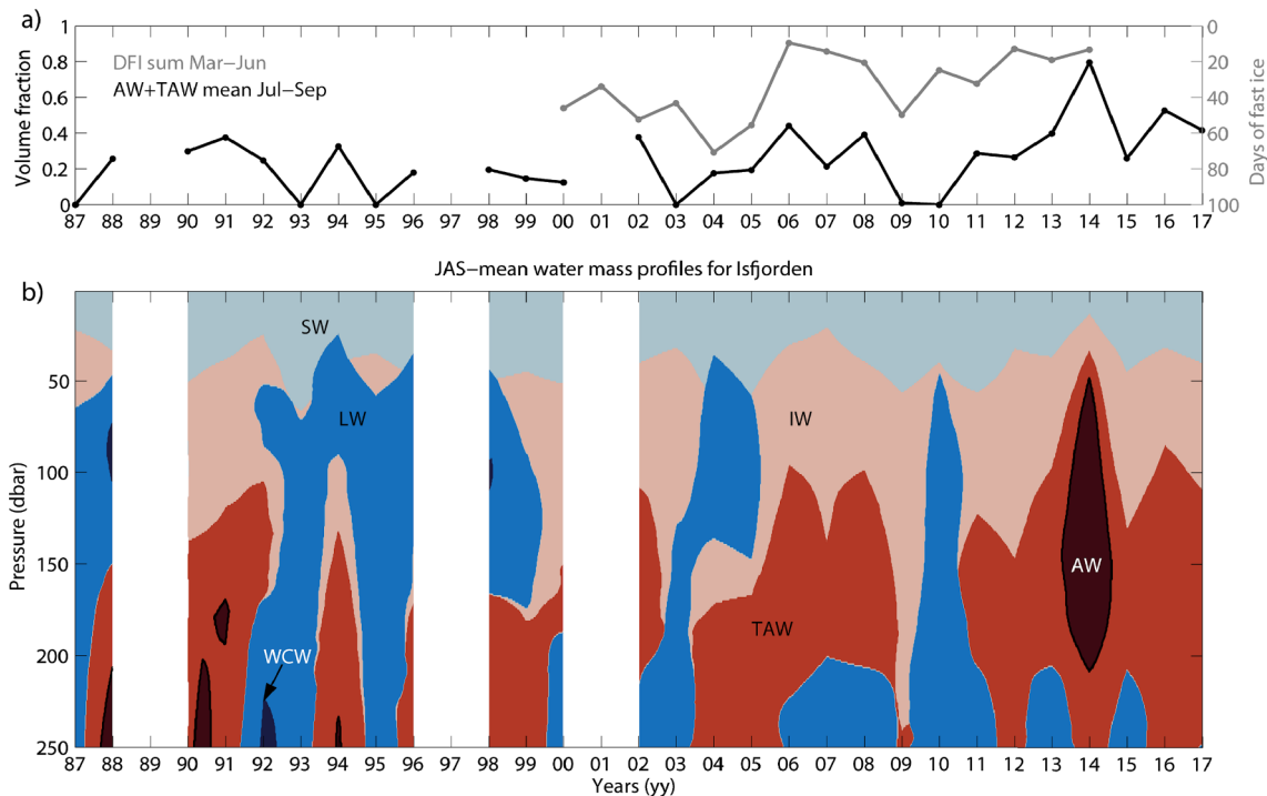
Fig. 4. Time series of annual (a) Atlantic Water (AW) and Transformed Atlantic Water (TAW) volume fraction (black line) and days of fast ice in Isfjorden (DFI, grey line), and (b) water mass distribution from the mean summer temperature and salinity profiles reaching deeper than 100 m inside Isfjorden proper (see Fig. 1) during the time period 1987 to 2017. The water masses indicated are listed in Table 1. Notice the reversed axis of DFI in (a).
