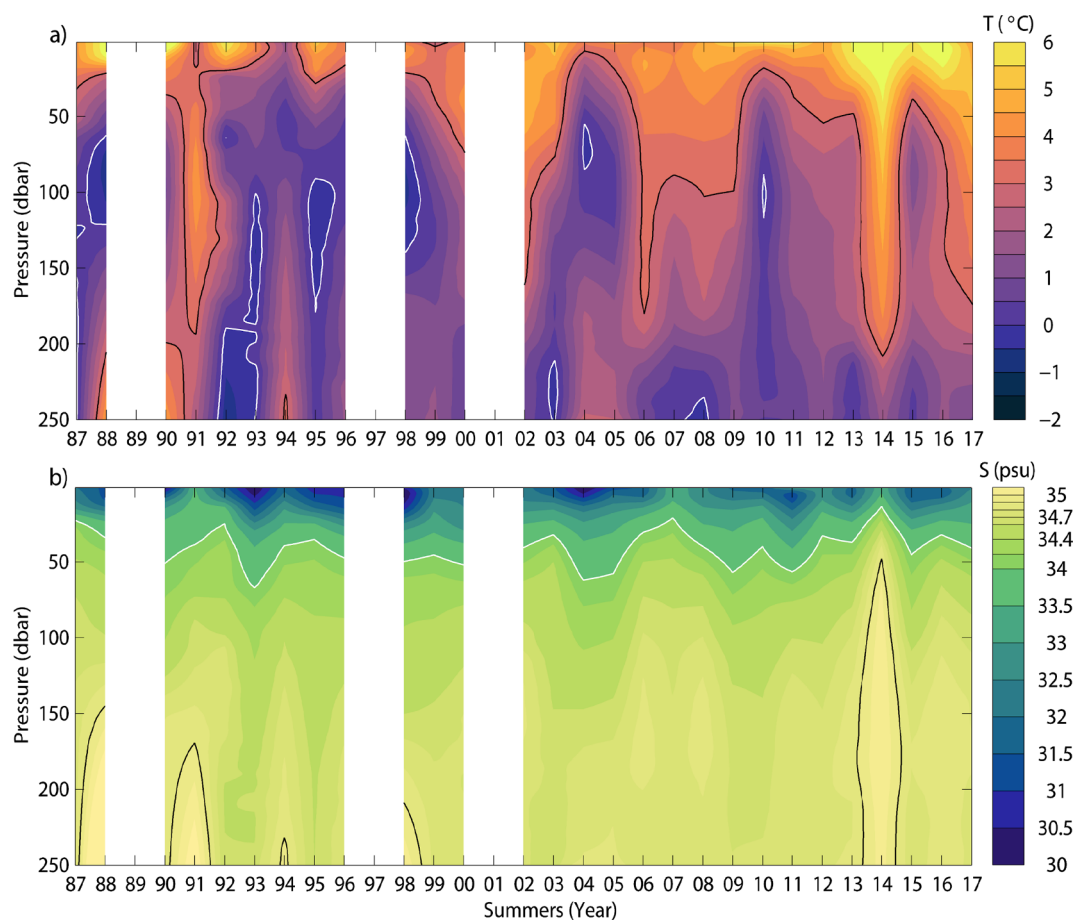
Fig. 2. Time series of mean summer (July–September) profiles of (a) temperature and (b) salinity based on profiles deeper than 100 m from Isfjorden proper during the time period 1987 to 2017. The black (white) lines indicate the 3 °C (0 °C) isothermal and the 34.9 (34) isohaline.
