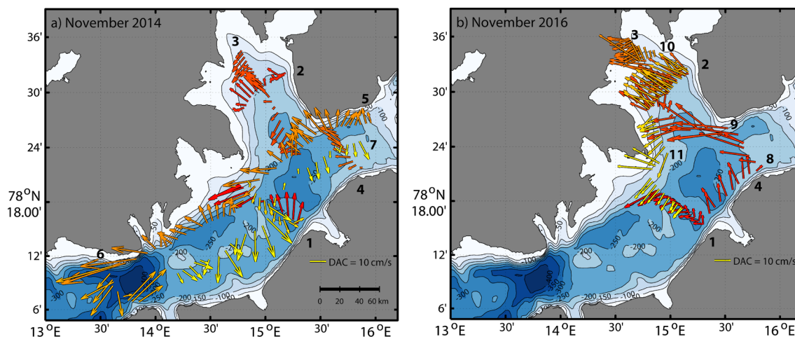
Fig. 17. De-tided depth-averaged currents (DACs) estimated during glider sections in Isfjorden in (a) November 2014 and (b) November 2016. Red (yellow) arrows are based on the earliest (latest) DAC data in each glider campaign. The numbered glider sections are indicated (see Table S5 in Supplementary data). The scale of the DACs is indicated in the lower right corner of the panels.
