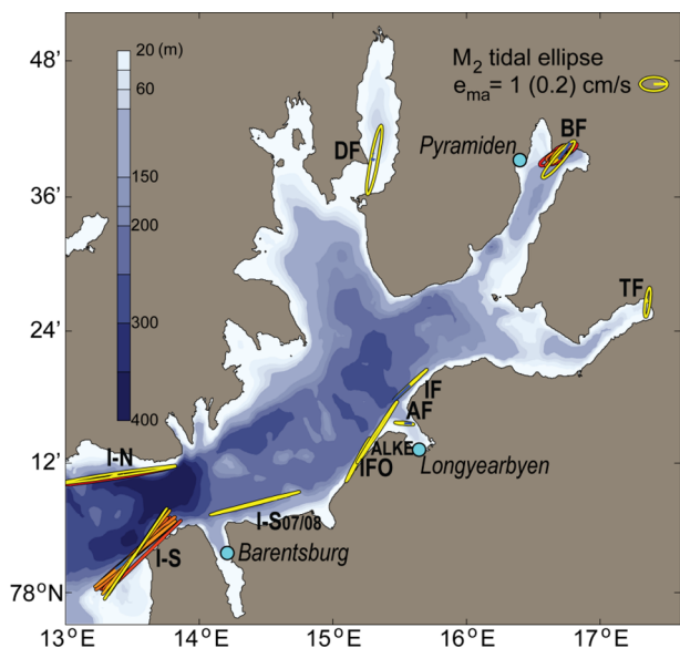
Fig. 19. The M2 tidal ellipse from the different mooring locations in Isfjorden estimated over their respective measuring periods. At locations with several yearlong records, red (yellow) ellipses are based on the oldest (most recent) depth-averaged current time series. The scale of the tidal ellipses is indicated in the top right corner (the scale for BF and TF is given in the parentheses).
