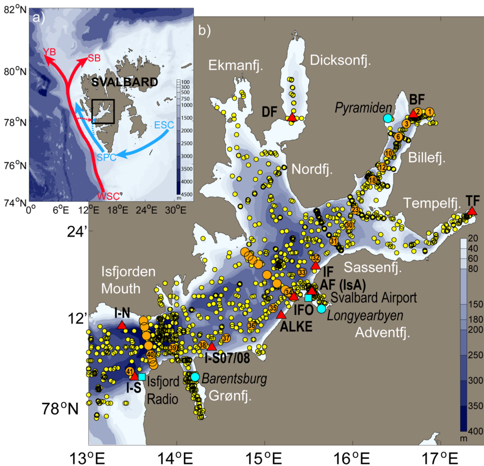
Fig. 1. (a) The ocean bathymetry around Svalbard Archipelago with the two main currents; West Spitsbergen Current (WSC) and East Spitsbergen Current (ESC) drawn with red and blue arrows, respectively. WSC separates into two branches; the Svalbard Branch (SB) and the Yermak Branch (YB). ESC continues as Spitsbergen Polar Current (SPC) west of Svalbard. The red and blue stippled arrows indicate inflow from WSC and SPC, respectively. The black box outlines the area covered in (b), which shows the bathymetry of the Isfjorden system with its side fjords. The numbered orange dots indicate the Isfjorden Transect (see Table 2) from the head of Billefjorden (Station 1) to the Isfjorden Mouth (Station 41) as well as the cross sections (not numbered) at the mouth and in Isfjorden proper. The positions of CTD profiles obtained from UNIS hydrographic database (UNIS HD) are shown with smaller yellow dots. The red triangles show the location of the moorings listed in Table 3, and the Isfjorden-Adventfjorden sampling station (IsA). The cyan squares show the location of the meteorological stations at Isfjord Radio and Svalbard Airport. The settlements: Barentsburg, Longyearbyen, and Pyramiden are indicated with cyan dots. The bathymetry is from the International Bathymetric Chart of the Arctic Ocean (IBCAO) version 3.0 (Jakobsson et al., 2012).
