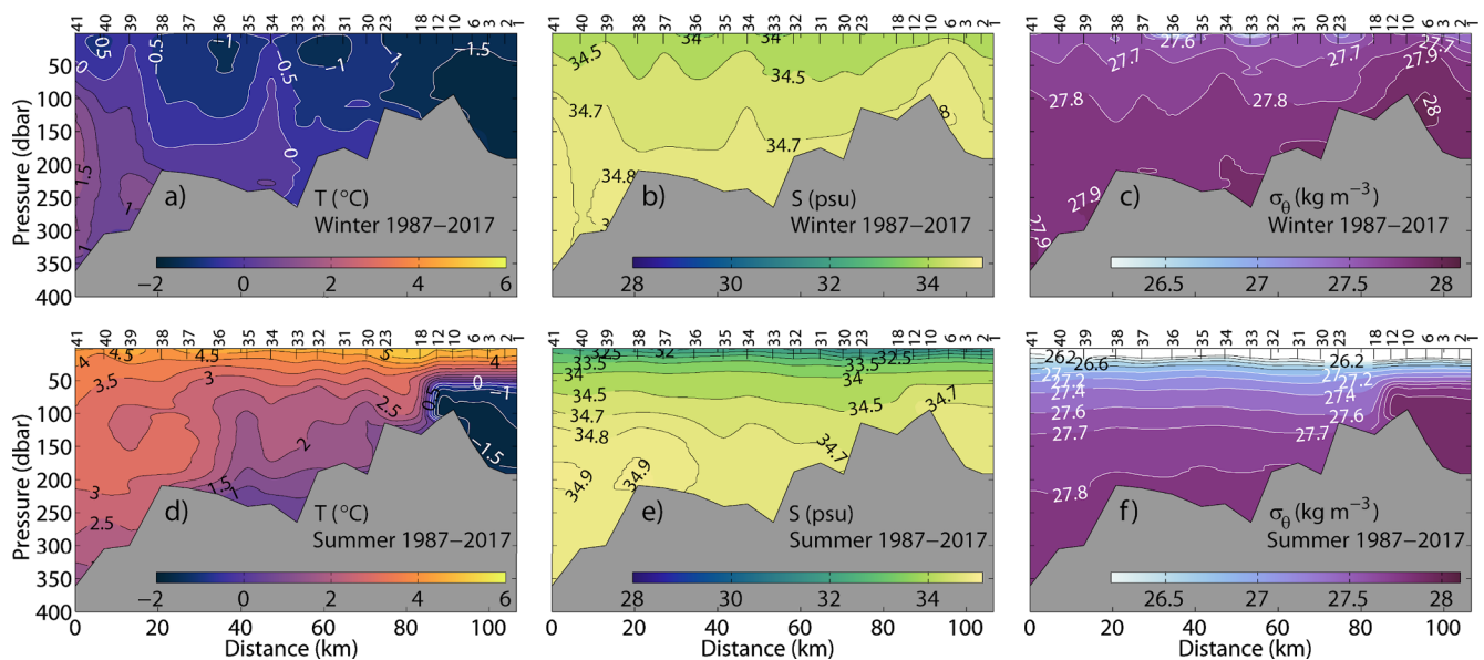
Fig. 6. Distribution of mean (a) and (d) temperature, (b) and (e) salinity, and (c) and (f) density along the Isfjorden Transect from the mouth area (Station 41) to the head of Billefjorden (Station 1) over all available years in the time period 1987–2017 for (a) to (c) the winter months (Jan–May) and (d) to (f) the summer months (Jul–Sep).
