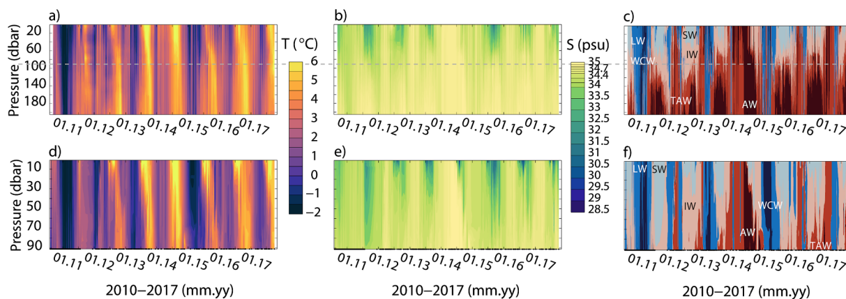
Fig. 13. Time series of vertical distribution of (a) & (d) temperature, (b) & (e) salinity, and (c) & (f) water masses based on (a) - (c) data from mooring I-S and (d) - (f) combined data from mooring ALKE (Sept. 2010 - Sept. 2011) and CTD profiles at IsA (Dec. 2011 - Oct. 2017). The grey dashed line indicates the 90 m depth at I-S for comparison with IsA. The sampling dates at IsA are indicated with black dots on the time axis. The water masses are listed in Table 1. For locations see Fig. 1b.
