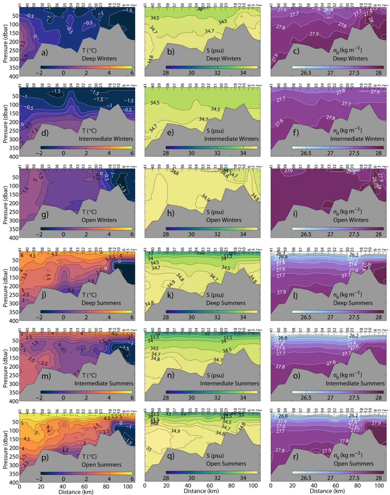
Fig. 7. Distribution of mean (a)–(p) temperature, (b)–(q) salinity, and (c)–(r) density along the Isfjorden Transect from the mouth area (Station 41) to the head of Billefjorden (Station 1) over Winter (a)–(c) Deep, (d)–(f) Intermediate, and (g)–(i) Open, and over (j)–(r) corresponding following summers.
