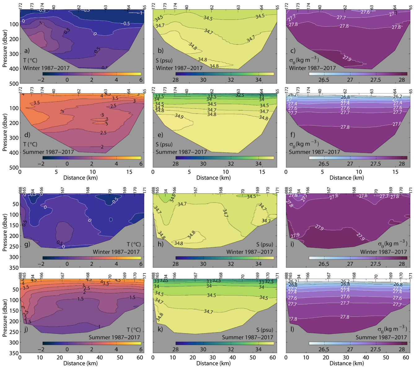
Fig. 11. Distribution of mean (a)–(f) temperature, (b)–(k) salinity and (c)–(l) density across (a)–(f) the mouth from south (Station 172) to north (Station 65) and (g)–(l) Isfjorden proper from south (Station 988) to north (Station 171) over (a)–(c) and (g)–(i) winters and (d)–(f) and (j)–(l) summers during the time period 1987 to 2017. For section locations see Fig. 1b.
