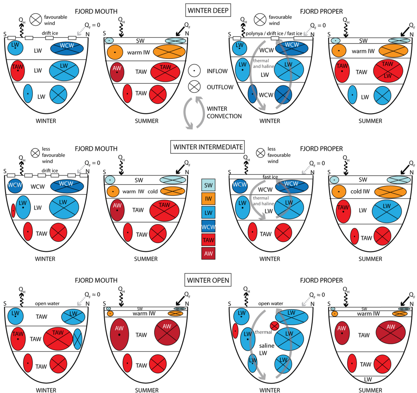
Fig. 21. A conceptual drawing of the fjord’s response in winter and summer hydrography (layering and water masses) and circulation (in- and outflow) to the three different winter convection types; Winter Deep (deep thermal and haline convection), Winter Intermediate (intermediate thermal and haline convection), and Winter Open (open water with only thermal convection) valid for broad Arctic fjords facing potential inflow of warm water of Atlantic origin (TAW and AW). Cross sections at the fjord mouth are shown to the left and those in the fjord proper to the right, where S is the southern (inflow) side and N is the northern (outflow) side. Colours indicate the water masses defined for the Isfjorden system (see Table 1). Q_H is heat flux, Q_F is freshwater flux, and the white blocks on the surface in winter indicate drift ice and fast ice cover. Favourable wind means strong wind with direction favouring out-fjord transport of sea ice (Nilsen et al., 2008a).
