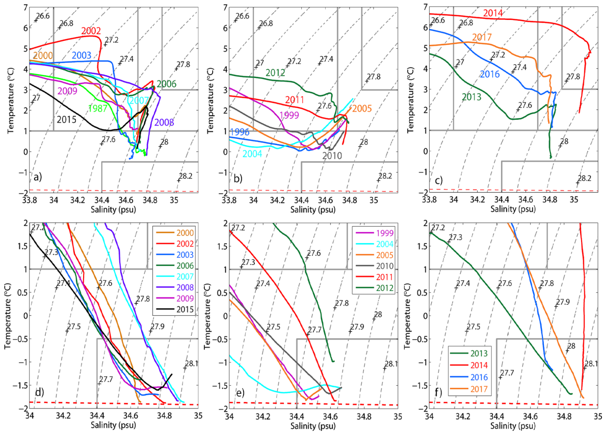
Fig. 9. Temperature and salinity diagrams with (a)–(c) the mean summer profiles reaching deeper than 100 m inside Isfjorden proper (around Stations 34 and 35) and (d)–(f) the summer profiles in the deepest part of Billefjorden (around Station 3) grouped into summers after winter of type (a) and (d) deep, (b) and (e) intermediate, and (c) and (f) open. Notice the different axis range in (a)–(c) and (d)–(f).
