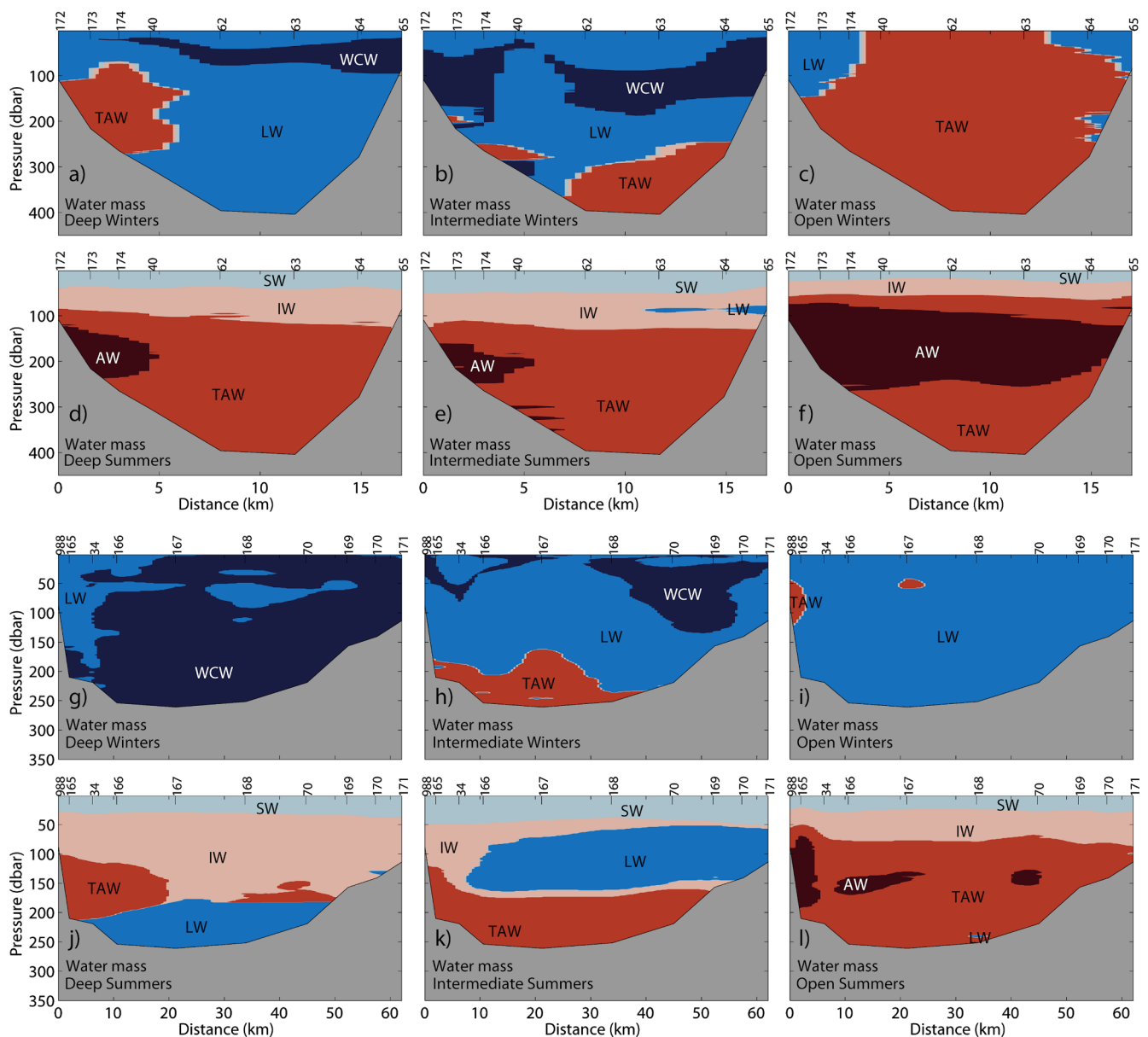
Fig. 12. Cross-fjord distribution of mean water masses over (a)–(c) and (g)–(i) winters and (d)–(f) and (j)–(l) summers after Winter (a)–(j) Deep, (b)–(k) Intermediate, and (c)–(l) Open at (a)–(f) the mouth from the south (Station 172) to the north (Station 65), and the section (g)–(l) in Isfjorden proper from the south (Station 988) to the north (Station 171). The water masses are given in Table 1, and the section locations are shown in Fig. 1b.
