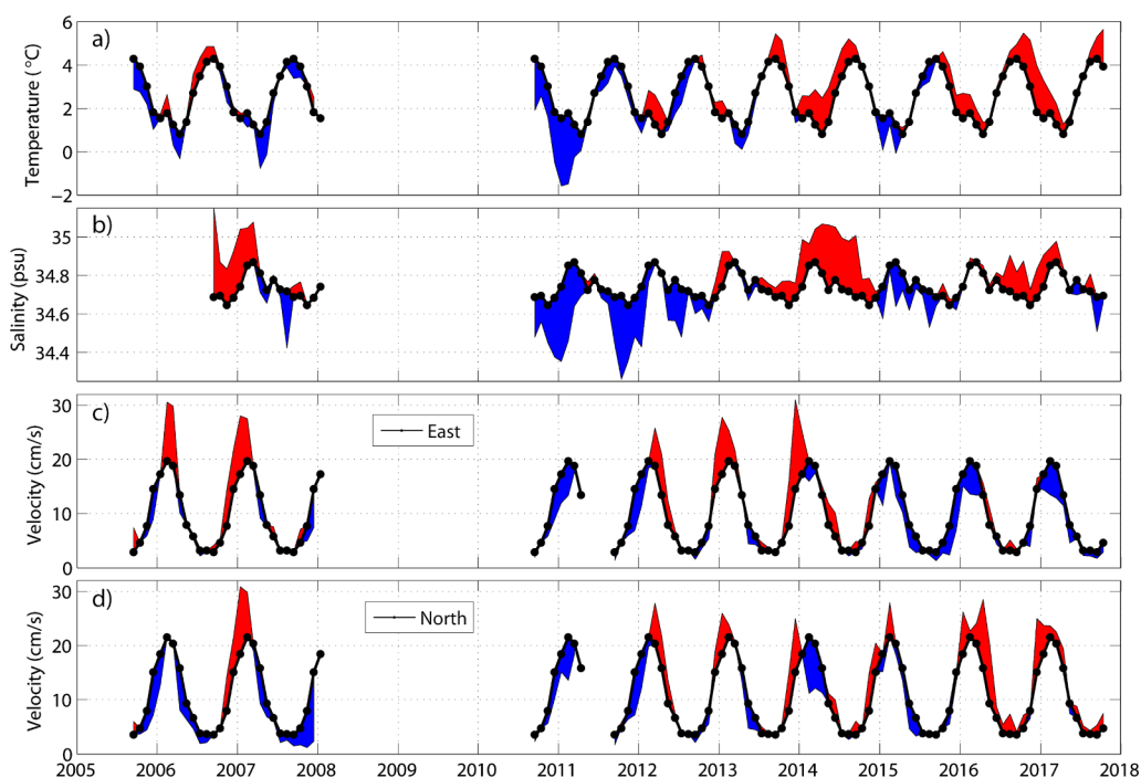
Fig. 15. Deviation from the monthly depth-averaged climatology (black dots and line) of (a) temperature, (b) salinity, (c) east- and (d) north velocity component from the I-S mooring time series. Red (blue) is (a) warmer (colder), (b) more (less) saline, (c) and (d) stronger (weaker) velocity component than the monthly climatology, which is based on the existing time series during the period from 2005 to 2017.
