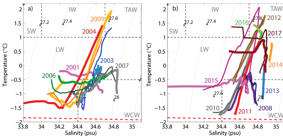
Fig. 5. Temperature and salinity diagrams with the mean winter profiles from an area around Stations 38 and 39 at the entrance (thin solid line with darker colour tone) and Stations 34 and 35 in Isfjorden proper (thick solid line with lighter colour tone) for (a) winter 2001 to 2007 and (b) winter 2008 to 2017. No profiles were available at the entrance in 2001, 2004, 2011, 2013, and 2014. Water masses are indicated by the grey dotted lines, and the freezing point temperature is given by the red dotted line.
