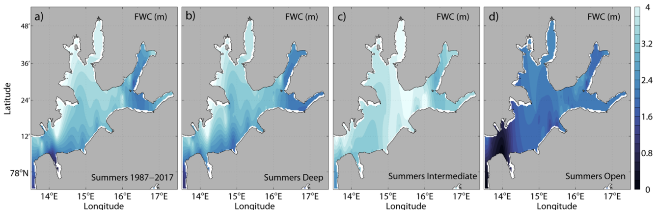
Fig. 10. Horizontal distribution of mean full-depth freshwater content (FWC) in meters from salinity profiles over summers (a) in the time period 1987 to 2017, and after Winter (b) Deep, (c) Intermediate, and (d) Open.
