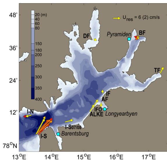
Fig. 16. The mean residual current from different mooring locations in Isfjorden estimated over their respective measuring periods. At locations with several yearlong records, red (yellow) arrows are based on the oldest (most recent) depth-averaged current (DAC) time series. The scale of the mean residual current is indicated in the top right corner (the scale for IF, BF, and TF is given in the parentheses).
