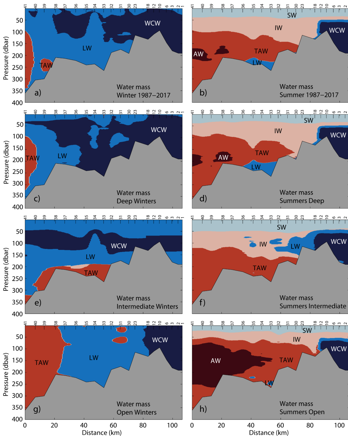
Fig. 8. Distribution of mean water masses over (a)–(g) winters and (b)–(h) summers during (a)–(b) the time period 1987 to 2017, and of Winter (c)–(d) Deep, (e)–(f) Intermediate, and (g)–(h) Open along the Isfjorden Transect from the mouth area (Station 41) to the head of Billefjorden (Station 1). The water masses indicated are listed in Table 1.
