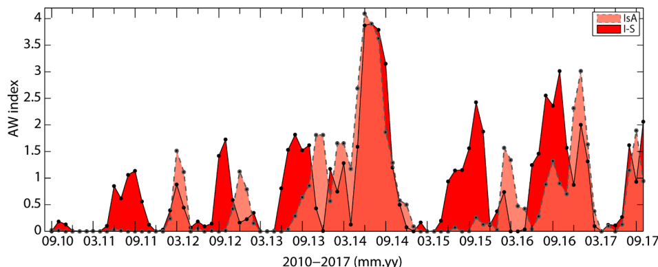
Fig. 14. Monthly AW indexes at I-S (red) and IsA (pink transparent) during the time period September 2010 to October 2017. The AW indexes are based on presence of AW at I-S and also TAW at IsA. See Fig. 1b for locations.
