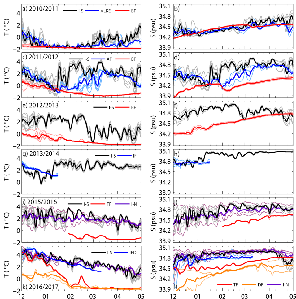
Fig. 20. 72-hrs smoothed temperature (left) and salinity (right) time series from the moorings in the Isfjorden system (see Fig. 1b and Table 3), showing only the time period from December to May in (a)–(b) 2010/2011, (c)–(d) 2011/2012, (e)–(f) 2012/2013, (g)–(h) 2013/2014, (i)–(j) 2015/2016, and (k)–(l) 2016/2017. The thick lines show the depth-averaged time series, and the thin lines with corresponding lighter colour tones show the time series from each measured depth (see Tables S3 and S4 in Supplementary data).
