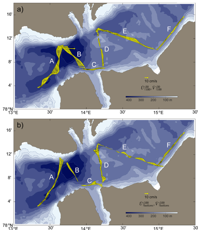
Fig. 18. De-tided depth-averaged currents (DACs) over (a) 30–100 m depth and (b) 100 m depth to bottom, estimated along VM-ADCP sections in the Isfjorden mouth and proper on 29 July 2007. The scale of the DACs is indicated in the lower right corner of the panels.
