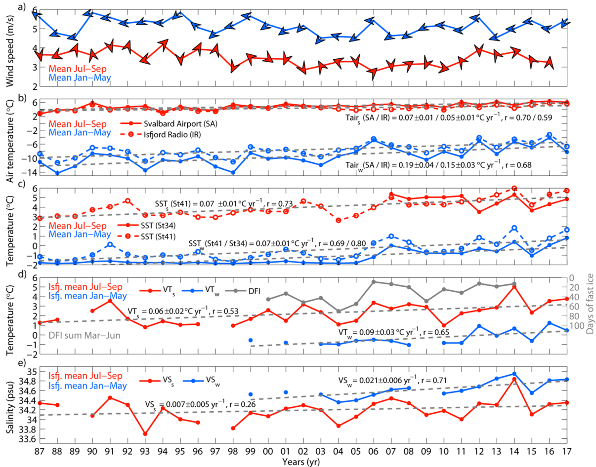
Fig. 3. Annual mean winter (blue) and summer (red) time series of (a) 10 m wind speed and direction (arrows) from averaged NOR10 data points over Isfjorden proper, (b) 2 m air temperature at Svalbard Airport (solid line) and Isfjord Radio (stippled line), and (c) OSTIA sea surface temperature in Isfjorden ( SST_{St34} ) and at the mouth ( SST_{St41} ) during 1987 to 2017. Annual volume weighted mean (d) temperature (VT) and (e) salinity (VS) from summer (red) and winter (blue) CTD profiles deeper than 100 m from Isfjorden proper for the same period as in (a) to (c). Also shown in (d) are days of fast ice (DFI) in Isfjorden from March to June each year from 2000 to 2014 (grey line, reversed axis). Winter (w) and summer (s) trends (per year) are indicated by the grey stippled lines, with the slope values ( \pm errors) and correlation coefficients ( r ) given in the corresponding panels.
