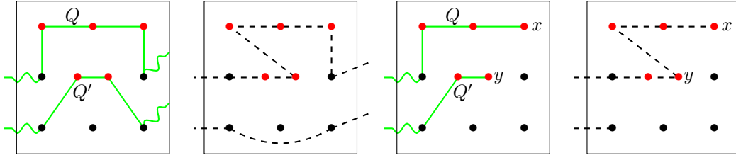
■ Figure 6 The proof of Lemma 13. Vertices colored black and red are the marked and unmarked vertices in the cell, respectively. In the first figure the union of internal vertices of Q and Q' is the set of unmarked vertices in the cell, and the second figure depicts how to reroute to make the cell nice. The third figure illustrates the case when both the endpoints x and y of the path P are in the cell, and the fourth figure depicts how to reroute to make the cell nice.
