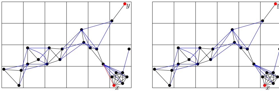
■ Figure 7 The graphs G' and G^* constructed from the graph G in Figure 1 are depicted on the left side and right side figures, respectively. Here, w(x) = 2 , w(y) = 3 , and for all z \in V(G') \setminus \{x, y\} , w(z) = 1 .
