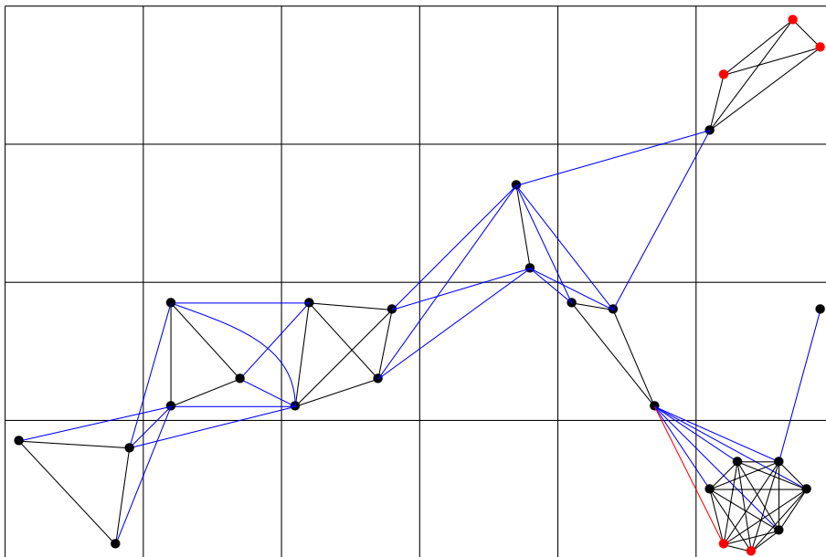
■ Figure 1 A clique-grid graph G . Marked vertices are colored black. Good and bad edges are colored blue and red, respectively (see Definition 8). For the sake of illustration only, we use the threshold 5 instead of 121 – that is, in phase II of marking let \text{Mark}_2(v, (i', j')) denote a set of 5 vertices in f^{-1}(i', j') that are adjacent to v in G , where if no 5 vertices with this property exist, then let \text{Mark}_2(v, (i', j')) denote the set of all vertices with this property.
