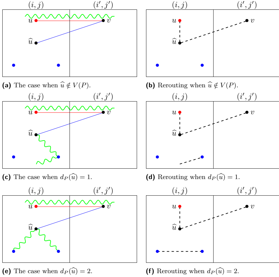
■ Figure 2 Case I in the proof of Lemma 9. Vertices colored black and red are marked and unmarked, respectively. Vertices colored blue are either marked or unmarked. Good and bad edges are colored blue and red, respectively. Curves colored green are part of the path P . Dashed lines are part of the path P_2 .
