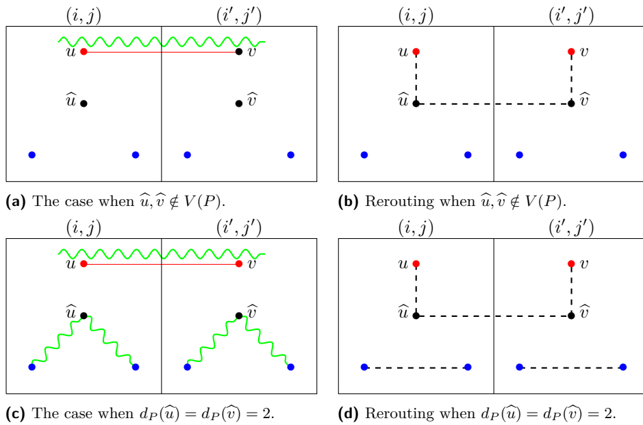
Figure 3 Two subcases of Case II in the proof of Lemma 9. Other subcases are handled similarly to the subcases depicted here. Vertices colored black and red are marked and unmarked, respectively. Vertices colored blue are either marked or unmarked. Good and bad edges are colored blue and red, respectively. Curves colored green are part of the path P . Dashed lines are part of the path P_2 .
