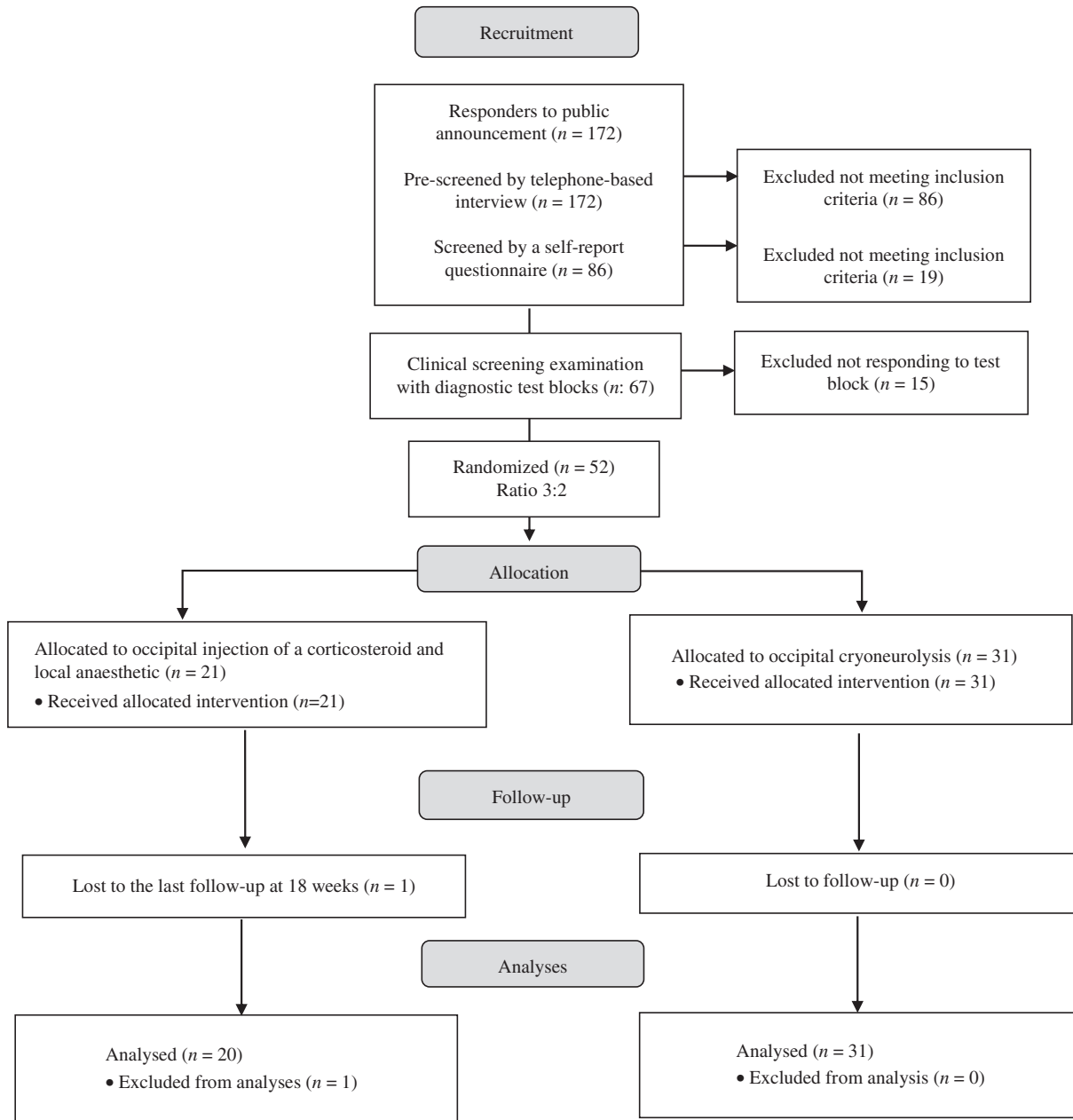
Fig. 1: Flow chart.
