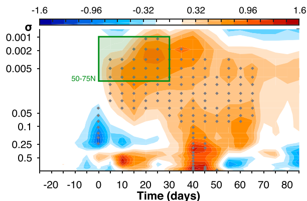
FIG. 10. Regression of polar cap ( 75^{\circ} – 90^{\circ} N) potential temperature response S on the earlier stratospheric zonal wind response in the green box ( \sigma = 10^{-3} – 10^{-2} , 50^{\circ} – 75^{\circ} N, days 1–30). Each symmetric response S_i is the anomaly from the control member C_i , so a possible dependence of downward propagation on the control simulation variability is not captured in this regression. Positive values indicate warmer potential temperature with a weakened polar vortex. Stippling shows points that are significantly different from zero (5% level).
