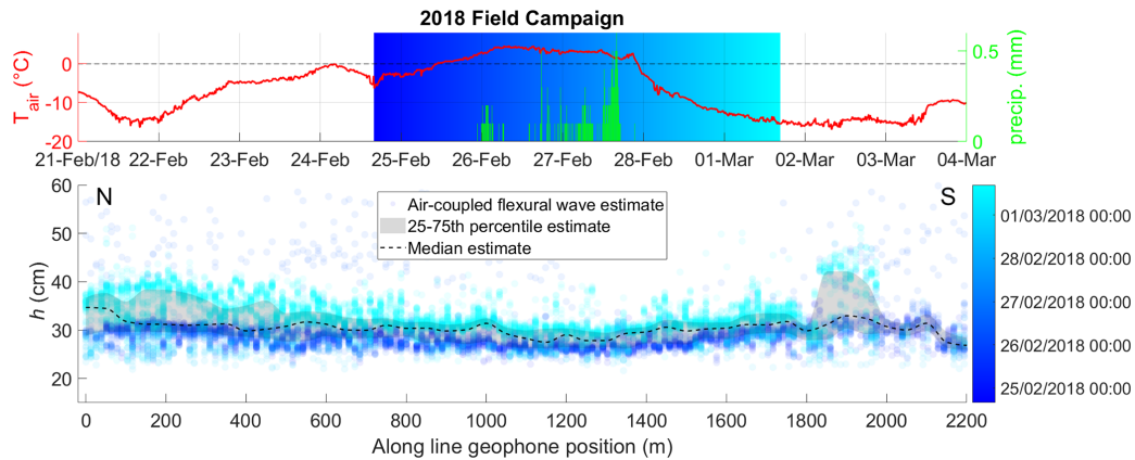
Figure 11. The 2018 field campaign air-coupled flexural wave ice thickness estimates (circles), temperature (red line) and precipitation (green bars) at Sveagruva weather station. Timing of experiments is indicated by blue–cyan colour gradient, and point estimates are transparent so overlapping repeat tests are indicated by denser colours. Figure 1 shows location of profile. Median is shown with a dashed line because there are two distinct, temporally separated populations.
