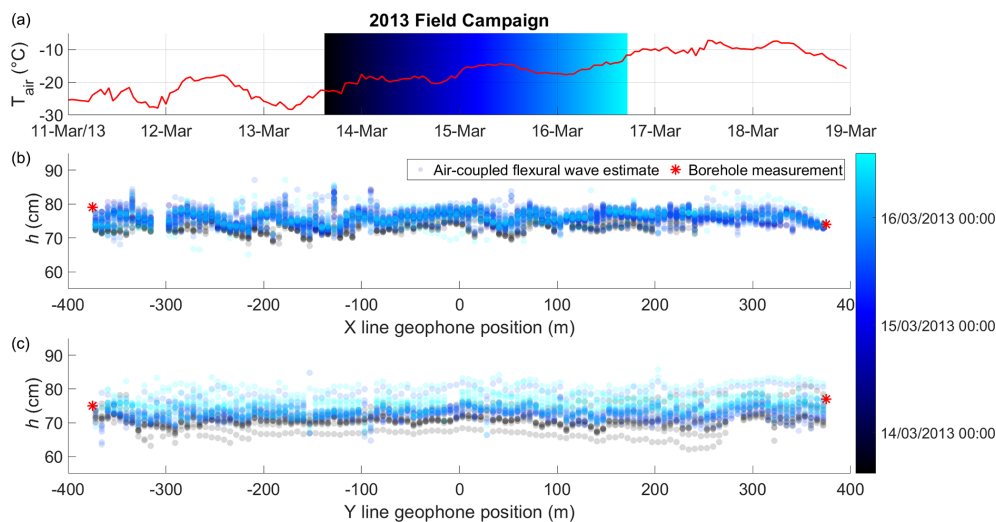
Figure 8. The 2013 field campaign air-coupled flexural wave ice thickness estimates (circles), borehole drilled thicknesses (red stars) and air temperature at nearby Sveagruga weather station (red line). The time span of the field campaign is indicated by black–blue–cyan colour gradient. Point estimates are transparent so overlapping repeat tests are indicated by denser colours. Figure 1 shows location of the profiles 2013 X (b) and 2013 Y (c).
