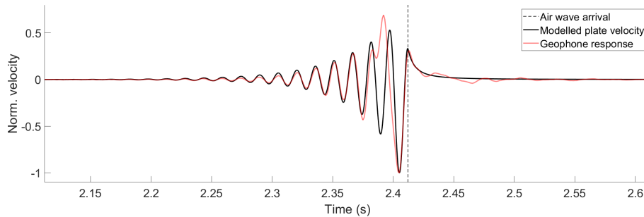
Figure 7. Modelled normalized velocity response time series (black curve) at an offset of 759 m compared with the time series recorded by a geophone at the same offset from a point charge fired during the 2013 field season (red curve). The air wave arrival time is indicated by the dashed line.
