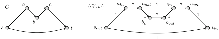
Fig. 10 Illustration of the transformation given in the proof of Theorem 4.9. Note that in this case, m = 6 , so the arcs between vertices v_{in} and v_{out} have weight 7
