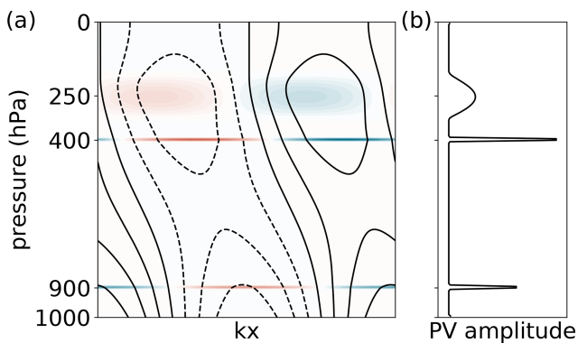
Figure 11. (a) Structure of interior PV (shading) and \psi (contours) for the most unstable mode of the default smooth experiment including latent heating and (b) amplitude of interior PV anomalies. Values are not comparable to physical values due to normalisation constraint mentioned in Sect. 2.1.
