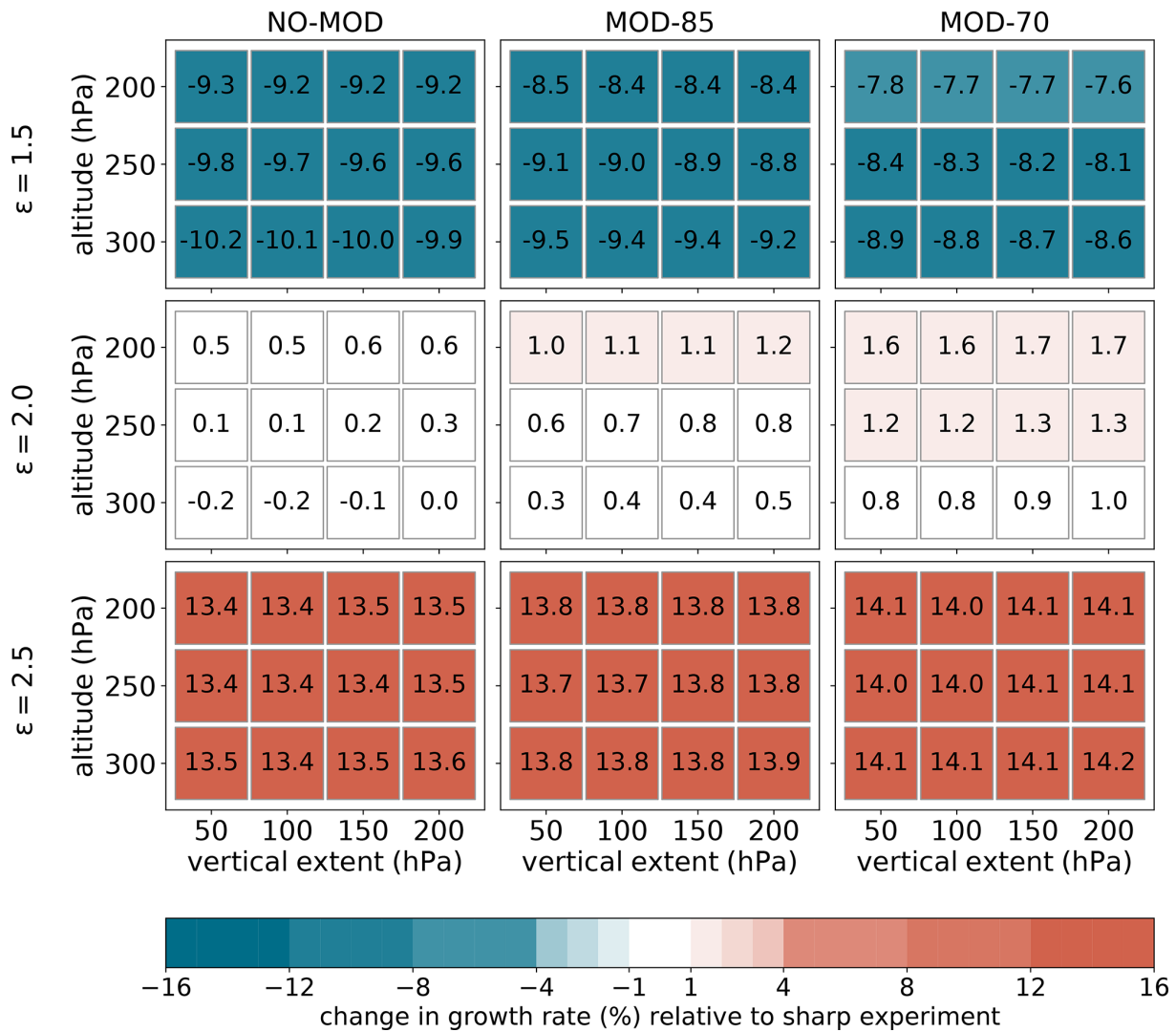
Figure 12. Same as Fig. 8 but including latent heating for three different heating intensity parameters ( \epsilon = 1.5, 2.0, 2.5 ). Note that the colour bar is extended from the one in Fig. 12 but contains the same colours at lower values.
