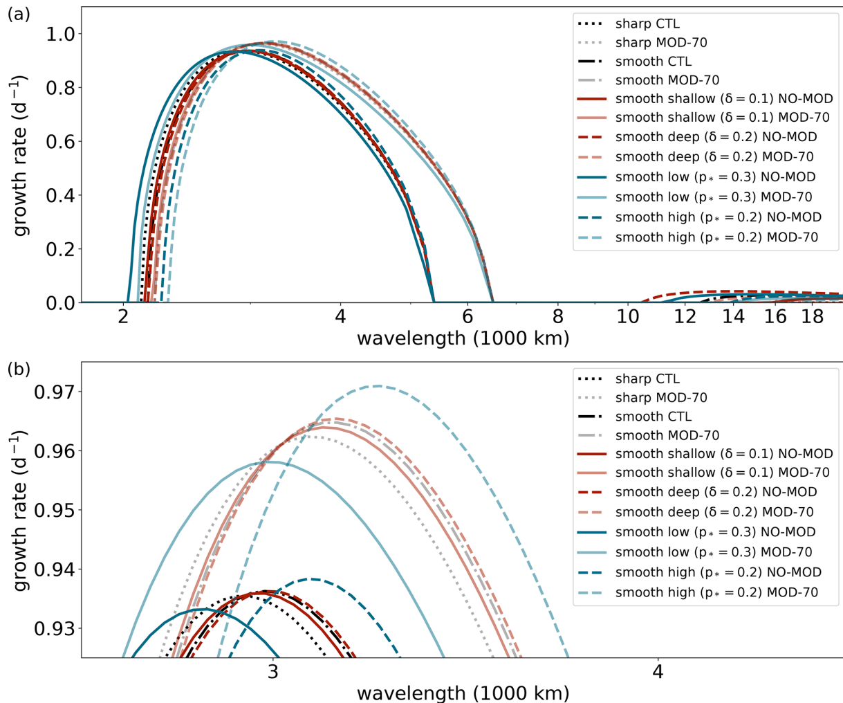
Figure 6. (a) Growth rate vs. wavelength for \lambda_{tr} = 3.5 , \lambda_{st} = -3.5 , S_{tr} = 1 , S_{st} = 4 , and various sensitivity experiments, with the default smooth experiment being associated with a tropopause region of 150 hPa depth centred at an altitude of 250 hPa. See text for further details. (b) Magnification of panel (a).
