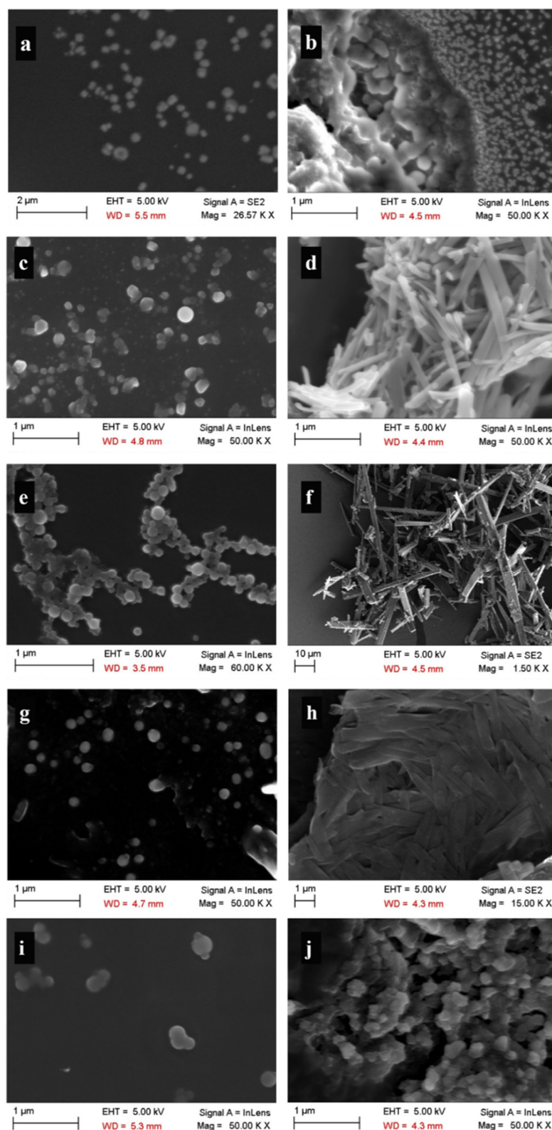
Figure 3. SEM images of particles of (a) AMIa, (b) AMIb, (c,d) COU, (e,f) CUR, (g,h) NOR, and (i,j) PRO generated by antisolvent precipitation method. (a,c,e,g,i) Solvent-evaporated particles. (b,d,f,h,j) Freeze-dried particles.
