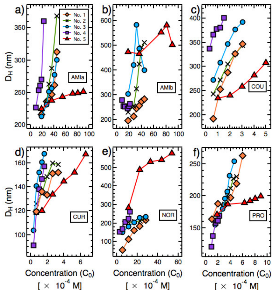
Figure 1. Mean particle size ( D_H ) of (a) AMIa, (b) AMIb, (c) COU, (d) CUR, (e) NOR, and (f) PRO with varying compound concentration in the solvent + antisolvent mixture solution ( C_0 ).
