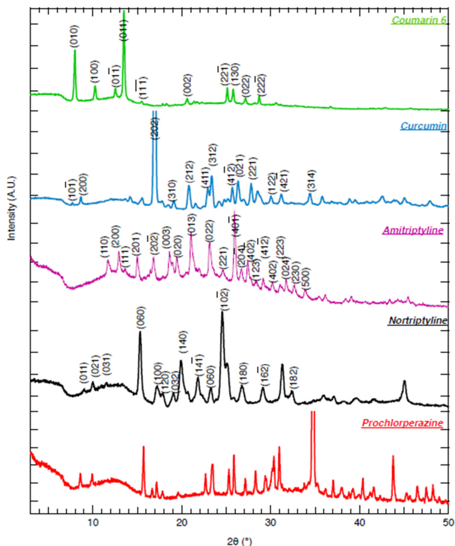
Figure 4. XRD data of freeze-dried samples of COU, CUR, AMI, NOR, and PRO particles. The XRD intensities are presented in logarithmic scales. The Miller indices of the main peaks are indicated for COU, CUR, AMI and NOR.
