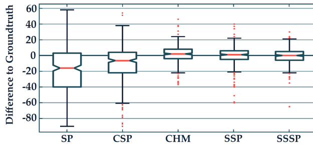
Figure A.10: Overview of the errors during the density value estimations for the assign task in all five visualization stimuli.
