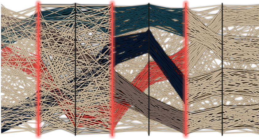
Figure 3.20: Visualization of a benchmark data set [17] consisting of four clusters: brown (50 lines), dark blue (49 lines), turquoise (48 lines), red (46 lines), and beige noise (150 lines).
