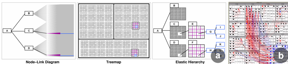
Figure 2.7: Graph and network examples using treemaps: (a) Elastic Hierarchy [189] combining node-link diagrams interactively with standard treemaps, and (b) Overlaid Graph Links [60] exploiting Bézier curves [60] capable of mapping a graph to an overloaded tree structure.
