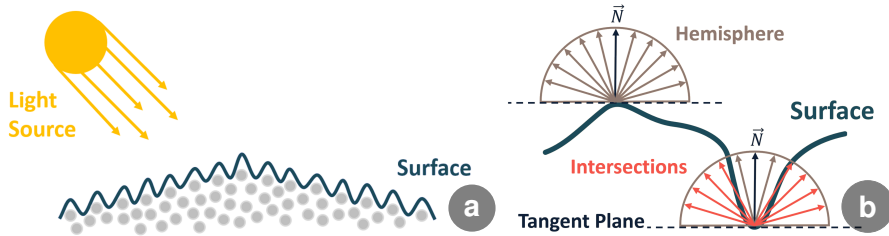
Figure 3.5: Juxtaposition of (a) an imaginary viewpoint from "the side" where a surface based on the density of underlying points is illuminated by a global light, and (b) an illustration showing how ambient occlusion can be determined using intersections of the local hemisphere.
