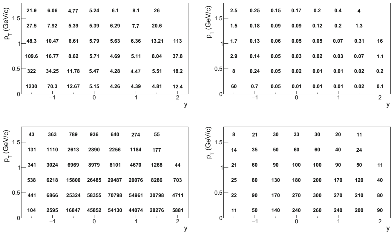
Fig. 6 Top : Monte-Carlo correction factors (see Eq. 2) in each (y, p_T) bin ( left ) and corresponding statistical uncertainties ( right ). Bottom : uncorrected bin-by-bin multiplicities of K_S^0 ( left ) and statistical uncertainties ( right )
