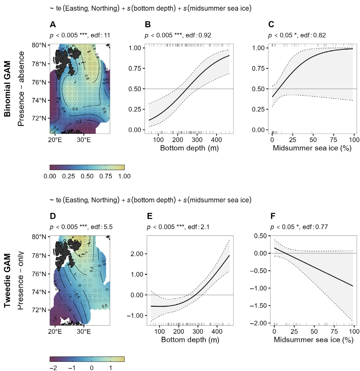
Fig. 5. Partial effects of key environmental factors on the probability of species presence (top row, A–C ) and biomass conditional on presence (bottom row, D–F ) of the remaining unidentified copepods in the large size fraction from the western Barents Sea, after Paraeuchaeta spp. and Calanus hyperboreus had been removed. Line plots show the shape of the response for one environmental variable independent of the other variables, with solid lines and shaded areas indicating the mean and 95% confidence intervals. The distribution of samples is given by the rugs on the x-axis. Confidence intervals are calculated to include the uncertainty about the overall mean. Contour plots show interactions with darker colors indicating lower and lighter colors higher values. Only significant terms included in the most parsimonious model, as indicated on top of each row, are shown. Note, that the y-axis in the plots for the binomial GAM (top row) shows the probability of occurrence, while for the Tweedie GAM (bottom row) values on the y-axis represent the deviation from the mean predicted biomass on the scale of the predictor, that is, a change of 0.5 on the log link scale used here would suggest a 65% increase in biomass.
