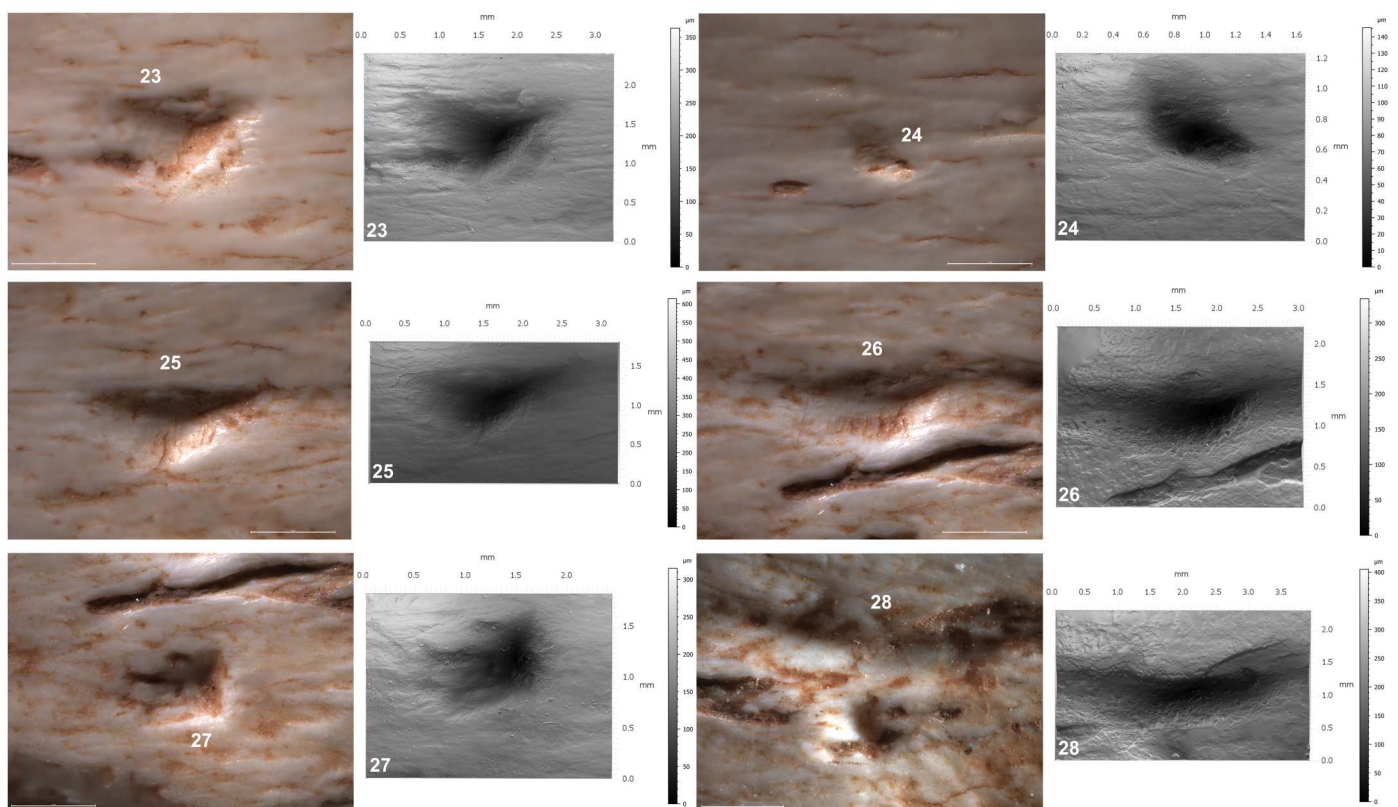
Fig. 6. Punctures 23 to 28 on the Canyars leather punch board. Comparison of the punctures 23 to 28 on the Canyars specimen by confocal (grayscale) and multifocus (colored) microscopy. Puncture ID are depicted in the top schematic drawing, and the different colors correspond to subsets of punctures made with the same tool (see Table 1). Scale bar (top), 1 cm.
