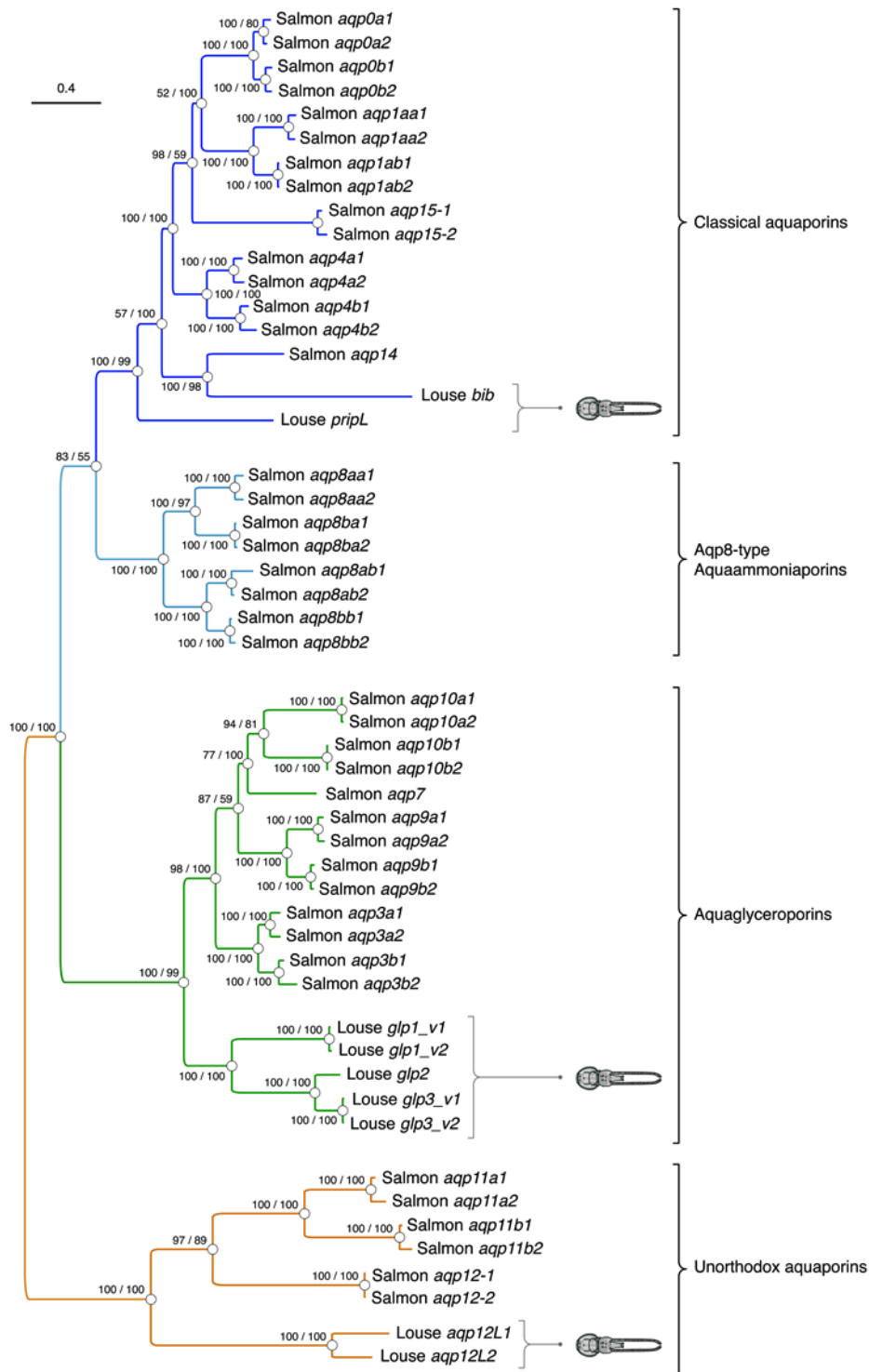
22 Figure S3. Bayesian majority-rule mid-point rooted tree of a codon alignment of the aquaporin 23 superfamilies in the Atlantic salmon and salmon louse. The tree was inferred from 1 million MCMC 24 generations on 57,075 nucleotide sites. Posterior probabilities of the codon/amino acid analyses are 25 shown at each node. Scale bar represents the number of nucleotide substitutions per site.
