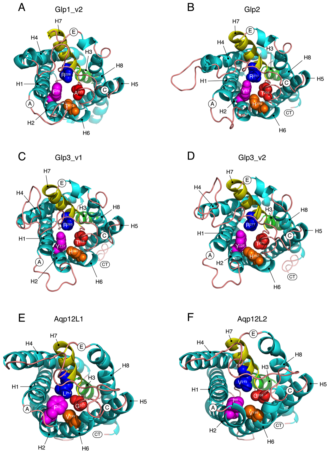
13 Figure S1. Extracellular views of cartoon renders of salmon louse aquaporins illustrating the ar/R 14 constriction residues (spacefill) that determine the molecular selectivity of the channel. Labels are 15 annotated as for Figure 1 in the main text.
