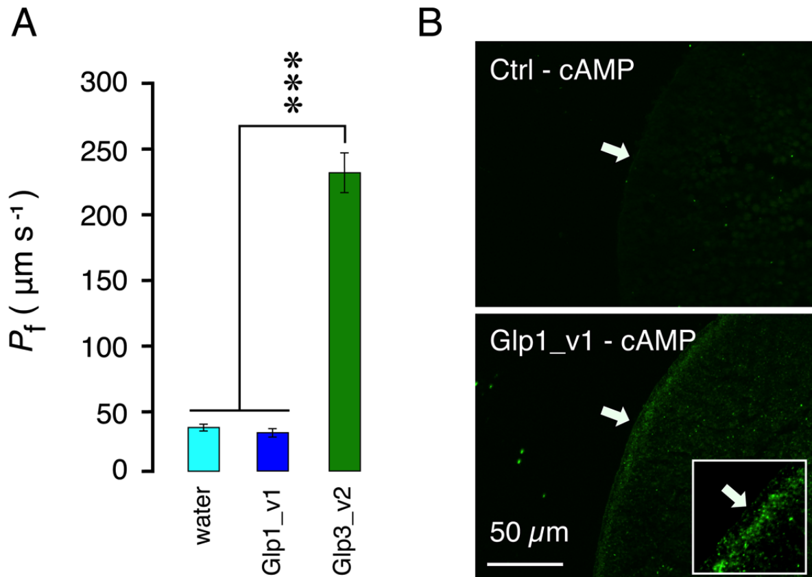
27 Figure S4. In the absence of cAMP, salmon louse Glp1_v1 is non functional in X. laevis oocytes. (A) 28 Osmotic water permeability ( P_f ) of Glp1_v1 without the addition of cAMP compared to water- and 29 glp_3v2 -injected oocytes as negative and positive controls, respectively. (B) Immunofluorescence 30 micrographs of paraffin sections of water- (Ctrl) and glp1_v1 -injected oocytes in the absence of cAMP 31 probed with paralog-specific antisera followed by Cy3-labeled anti-rabbit IgG. Arrows point to the 32 plasma membrane. Inset: Magnified region shows the retention of Glp1_v1 (green) just below the 33 oocyte plasma membrane.
