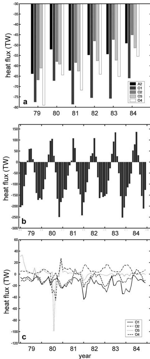
Figure 4. (a) Annual mean heat flux (TW) for different O-experiments, (b) monthly mean heat flux of the reference run A2, and (c) monthly mean oceanic heat flux differences: O-experiments minus reference run A2 ( O_x - A2 ). Negative heat flux in Figures 4a and 4b equals ocean heat loss to the atmosphere; positive heat flux equals ocean heat gain from the atmosphere.
