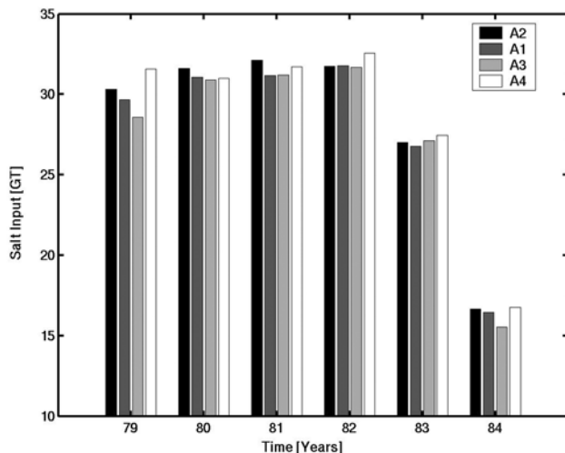
Figure 10. Annual mean salt input (GT) for different A-experiments.
