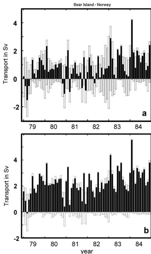
Figure 2. Time series of transport rates in Sv (Sverdrup = 10^6 \text{ m}^3/\text{s} ) through the Barents Sea opening (white columns) for (a) the reference experiment A2 and (b) the increased throughflow experiment O1. The net throughflow in both experiments is shown in black.
