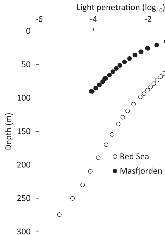
Fig. 2. Light penetration (given as the fraction of the irradiance just below surface) for the wavelength band 470–500 nm in the clear Red Sea compared with that of the murkier Masfjorden at the days of acoustic registrations; the Red Sea 15 November 2014 and Masfjorden 16 August 2011.
