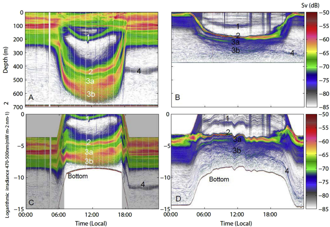
Fig. 3. Depth distribution of the acoustic scattering layers in the Red Sea on 15 November 2014 (A) and in Masfjorden on 16 August 2011 (B). The lower panels are based on the same observations, but instead of depth show the calculated ambient irradiance ( \log_{10} ) of the acoustic scatters for the Red Sea (C) and Masfjorden (D). The ambient irradiance ( \mu\text{mol quanta m}^{-2} \text{s}^{-1} ) was calculated from the surface broadband (Red Sea) and PAR (Masfjorden) and the corresponding K_{\text{PAR}} that were estimated from the underwater measurements at mid-day. We did not have observations of surface irradiance at night for the Red Sea and this period is indicated by grey shading in C.
