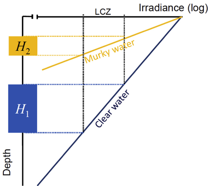
Fig. 1. Predictions from the LCZ hypothesis. If mesopelagic organisms distribute according to a light comfort zone (LCZ), the depth distribution of the organisms in a murky water column will be shallower and also narrower ( H_2 ) than that of a clear water column ( H_1 ). Both the depth location and the extension of the vertical distribution are proportional to the reciprocal light attenuation coefficient for downwelling irradiance which is given by the slope of the irradiance curve (log-scale). Modified from Dupont and Aksnes (2013).
