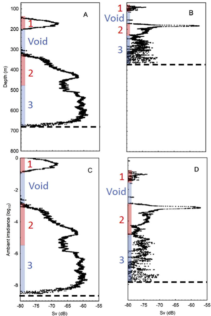
Fig. 4. Mid-day depth distribution of acoustic scatter in the Red Sea (A, 15 November 2014) and in Masfjorden (B, 16 August 2011). The lower panels are based on the same observations, but instead of depth show the total ambient irradiance (photons \text{m}^{-2} \text{s}^{-1} ), i.e. obtained by summing over the measured spectrum, of the acoustic scatters of the Red Sea (C) and Masfjorden (D). Broken lines indicate location of bottom. The numbers correspond to the layers that are also indicated in Fig. 3 and Table 1.
