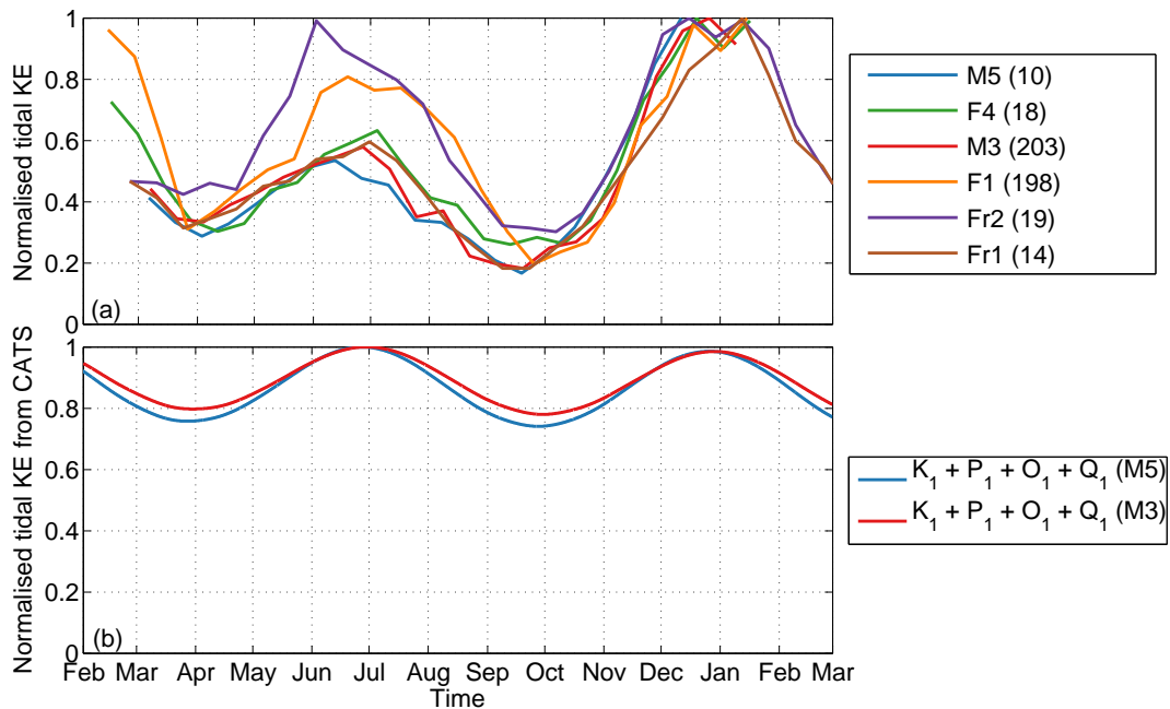
Figure 6. (a) Time series of normalised diurnal tidal KE at moorings M5 and F4 (deeper continental slope), M3 and F1 (shelf break) and the first year of record at Fr2 and Fr1 (shelf). At M5, KE is only calculated until the ADCP stops measuring (see Table 1). The maximum diurnal tidal KE values in \text{cm}^2 \text{s}^{-2} are given in parentheses in the legend. (b) Time series of normalised tidal KE at the K_1 + P_1 + O_1 + Q_1 tidal frequencies as predicted by the CATS tidal model at the locations and deployment times of moorings M3 and M5.
