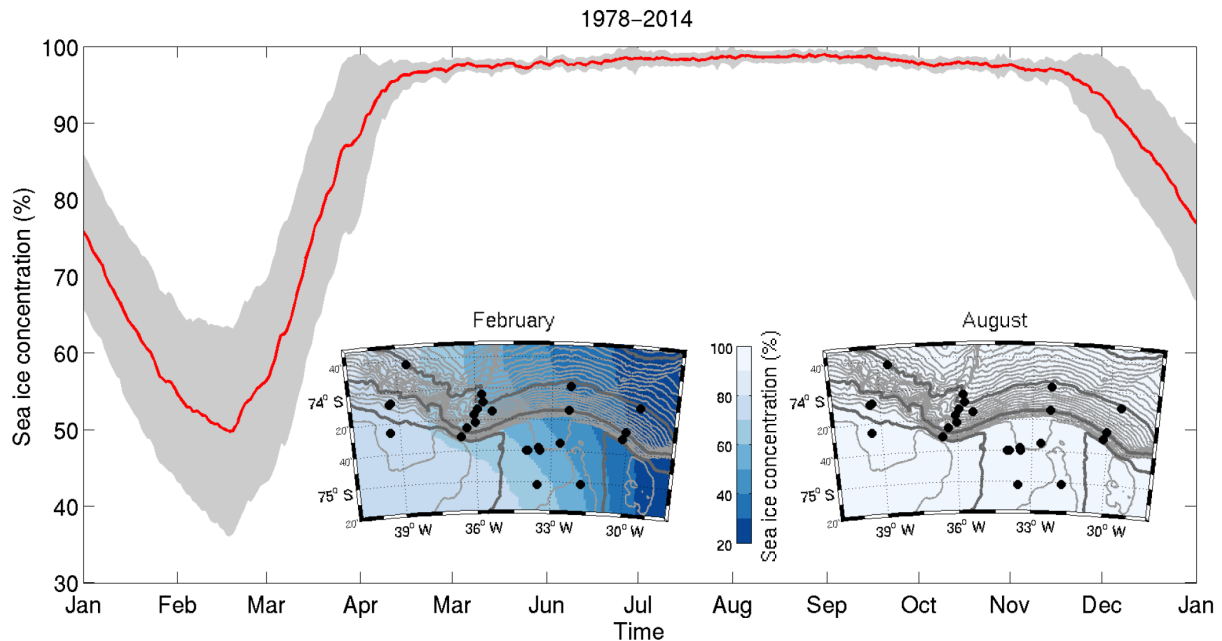
Figure 14. Sea ice concentration averaged over the study area and the period 1978–2014 (red line) with standard deviation (grey). Insets show maps of mean sea ice concentrations in February and August; isobaths and mooring locations (black dots) are as in Fig. 1.
