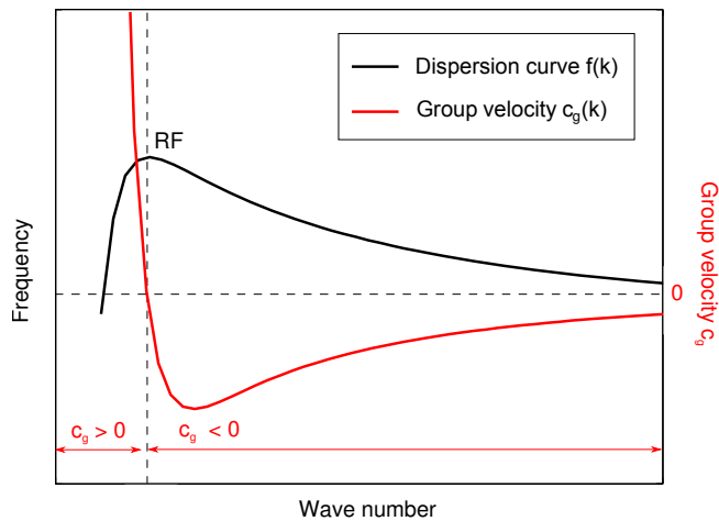
Figure 2. Illustration of a typical mode 1 CTW dispersion curve (black line) with the corresponding group velocity (red line). For small wave numbers, the group velocity is positive, while it becomes negative for larger wave numbers, i.e. indicating a change of direction of energy propagation. At the maximum of the dispersion curve (the resonant frequency, RF), the group velocity vanishes and energy is trapped.
