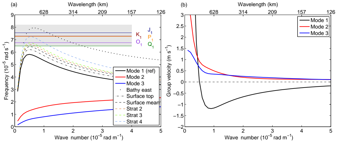
Figure 9. (a) Dispersion curves for CTWs of modes 1–3 using the reference stratification (thick lines). In addition, the dispersion curves for mode 1 CTWs for the bathymetry east of the study area (“bathy east”), differently inferred surface N^2 values for the reference stratification (“surface top”, using the uppermost value of the observational stratification profile, and “surface mean”, using the average of the upper 80 m of the observed stratification profile) and three other stratification profiles are shown. Stratification profiles 2–4 are representative of regions in the study area with increasing distance west of the reference stratification and inferred similarly. The diurnal tidal band is shaded in light grey with the most important diurnal frequencies marked by coloured lines. (b) Group velocities for CTWs of modes 1–3 using the reference stratification. Zero group velocity is indicated by a dashed line.
