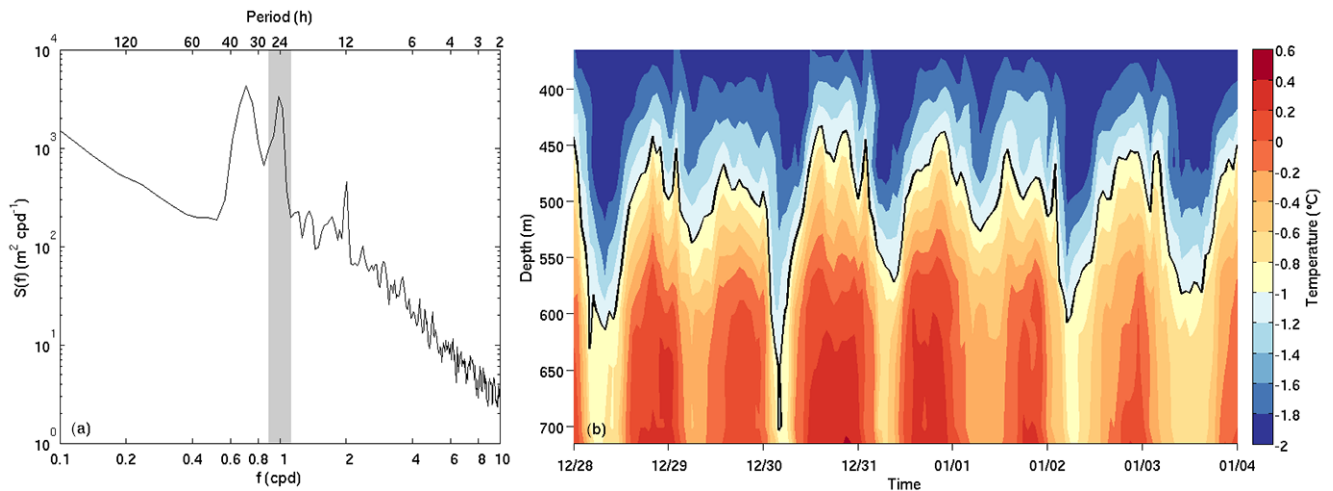
Figure 13. (a) Power spectral density of the height above the bottom of the -1^{\circ}\text{C} isotherm, which indicates the transition between WW and WDW at M3. The diurnal tidal frequency band is marked in grey. (b) Hovmöller diagram of low-pass filtered temperature at mooring M3 from 28 December to 4 January. The -1^{\circ}\text{C} isotherm is shown by a black line.
