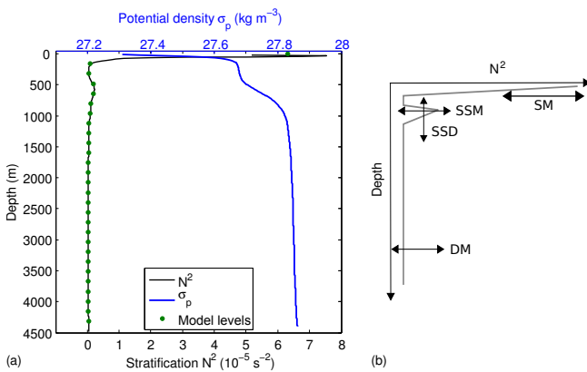
Figure 8. (a) Profiles of potential density (blue line) and resulting stratification (“reference stratification”, black line) from historic CTD data obtained in January and February in the area of moorings M1 to M5, merged with profiles from the deeper Weddell Sea at depth. Green markers indicate the vertical levels of the numerical code. (b) Sketch showing the parameters changed in the stratification sensitivity tests. Arrows indicate direction (but not magnitude) of changes. SM: surface magnitude, SSM: subsurface magnitude, SSD: subsurface depth, DM: deep magnitude.
