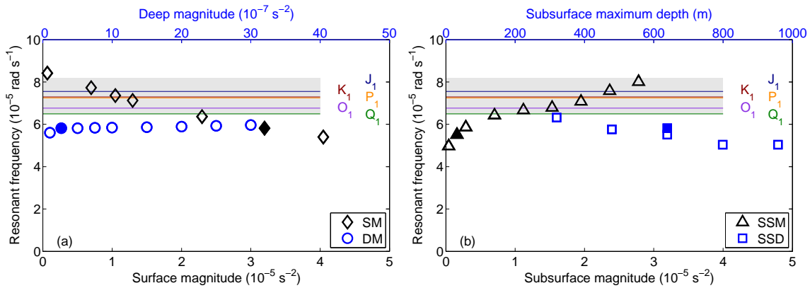
Figure 10. Sensitivity test for changing stratification. (a) The surface magnitude (SM) and deep magnitude (DM) are varied. (b) The subsurface magnitude (SSM) and its depth (SSD) are varied. Results from the reference stratification profile are indicated by filled markers. For the case of SSD, the shape of SSM in the profile is simplified (open marker below filled marker) and then varied in depth. The diurnal tidal band is shaded in light grey with the most important diurnal frequencies marked by coloured lines.
