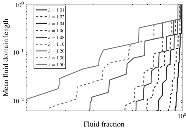
FIGURE 7. This log–log plot summarizes the relationship between remaining fluid fraction and characteristic fluid domain size. The linear trends (in log–log space) confirm the fractal structure of the solution over the full range of freezing rates.
