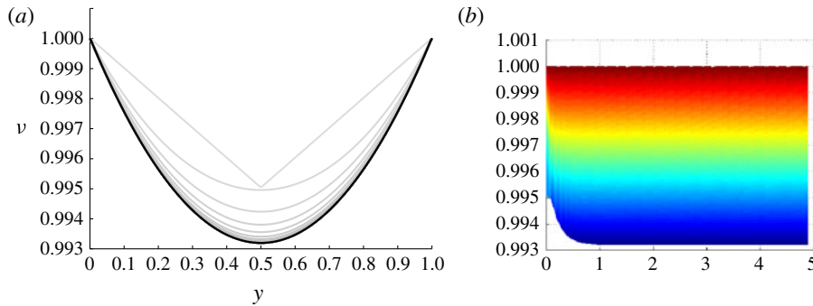
FIGURE 5. (Colour online) (a) The function \nu at various times (darker colour corresponding to later time); (b) the solution surface plotted against dimensionless time.
