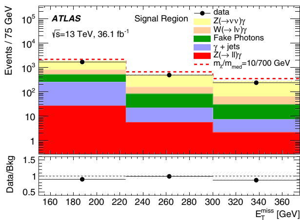
Fig. 3 Distribution of E_T^{\text{miss}} (left) and of E_T^\gamma (right) in the signal regions for data and for the expected total background; the total background expectation is normalised using the scale factors k' derived from the multiple-bin fit. Overflows are included in the third bin. The error bars are statistical, and the dashed band includes statistical and systematic
