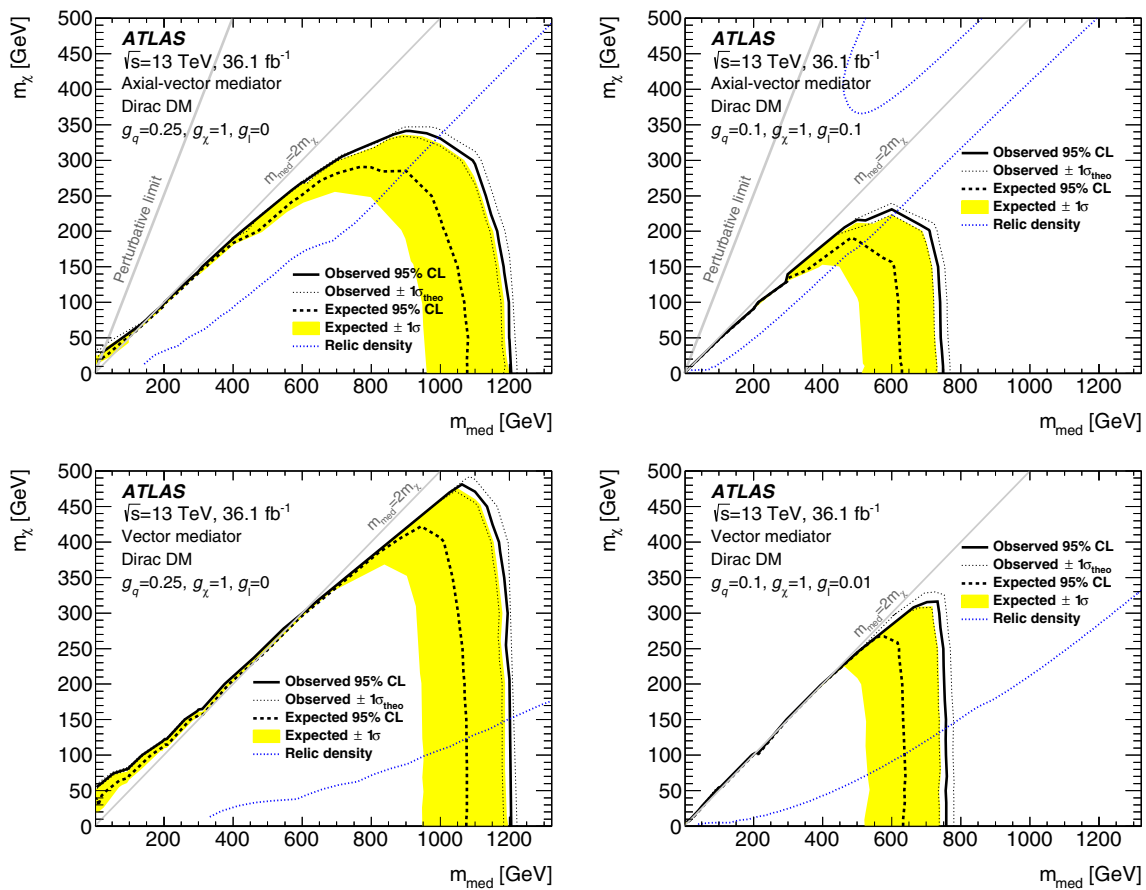
Fig. 4 The observed and expected 95% CL exclusion contours for a simplified model of dark-matter production involving an axial-vector operator, Dirac DM and couplings g_q = 0.25, g_\chi = 1 and g_\ell = 0 as a function of the dark-matter mass m_\chi and the mediator mass m_{\text{med}} (upper left). The plane under the limit curve is excluded. The same is shown for an axial-vector operator with couplings g_q = 0.1, g_\chi = 1 and g_\ell = 0.1 (top right), for a vector operator with couplings g_q = 0.25, g_\chi = 1 and g_\ell = 0 (bottom left) and for a vector operator with couplings
