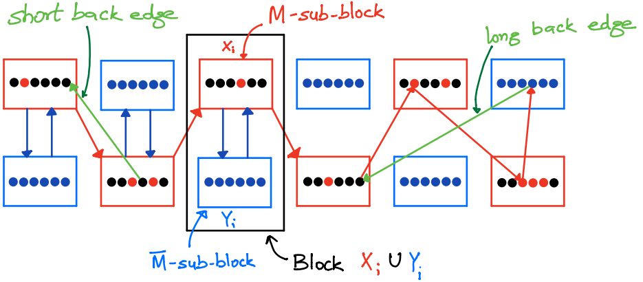
Figure 6.3: M -sequence of T
