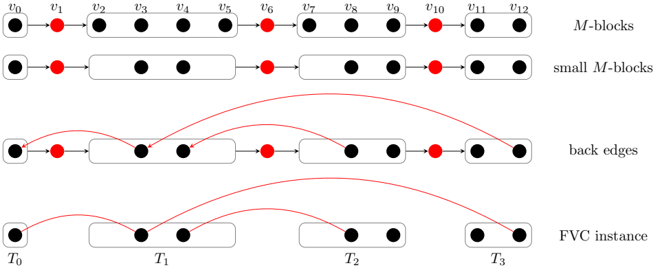
Figure 5.2: From TFVS to FVC
