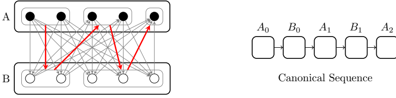
Figure 6.1: Canonical sequence of an acyclic bipartite tournament
