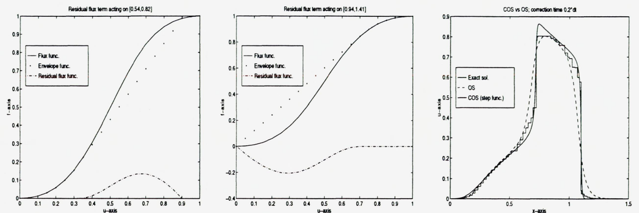
Figure 4.3. Example 2 (non-monotone data). The computations are done with 64 grid cells, 20 linear interpolation points, and 1 time step. Left and Middle: Residual flux function. Right: COS with correction time 0.08. Also in this non-monotone case (with several anti-diffusive flux terms) we see that COS resolves the shock front notably better than OS. Note that there is a loss of amplitude due to a large time step (see the text for a partial discussion).
