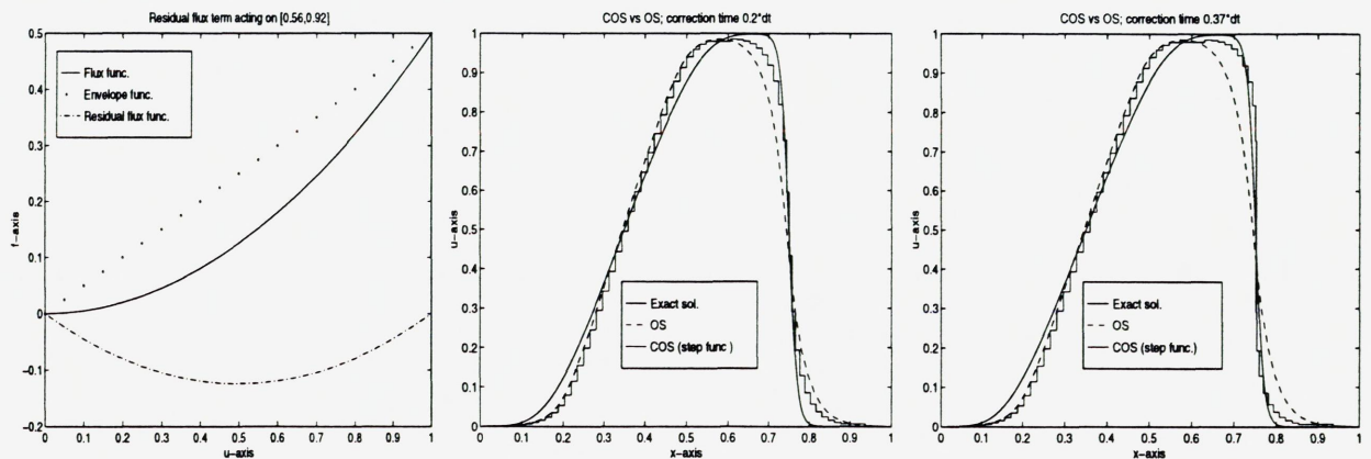
Figure 4.1. Example 1. The computations are done with 64 grid cells, 20 linear interpolation points, and 1 time step. Left: Residual flux function. Middle: COS with correction time 0.06. Right: COS with correction time 0.111. For a proper choice of the correction time we clearly see (right) that the error introduced by the heat equation is corrected so that (almost) the right size of the shock layer is obtained.
