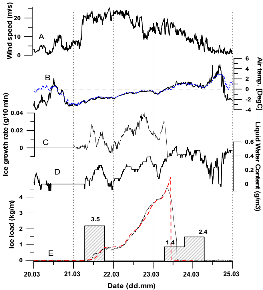
Figure 7. A) Wind speed calculated at 723 m a.s.l. B) Air temperature estimated (solid line) and measured (dotted line) at 723 m a.s.l. C) Ice growth rate (g/m 10 min) 3 hrs running mean at the ice scale. D) Estimated liquid water content at 723 m a.s.l. E) Ice load measured (solid line) and estimated (dotted line) (kg/m) at the ice scale. Lower step plot shows 12 hrs accumulated precipitation, where the numbers above indicate the amount of precipitation in
