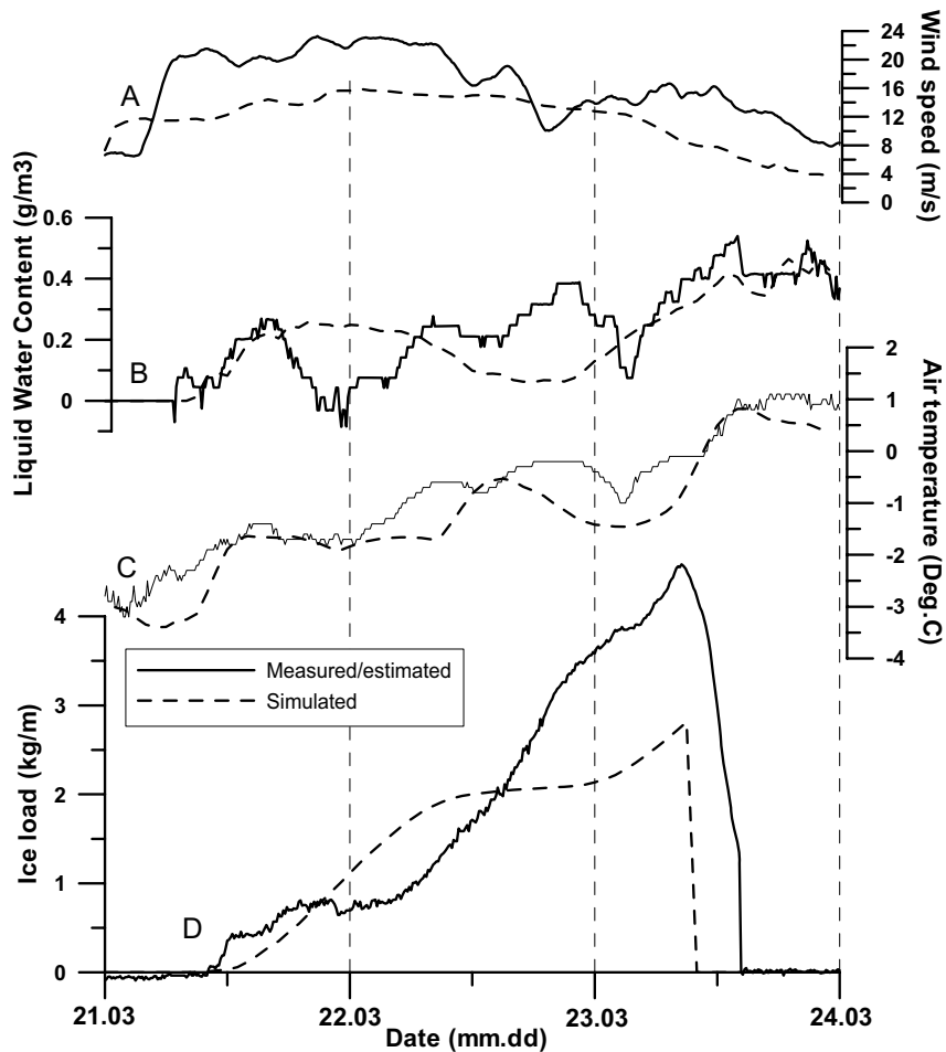
Figure 8. A) Wind speed and B) LWC estimated from measurements (solid line) at 723 m a.s.l. and simulated by MM5 (dotted line) at 554 m a.s.l., respectively. C) Air temperature at 723 m a.s.l. measured (solid line) and simulated (dotted line). D) Ice load measured by the ice scale (solid line) and simulated by MM5 (dotted line).
