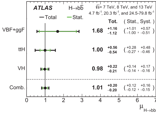
Fig. 7. The fitted values of the Higgs boson signal strength \mu_{H \rightarrow b\bar{b}} for m_H = 125 GeV separately for the VH, t\bar{t}H and VBF+ggF analyses along with their combination, using the 7 TeV, 8 TeV and 13 TeV data. The individual \mu_{H \rightarrow b\bar{b}} values for the different production modes are obtained from a simultaneous fit with the signal strengths for each of the processes floating independently. The probability of compatibility of the individual signal strengths is 83%.
